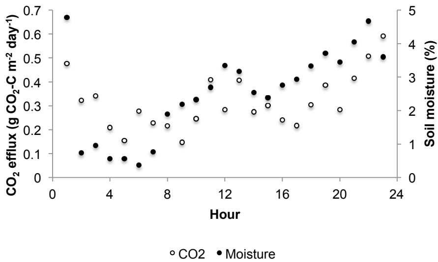
Supplementary Figure S2 | Mean CO 2 efflux rates and soil moisture contents in the field during the 24-hour study.
