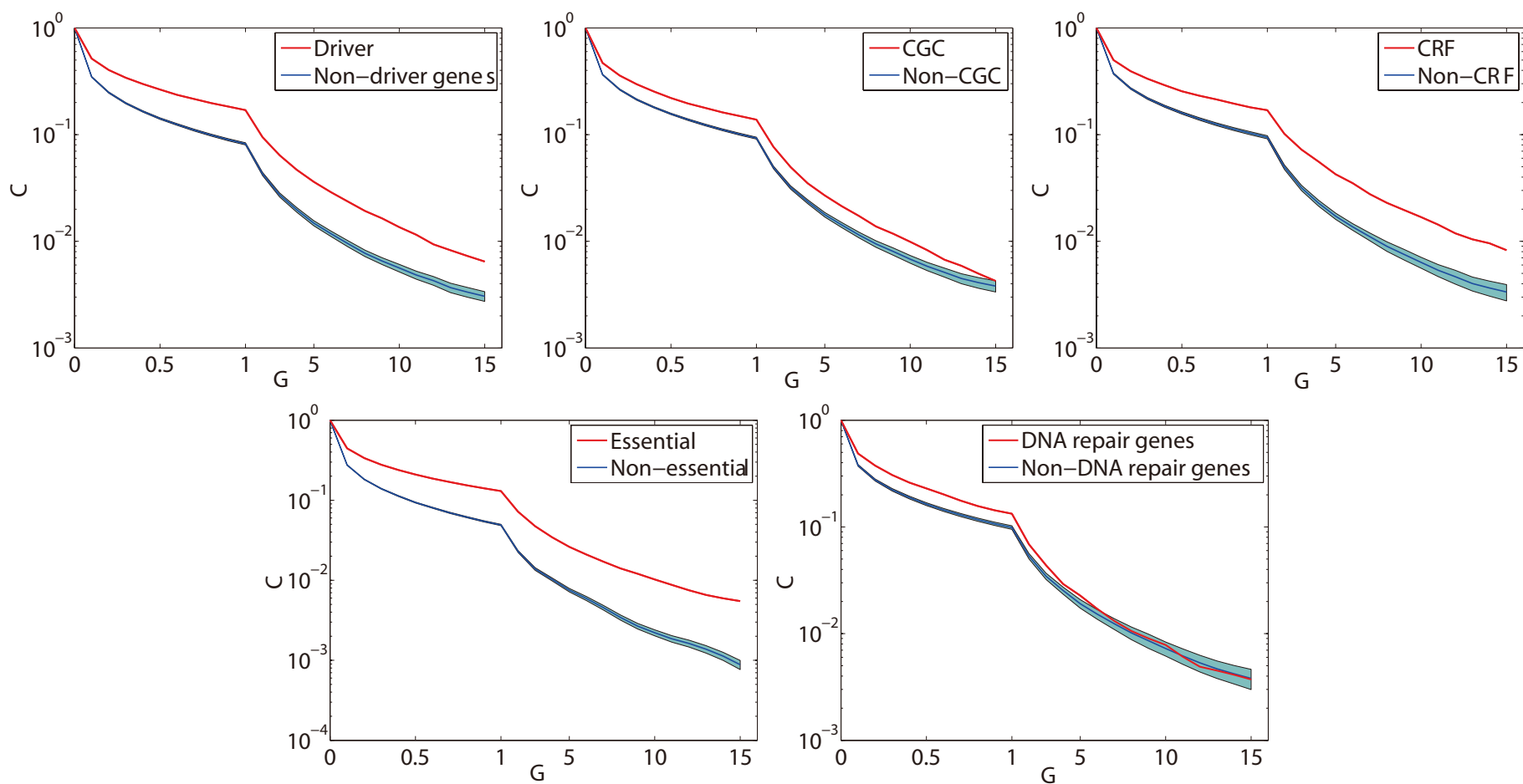
Fig. S2. The complementary cumulative distribution ( C ) of the gene-gene gravitation score ( G ) for five different gene sets: cancer driver gene (Driver), Cancer Gene Census (CGC), chromatin regulation factors (CRF), essential genes, and DNA repair genes in breast invasive carcinoma (BRCA). The number of gene-gene pairs for blue line is equal to red line by random sampling 100 times. The shadow of blue line represent the standard deviation.
