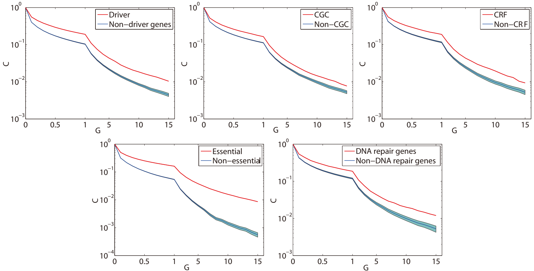
Fig. S3. The complementary cumulative distribution ( C ) of the gene-gene gravitation score ( G ) for five different gene sets: cancer driver gene (Driver), Cancer Gene Census (CGC), chromatin regulation factors (CRF), essential genes, and DNA repair genes in colon adenocarcinoma (COAD). The number of gene-gene pairs for blue line is equal to red line by random sampling 100 times. The shadow of blue line represent the standard deviation.
