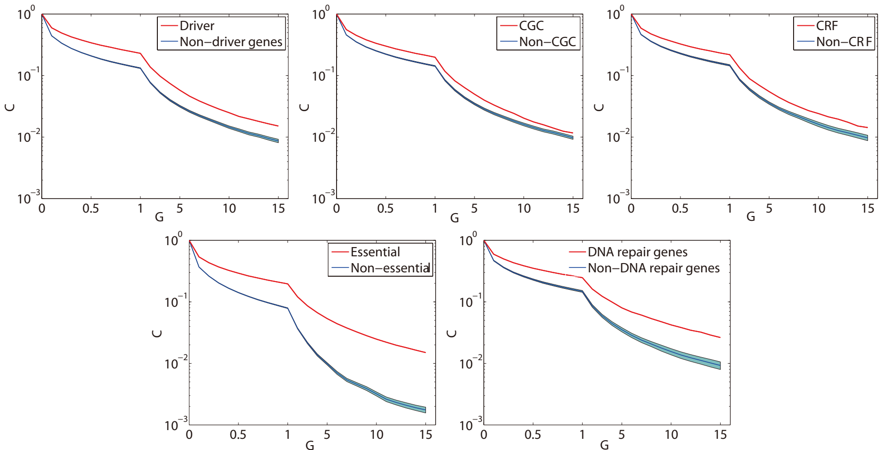
Fig. S4. The complementary cumulative distribution ( C ) of the gene-gene gravitation score ( G ) for five different gene sets: cancer driver gene (Driver), Cancer Gene Census (CGC), chromatin regulation factors (CRF), essential genes, and DNA repair genes in glioblastoma multiforme (GBM). The number of gene-gene pairs for blue line is equal to red line by random sampling 100 times. The shadow of blue line represent the standard deviation.
