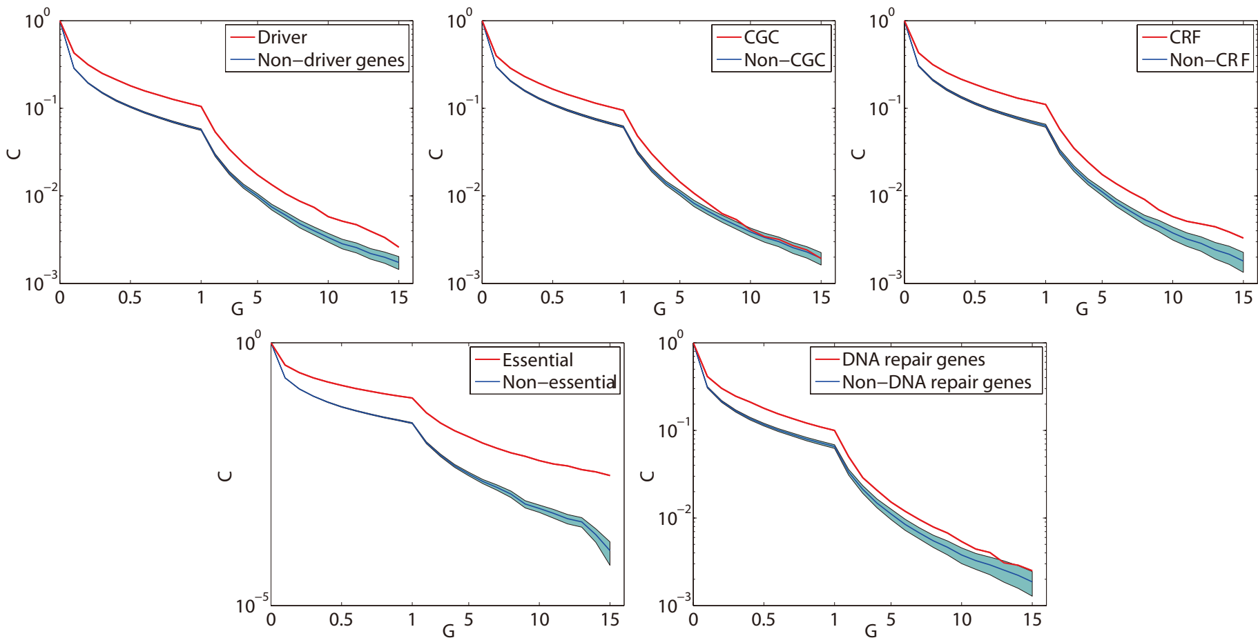
Fig. S9. The complementary cumulative distribution (C) of the gene-gene gravitation (G) score for five different gene sets: cancer driver gene (Driver), Cancer Gene Census (CGC), chromatin regulation factors (CRF), essential genes, and DNA repair genes in ovarian serous cystadenocarcinoma (OV). The number of gene-gene pairs for blue line is equal to red line by random sampling 100 times. The shadow of blue line represent the standard deviation.
