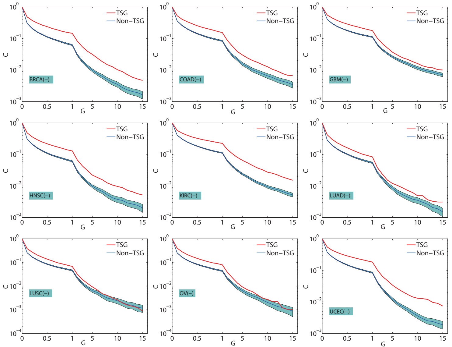
Fig. S14. The complementary cumulative distribution (C) of the repulsive gene-gene gravitation score (G) for tumor suppressor genes (TSG) across 9 major cancer types: breast invasive carcinoma (BRCA), colon adenocarcinoma (COAD), glioblastoma multiforme (GBM), head and neck squamous cell carcinoma (HNSC), kidney renal clear cell carcinoma (KIRC), lung adenocarcinoma (LUAD), lung squamous cell carcinoma (LUSC), ovarian serous cystadenocarcinoma (OV), and uterine corpus endometrial carcinoma (UCEC). The number of repulsive gene-gene pairs for blue line is equal to red line by random sampling 100 times. The shadow of blue line represent the standard deviation.
