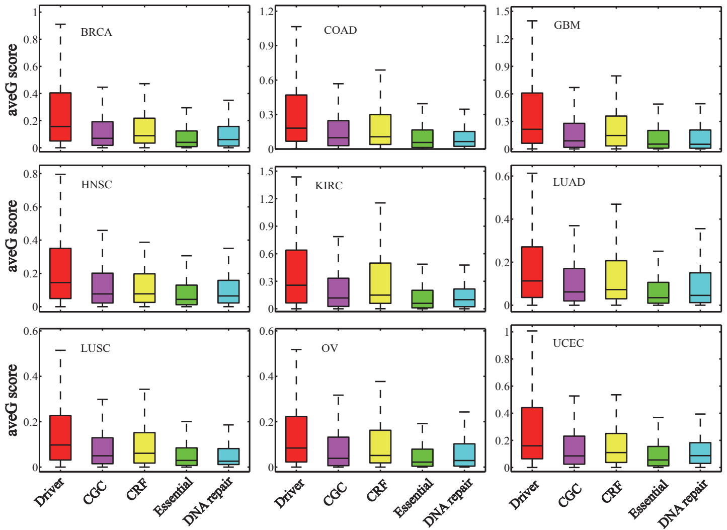
Fig. S27. Box plots of gene average gravitation (aveG) score for five gene sets across 9 cancer types when set up \alpha = 0.2 during mutation network propagation. Red: Cancer driver genes (Driver); purple: Cancer Gene Census (CGC) genes; yellow: Chromatin regulation factors (CRF); green: Essential genes (Essential); and blue: DNA repair genes.
