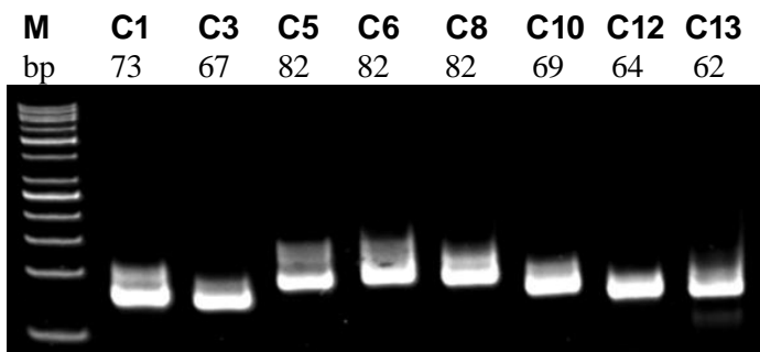
S1 Fig. PAGE analysis of Klenow fill-in products. 15 pmol of each randomized double stranded fragment were applied on a 10% PAGE for evaluation of the integrity of the elongation products; M=50 bp ladder (Invitrogen).
