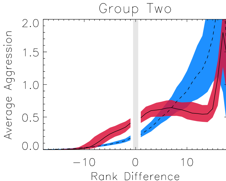
S2 Fig. Stationary features of Group Two with NBB included. Stationary features of Group Two are largely unchanged by the inclusion of NBB, except for the peak at the largest rank differences corresponding to aggression directed against the lowest ranking individual, NBB, by high-ranking individuals who repel NBB's unwanted attempts at affiliation. Multi-modal observations allow us to attribute these effects entirely to NBB's anomalous attempts to affiliate with high-ranking individuals who continually repelled these unwanted attempts. Exclusion of this single individual completely eliminates this peak, as can be seen in Fig. ?? in the Main Text. Inclusion of NBB also leads to an apparent delay in the onset of structured aggression in Group Two.
