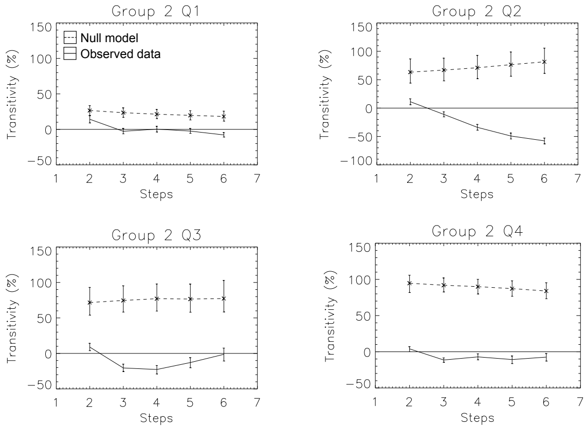
S10 Fig. T(n) broken out quarter-by-quarter for Group Two.
