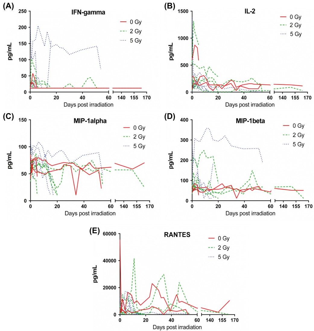
Supplementary Figure 1. Effects of 2 and 5 Gy TBI on plasma: (A) IFN- \gamma , (B) IL-2, (C) MIP-1 \alpha , (D) MIP-1 \beta , and (E) RANTES. Single data points from individuals plotted across time.
