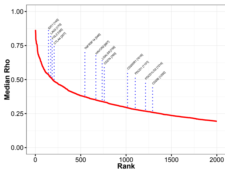
CLEC2B
