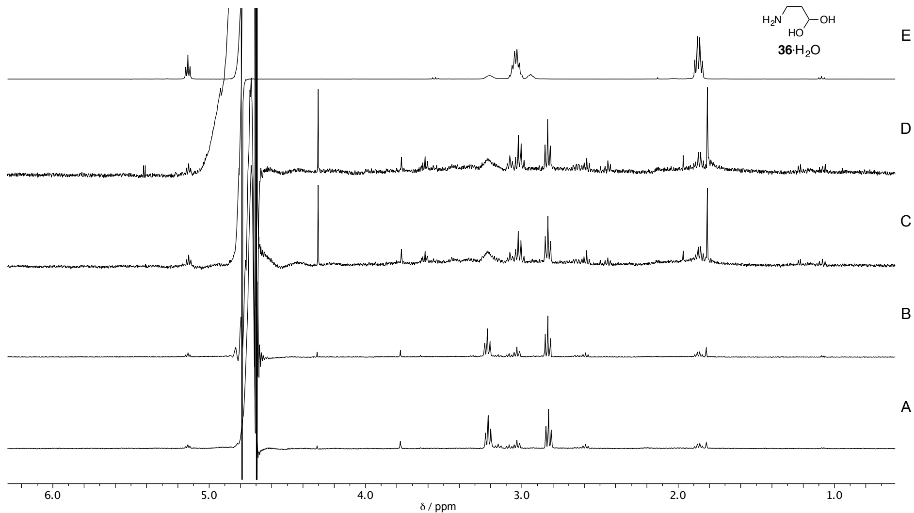
Figure S18. 1 H-NMR analysis (H 2 O/D 2 O, 9:1) of the photochemical conversion of aminopropionitrile 34 to aminopropionaldehyde hydrate 36 ·H 2 O. A – reaction mixture after 4 h; B – reaction mixture after 6 h; C – reaction mixture after 16 h; D – reaction mixture after 22 h; E – synthetic standard of aminopropionaldehyde hydrate 36 ·H 2 O prepared as described in the next section.
