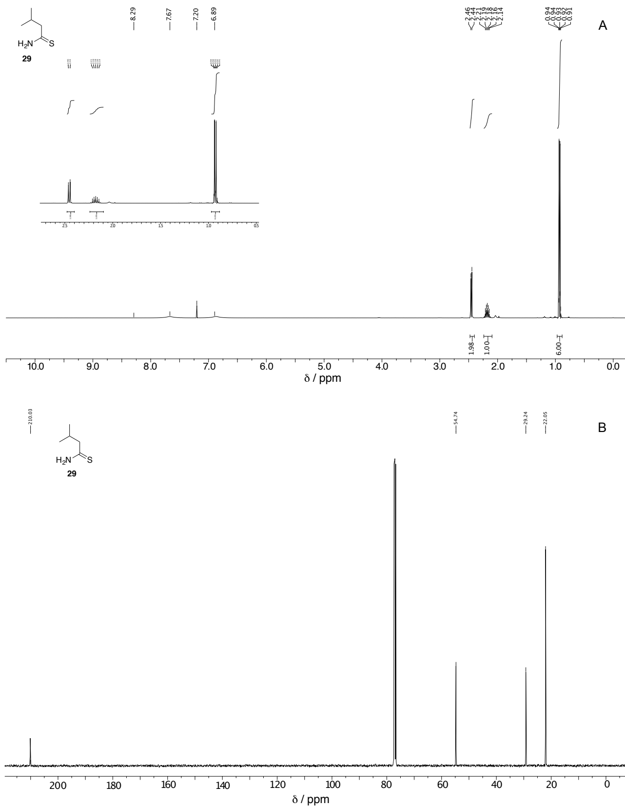
Figure S13. Analysis of the synthetic standard of thioamide 29 : A – ^1\text{H} -NMR (400 MHz, \text{CDCl}_3 ). Insert: expanded section between 0.5-3 ppm; B – ^{13}\text{C} -NMR (100 MHz, \text{CDCl}_3 ).
