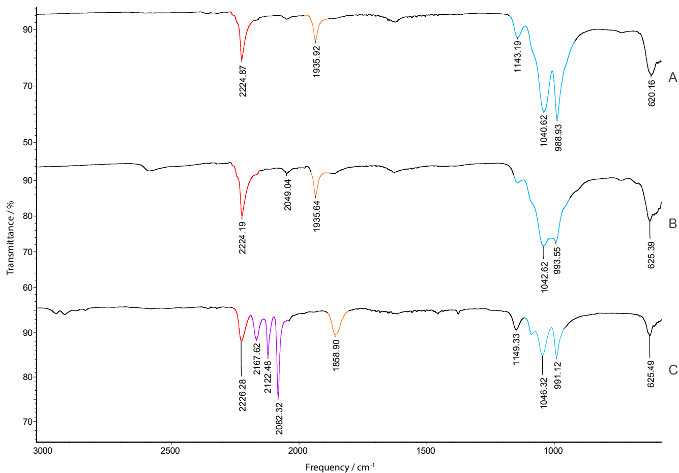
Figure S46. IR spectra from investigation of selective phosphate release from the \text{CuC}_3\text{N} –copper(I) phosphate mixture. A – starting \text{CuC}_3\text{N} –copper(I) phosphate mixture; B – residual precipitate without the addition of HCN, showing \text{CuC}_3\text{N} –copper(I) phosphate mixture signals (as in A); C – residual precipitate with the addition of HCN, suggesting reduction in amount of phosphate (blue signals), a similar signal for \text{C}\equiv\text{N} (red), a shift in the signal for \text{C}\equiv\text{C} (orange), and new signals in the \text{C}\equiv\text{N} region (purple) indicative of some \text{CuCN} and a possible [(\text{NC})_n\text{CuC}_3\text{N}]^{\text{p-}} type species prior to release of the cyanoacetylene 6 .
