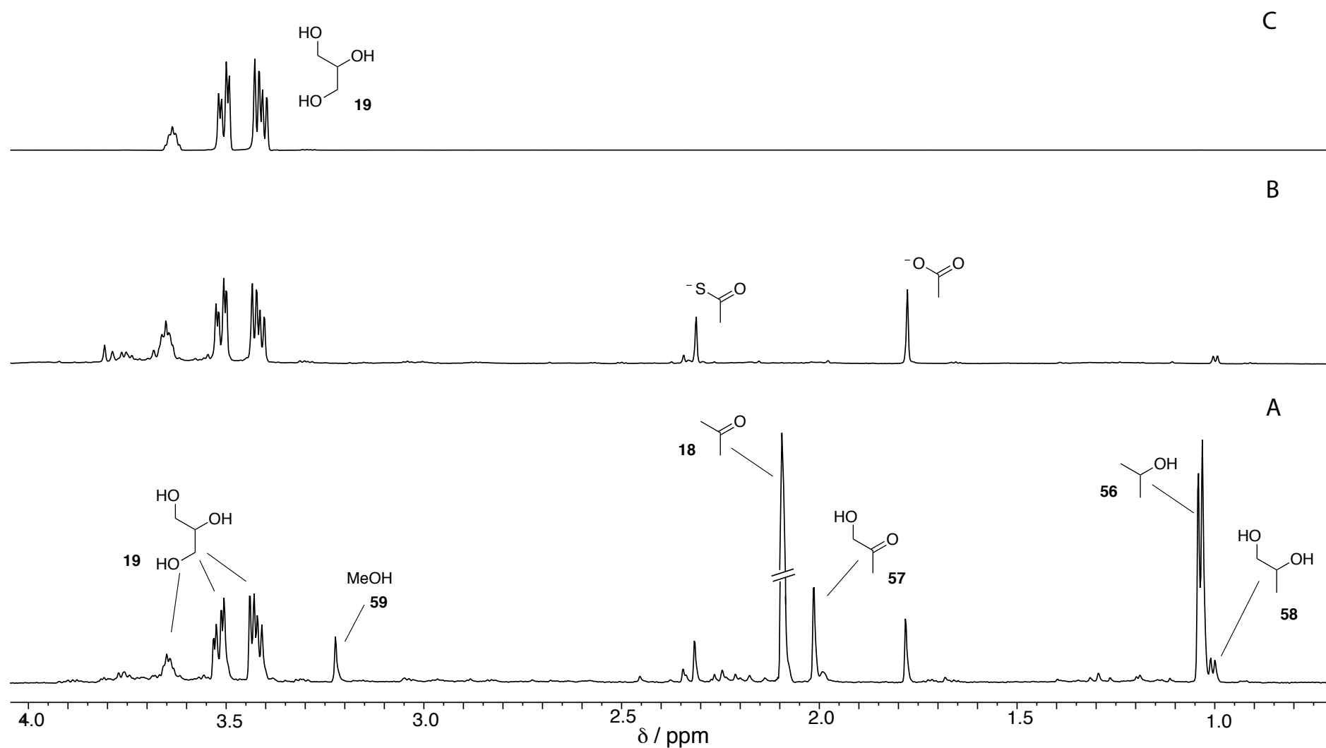
Figure S2. 1 H-NMR analysis (H 2 O/D 2 O, 9:1) of the conversion of dihydroxyacetone 17 into acetone 18 and glycerol 19 . A – spectrum of a sample from the photochemical reaction after 6 h; B – spectrum of the same sample after evaporation to dryness and redissolution in H 2 O/D 2 O (9:1, 1 mL); C – spectrum of a reference sample of glycerol.
