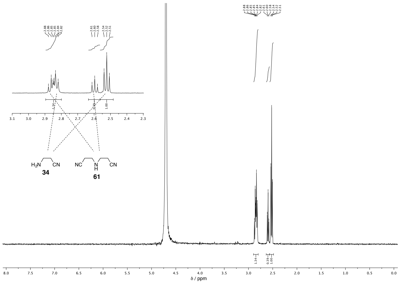
Figure S17. ^1\text{H-NMR} analysis (D 2 O) of the formation of aminopropionitrile 34 along with 3,3'-iminodipropionitrile 61 , from acrylonitrile 33 after 6 h.
