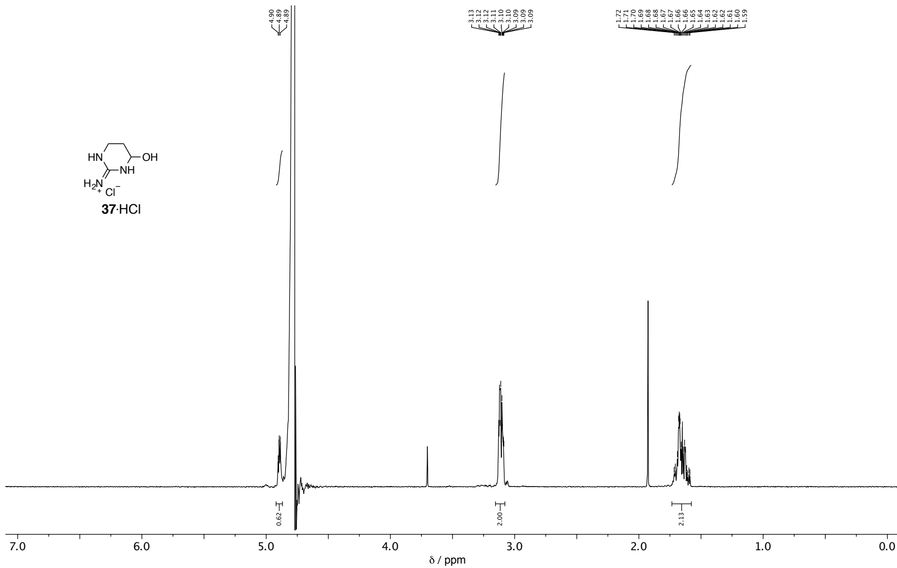
Figure S24. 1 H-NMR spectrum of 4-hydroxytetrahydropyrimidin-2(1H)-iminium hydrochloride 37 ·HCl.
