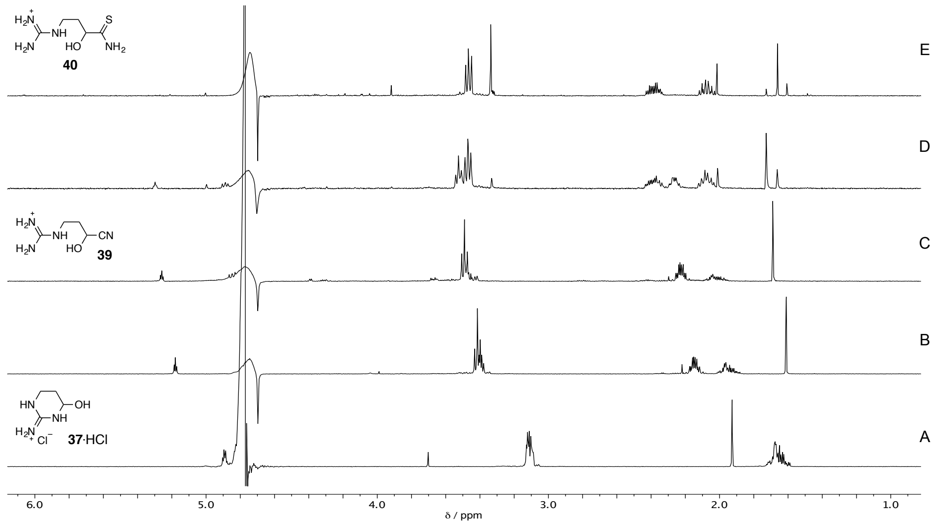
Figure S26. 1 H-NMR analysis (H 2 O/D 2 O, 9:1) of the conversion of 4-hydroxy-tetrahydropyrimidin-2(1H)-iminium hydrochloride 37·HCl to \alpha -hydroxythioamide 40 by the way of cyanohydrin 39 . A – synthetic standard of 4-hydroxy-tetrahydropyrimidin-2(1H)-iminium hydrochloride 37·HCl ; B – reaction with HCN at pH 7.1 after 20 h; C – reaction mixture with HCN at pH 7.1 after 6 d giving predominantly the corresponding cyanohydrin 39 ; D – reaction with NaSH at pH 8.2 after 22 h; E – reaction with NaSH at pH 8.2 after 4 d giving the corresponding \alpha -hydroxythioamide 40 .
