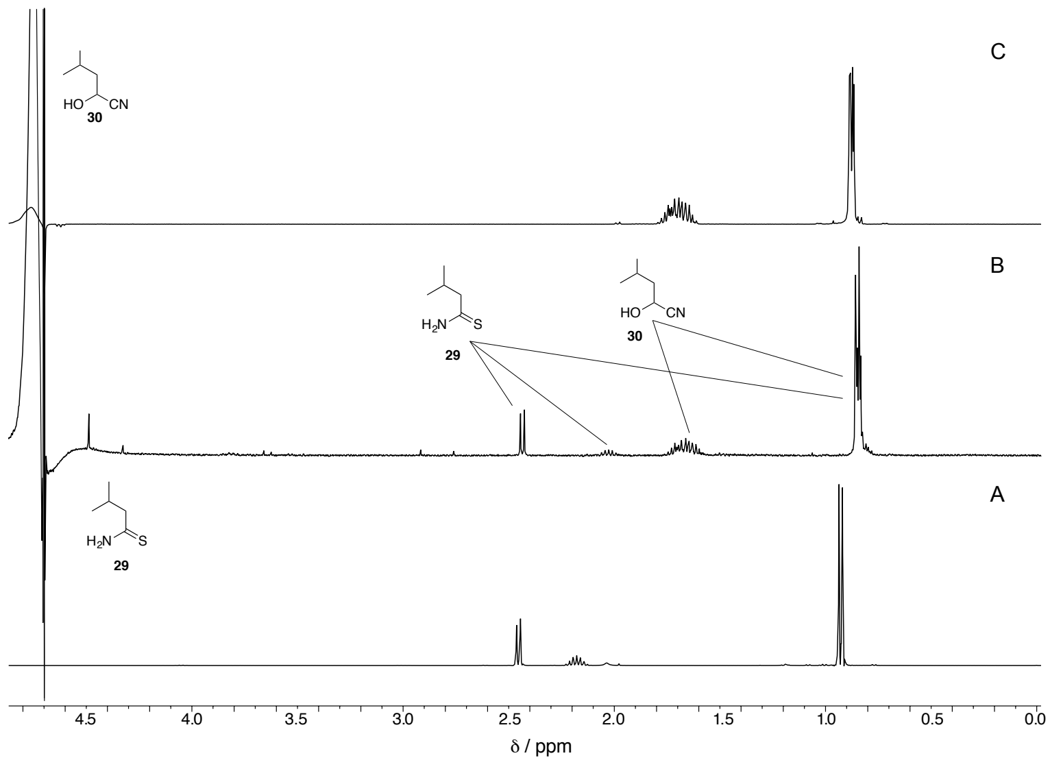
Figure S14. 1 H-NMR analysis of the conversion of thioamide 29 to cyanohydrin 30 . A (CDCl 3 ) –starting material, the pure synthetic standard of thioamide 29 ; B (H 2 O/D 2 O, 9:1) –reaction products after 1.5 h of irradiation; C (H 2 O/D 2 O, 9:1) – pure synthetic standard of cyanohydrin 30 .
