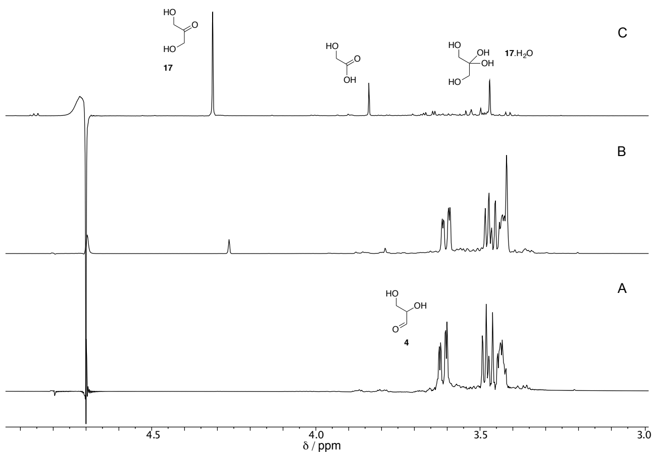
Figure S1. 1 H-NMR analysis (H 2 O/D 2 O, 9:1) of the conversion of glyceraldehyde 4 to dihydroxyacetone 17 by enolisation-ketonisation. A – glyceraldehyde at t = 0; B – reaction after 3 d showing the formation of glycolate and dihydroxyacetone (ketonic and hydrate form); C – reaction after 20 d showing the near complete conversion of glyceraldehyde to dihydroxyacetone (ketonic and hydrate form, 59 %), glycolate (14.1 %) and formate (12.7%). The formate peak at 8.3 ppm is not shown.
