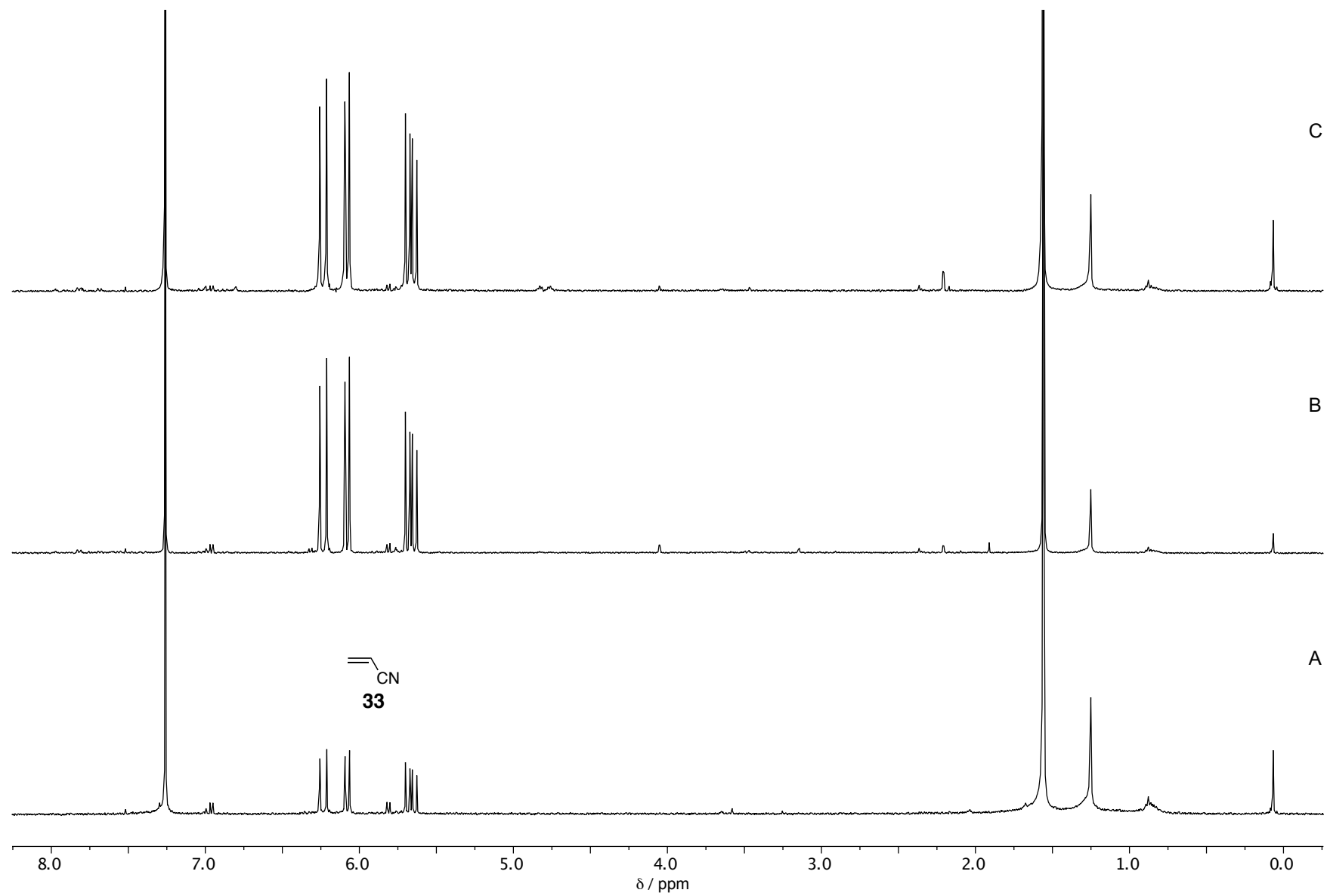
Figure S16. ^1\text{H-NMR} analysis ( \text{CDCl}_3 ) of the formation of acrylonitrile 33 . A – extract after 1 h; B – extract after 3 h; C – extract after 22 h.
