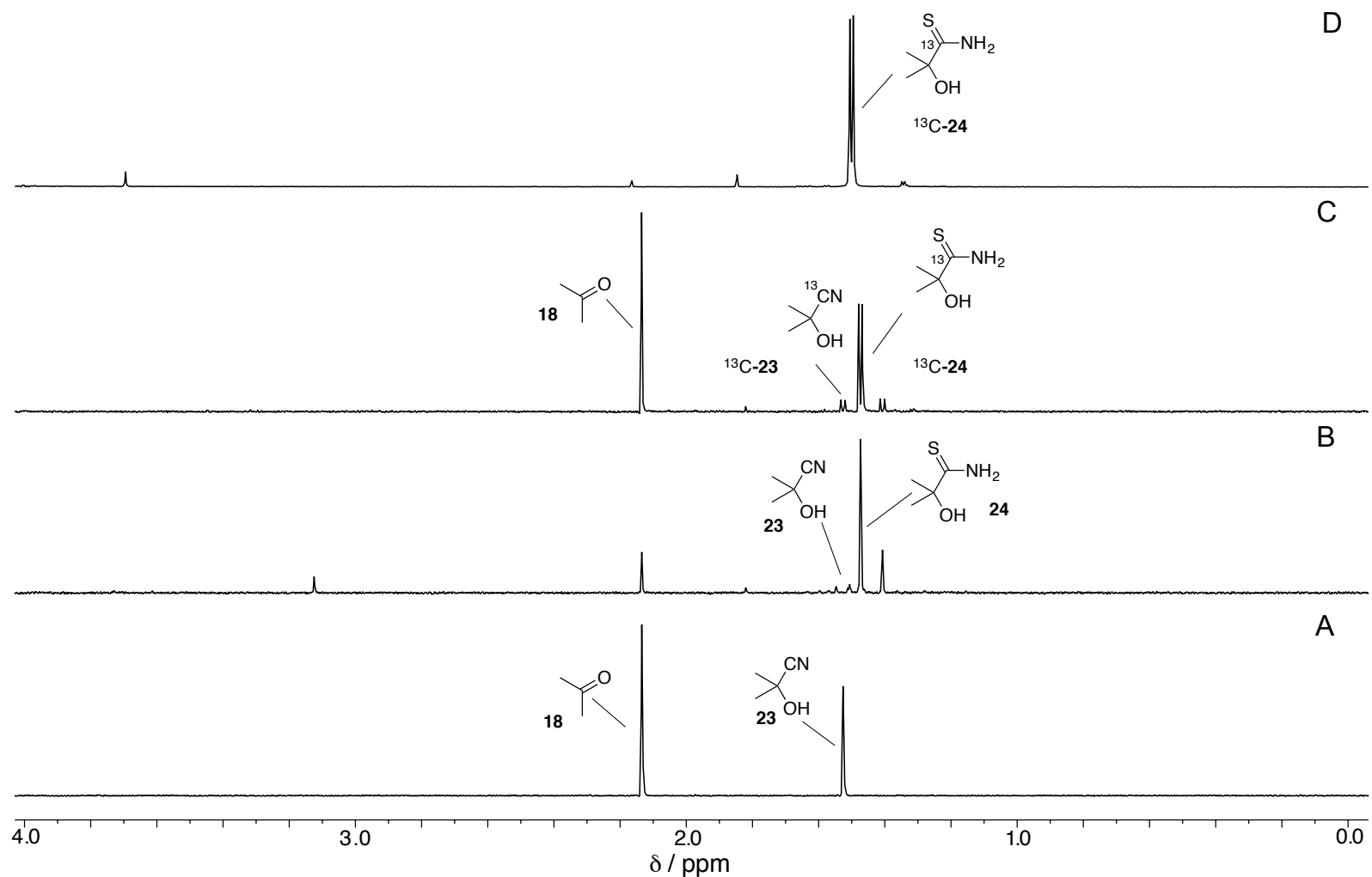
Figure S6. ^1\text{H} -NMR analysis ( \text{H}_2\text{O}/\text{D}_2\text{O} , 9:1) of the conversion of acetone 18 into cyanohydrin 23 and \alpha -hydroxythioamide 24 . A – spectrum of the reaction products 3 h after the addition of KCN; B – spectrum of the reaction products 48 h after the addition of NaSH; C – spectrum of the corresponding reaction using ^{13}\text{C} -labelled \text{K}^*\text{CN} for the cyanohydrin formation 24 h after the addition of NaSH; D – as C after removal of excess cyanide and acetone by sparging with \text{N}_2 followed by evaporation to dryness.
