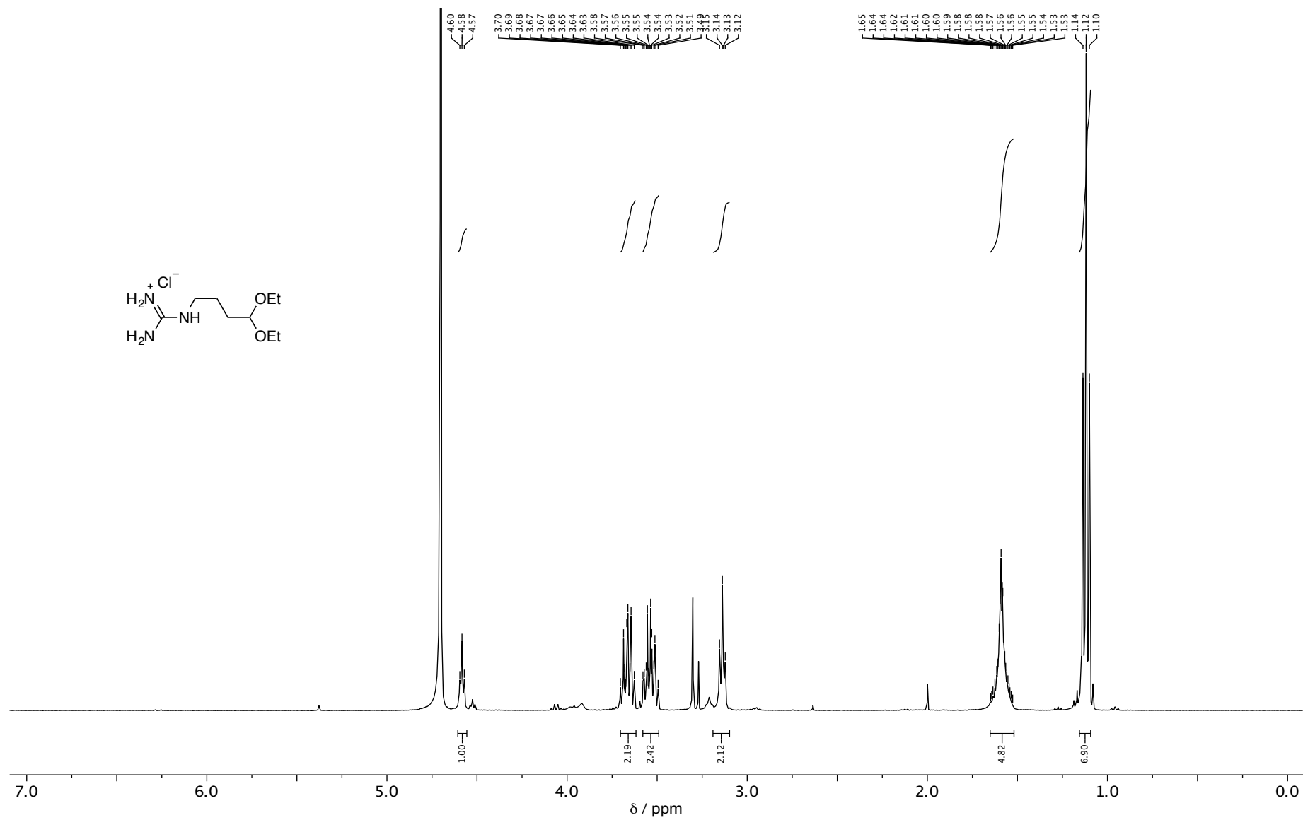
Figure S28. ^1\text{H} -NMR spectrum of amino((4,4-diethoxybutyl)amino)methaniminium hydrochloride.
