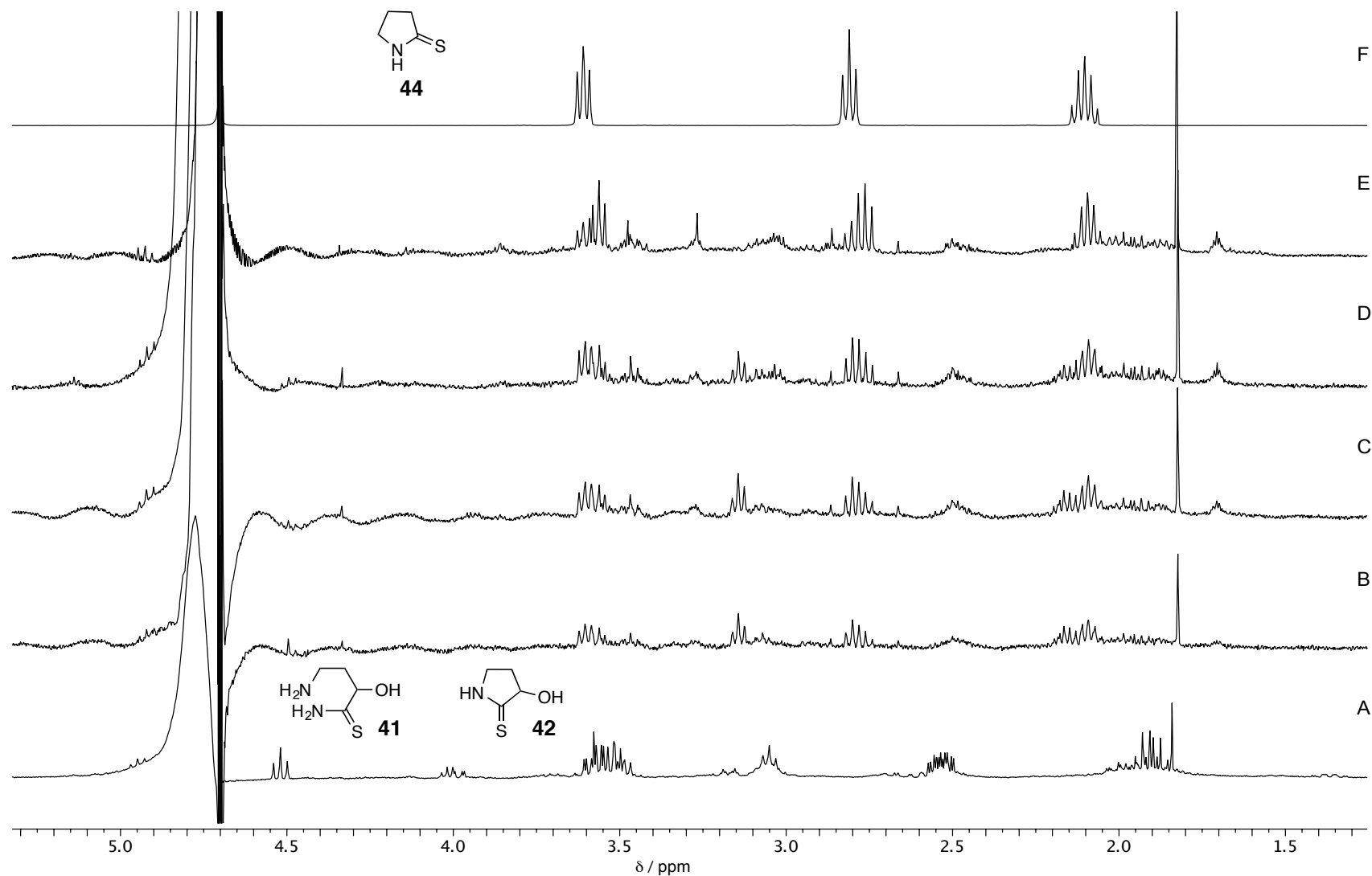
Figure S20. 1 H-NMR analysis (H 2 O/D 2 O, 9:1) of the photochemical conversion of α-hydroxythioamides 41 and 42 to the corresponding cyclic deoxygenated pyrrolidine-2-thione 44 . A – mixture of linear and cyclic α-hydroxythioamides 41 and 42 ; B – reaction mixture after 3 h; C – reaction mixture after 5 h; D – reaction mixture after 7 h; E – reaction mixture after 12 h; F – commercially available pyrrolidine-2-thione 44 .
