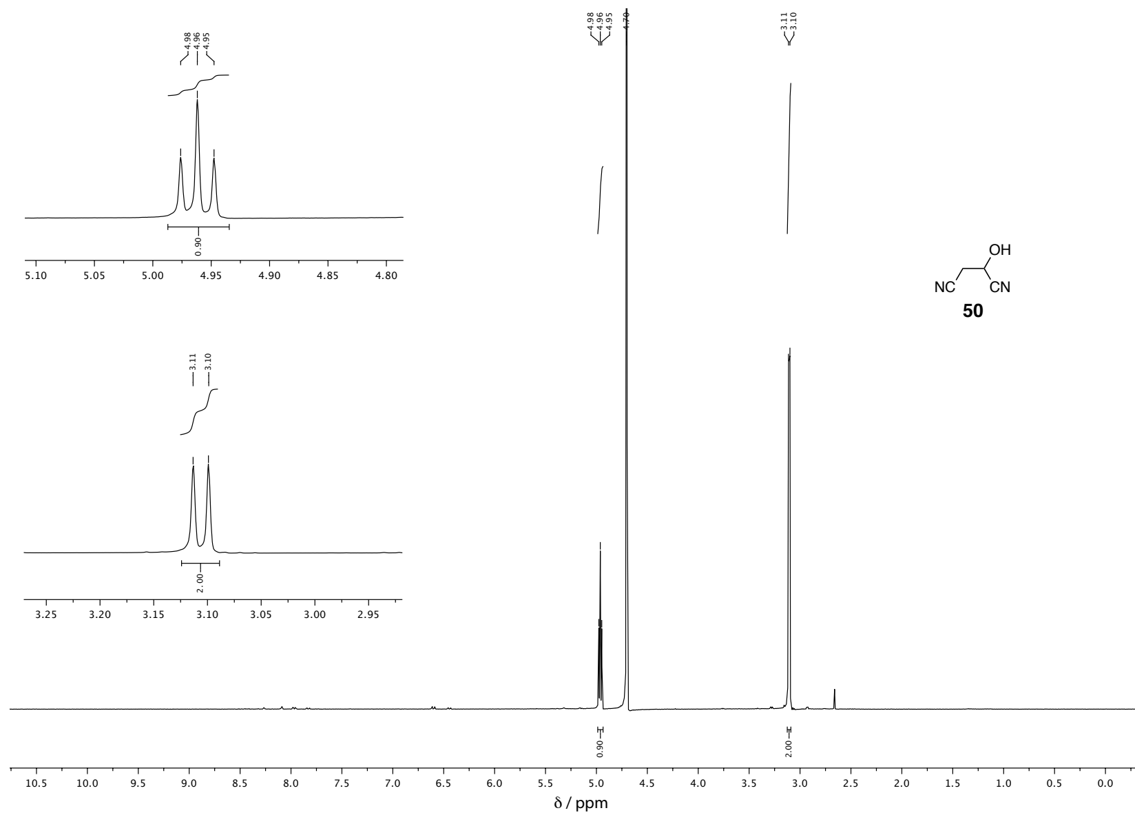
Figure S34. 1 H-NMR spectrum of the synthetic standard of Asn/Asp cyanohydrin 50 .
