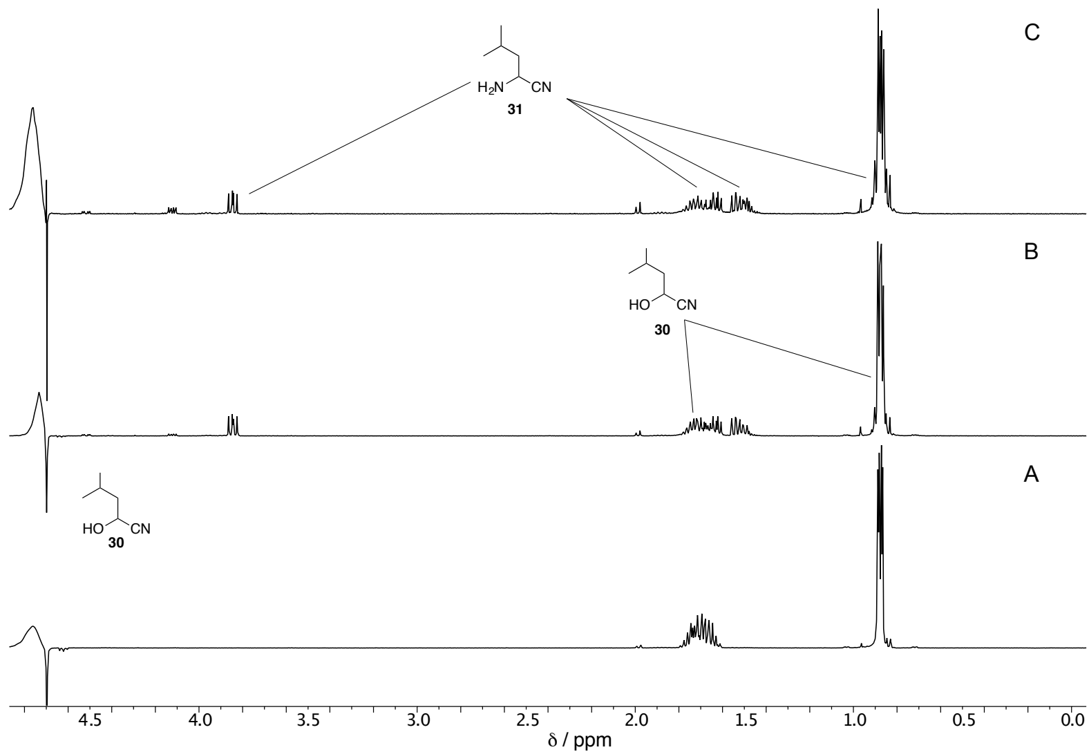
Figure S15. ^1\text{H-NMR} analysis ( \text{H}_2\text{O}/\text{D}_2\text{O} , 9:1) of the conversion of cyanohydrin 30 into \alpha -aminonitrile 31 . A – spectrum of the reaction mixture before addition of ammonia showing the pure cyanohydrin 30 ; B – spectrum of the reaction mixture 4 d after ammonia addition. C – spectrum of the reaction mixture 13 d after ammonia addition.
