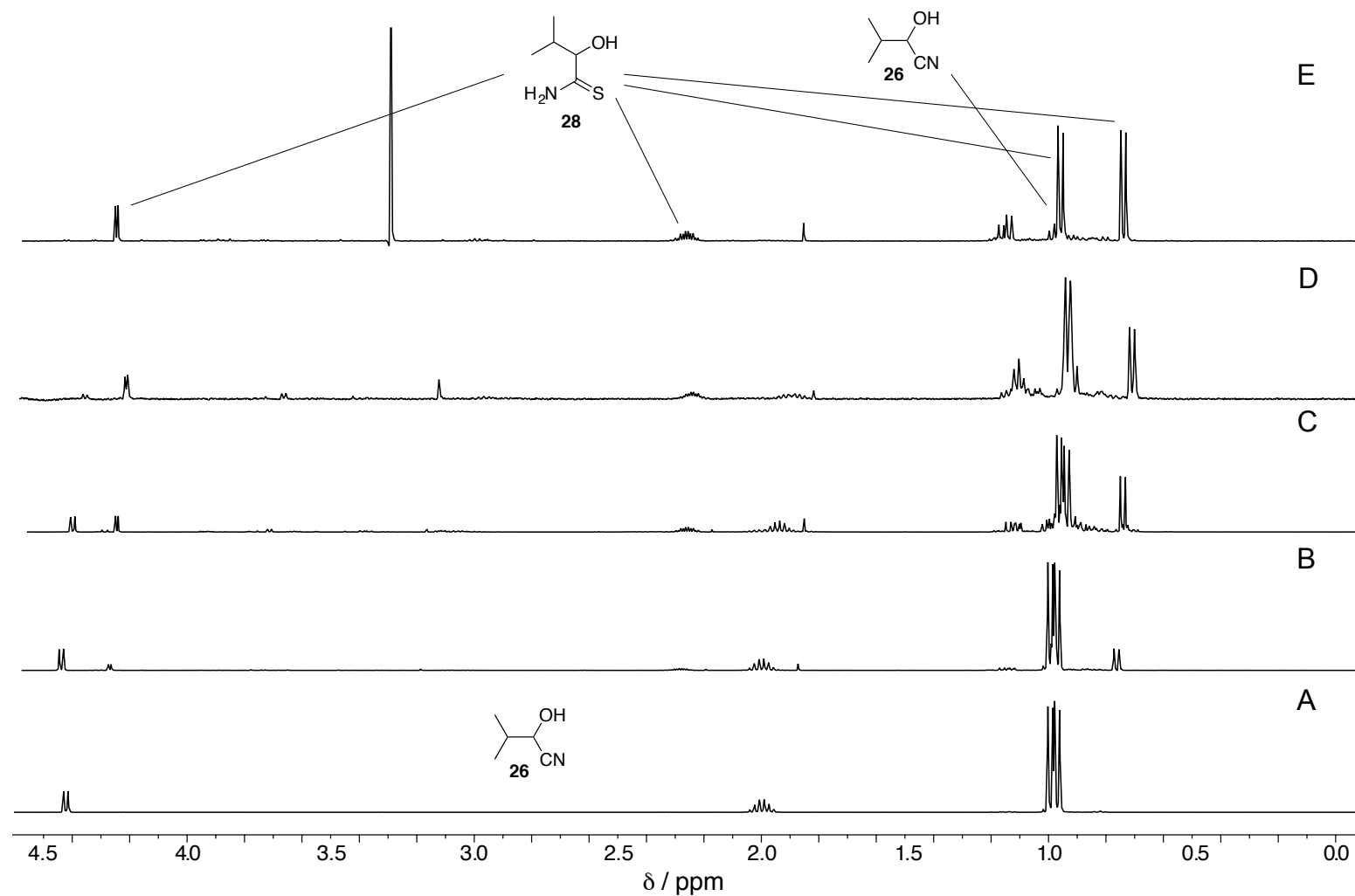
Figure S11. 1 H-NMR analysis (H 2 O/D 2 O, 9:1) of the conversion of cyanohydrin 26 into \alpha -hydroxythioamide 28 . A – spectrum of the reaction mixture before addition of NaSH showing the cyanohydrin 26 as the only product; B – spectrum of the reaction mixture 2 d after NaSH addition; C – as B after 3 d; D – as B after 7 d; E – as B after 9 d. The appearance of methanol after 9 d (signal at 3.25 ppm) is thought to be due to a contamination during sample handling.
