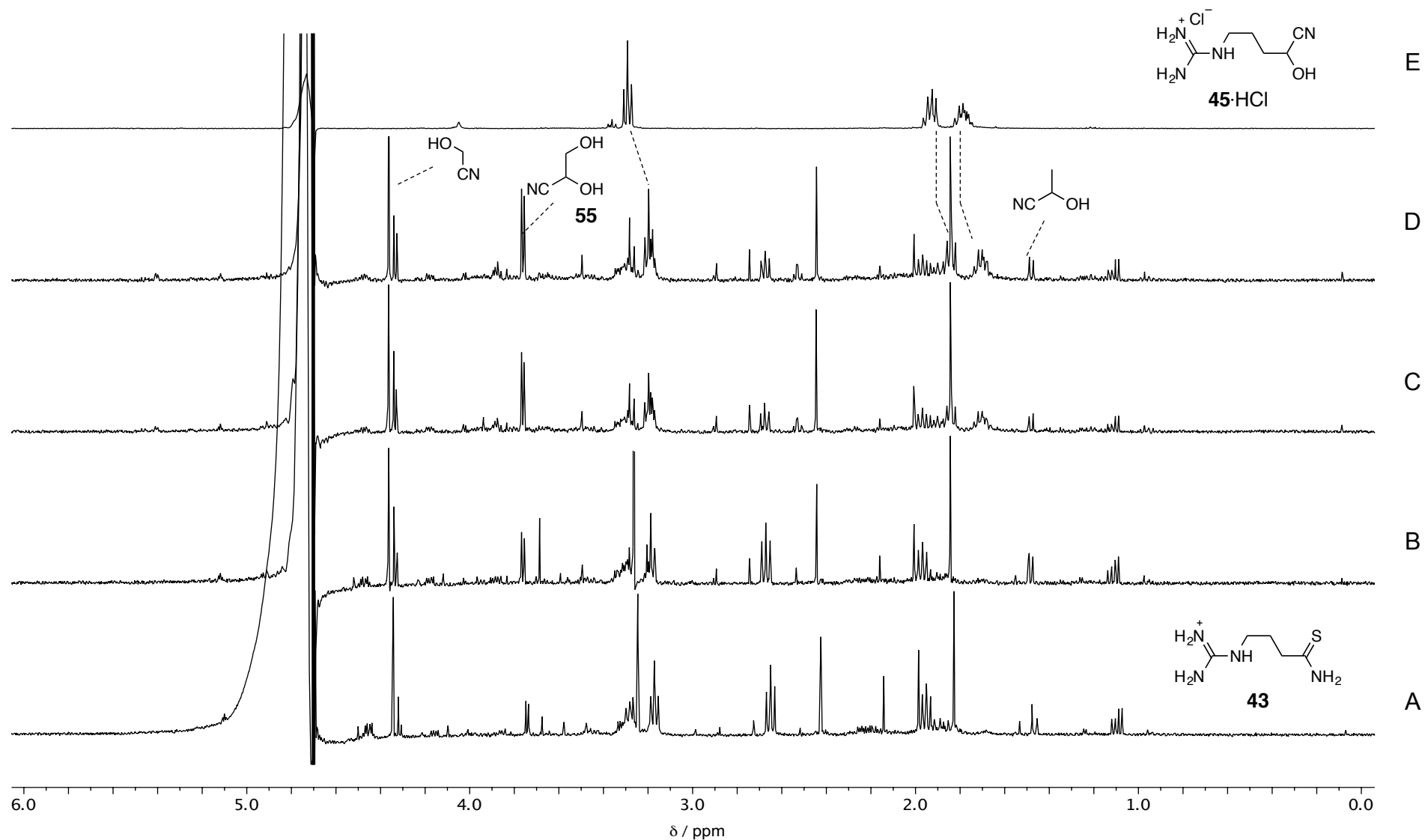
Figure S30. 1 H-NMR analysis (H 2 O/D 2 O, 9:1) of the photochemical conversion of thioamide 43 to cyanohydrin 45 . A – starting reaction mixture of thioamide 43 ; B – reaction mixture after 1.5 h; C – reaction mixture after 6 h; D – reaction mixture after 12 h, also showing the presence of Gly, Ser 55 , and Ala cyanohydrins; E – synthetic standard of cyanohydrin hydrochloride 45·HCl .
