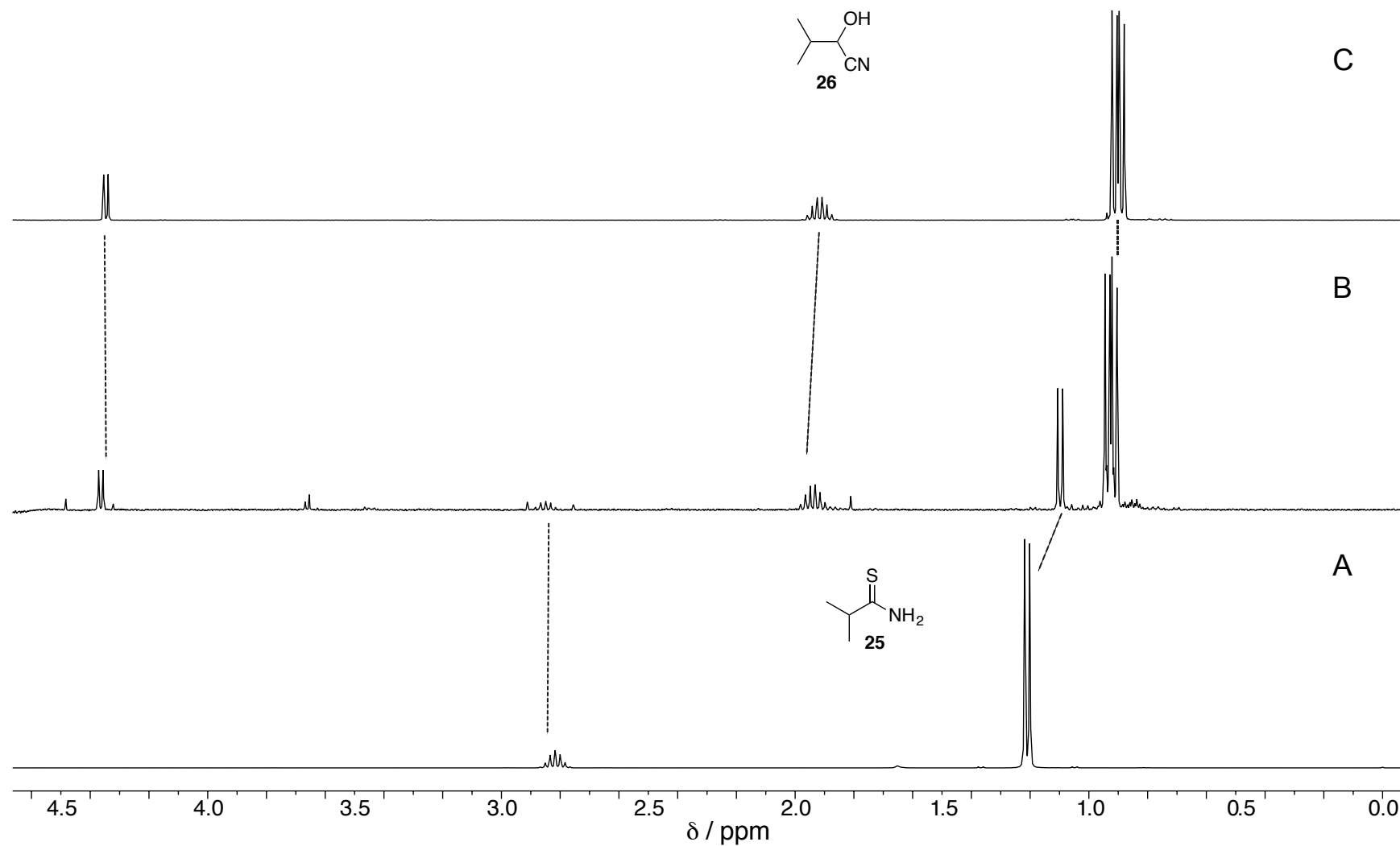
Figure S9. ^1\text{H-NMR} analysis of the conversion of the thioamide 25 into cyanohydrin 26 . A ( \text{CDCl}_3 ) – pure synthetic standard of thioamide 25 ; B ( \text{H}_2\text{O}/\text{D}_2\text{O} , 9:1) – the products of the photoreaction after 3 h of irradiation; C ^1\text{H-NMR} ( \text{H}_2\text{O}/\text{D}_2\text{O} , 9:1) – pure synthetic standard of cyanohydrin 26 prepared as described in the following section.
