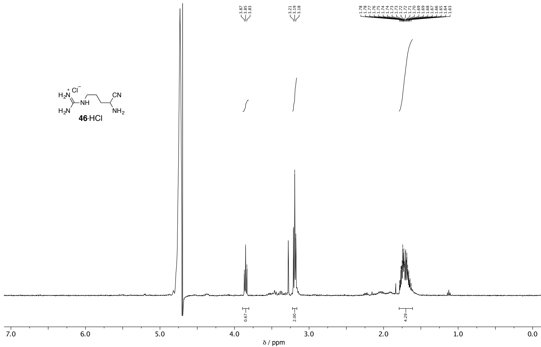
Figure S31. ^1\text{H-NMR} spectrum of \alpha -aminonitrile 46 ·HCl generated from cyanohydrin hydrochloride 45 ·HCl.
