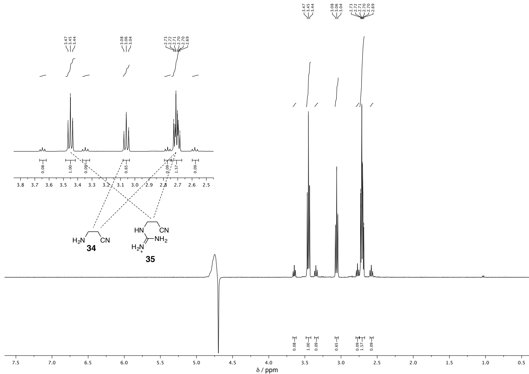
Figure S22. ^1\text{H-NMR} analysis ( \text{H}_2\text{O}/\text{D}_2\text{O} , 9:1) of the guanidinylation of aminopropionitrile 34 to give 35 .
