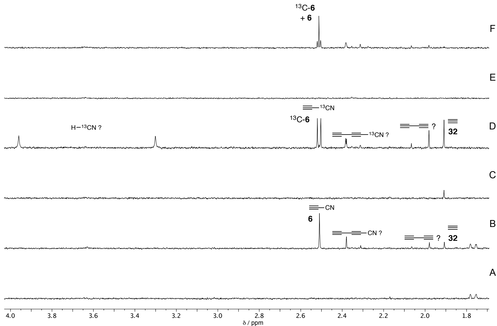
Figure S33. ^1\text{H} -NMR analysis ( \text{CDCl}_3 ) of the formation of cyanoacetylene 6 from acetylene 32 and \text{HCN}/\text{H}^{13}\text{CN} 11 / ^{13}\text{C} - 11 – expansion of spectra from Figure S32. Question marks indicate inferred assignments. A – KCN experiment: extract after 3 h; B – KCN experiment + KCN: extract after 3 h; C – \text{K}^{13}\text{CN} experiment: extract after 3 h; D – \text{K}^{13}\text{CN} experiment + \text{K}^{13}\text{CN} : extract after 3 h; E – KCN experiment: extract after 3 h; F – KCN experiment + \text{K}^{13}\text{CN} : extract after 3 h, showing both cyanoacetylene 6 and ^{13}\text{C} -cyanoacetylene ^{13}\text{C} - 6 .
