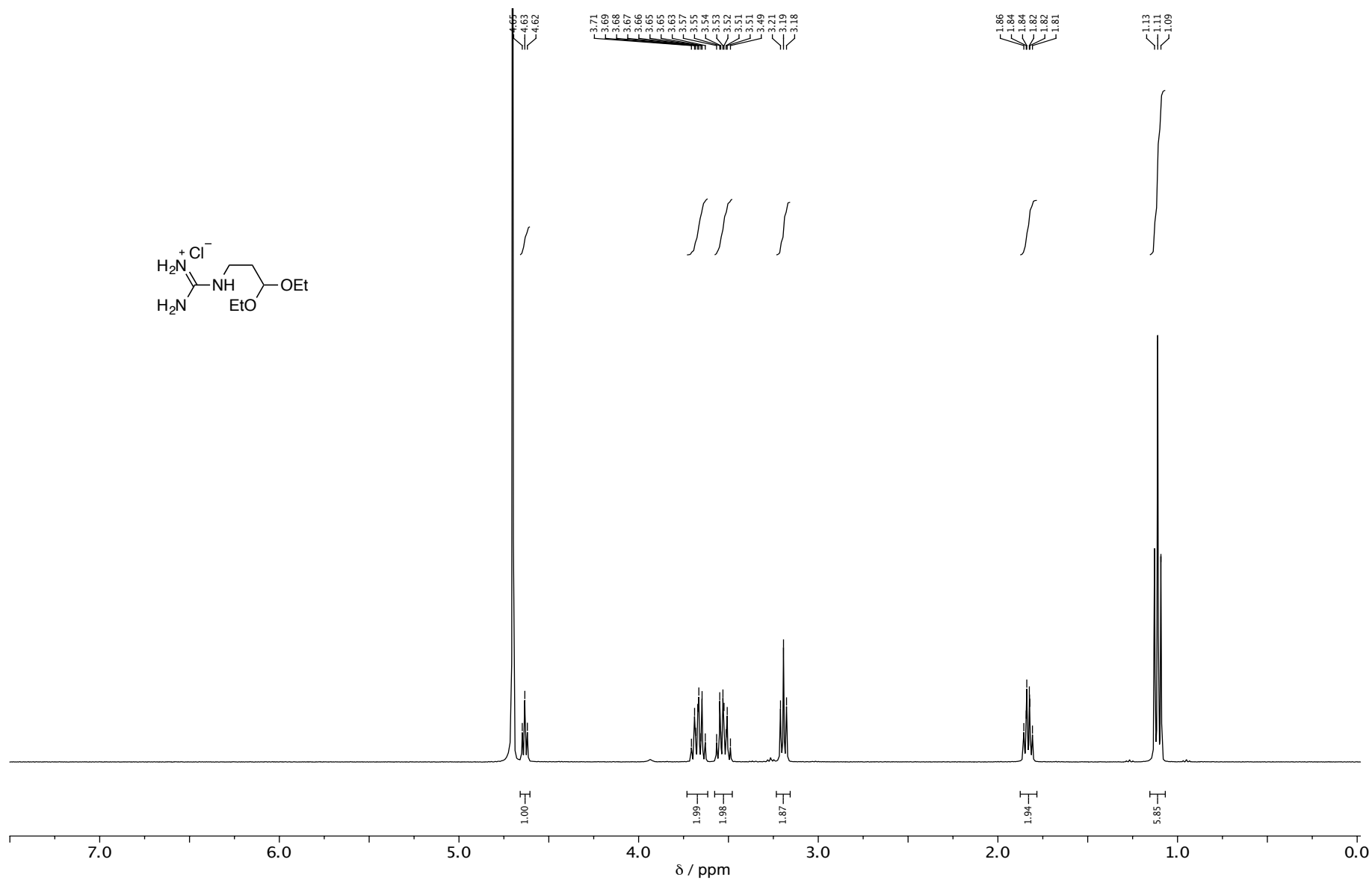
Figure S23. 1 H-NMR spectrum of amino((3,3-diethoxypropyl)amino)methaniminium hydrochloride.
