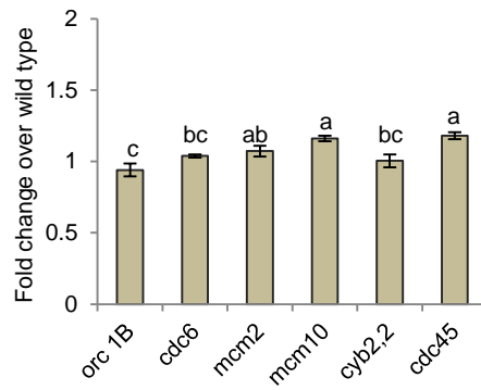
S4 Figure: Expression analysis of cell-cycle regulating genes in EcbHLH57 expressing transgenic plants under normal growth conditions. Graph depicting qRT-PCR analysis of cell-cycle regulating genes. Data represent mean of three replications (n = 3) and bars indicate standard error. The lowercase letters that are different indicate significant difference (Duncan's multiple range test, P < 0.05 ) between means of analyzed genes.
