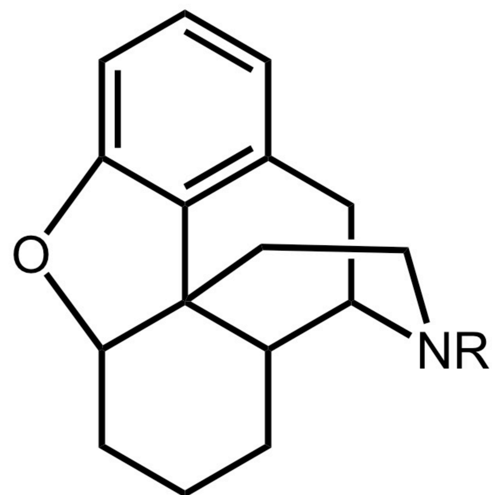
Morphinan
