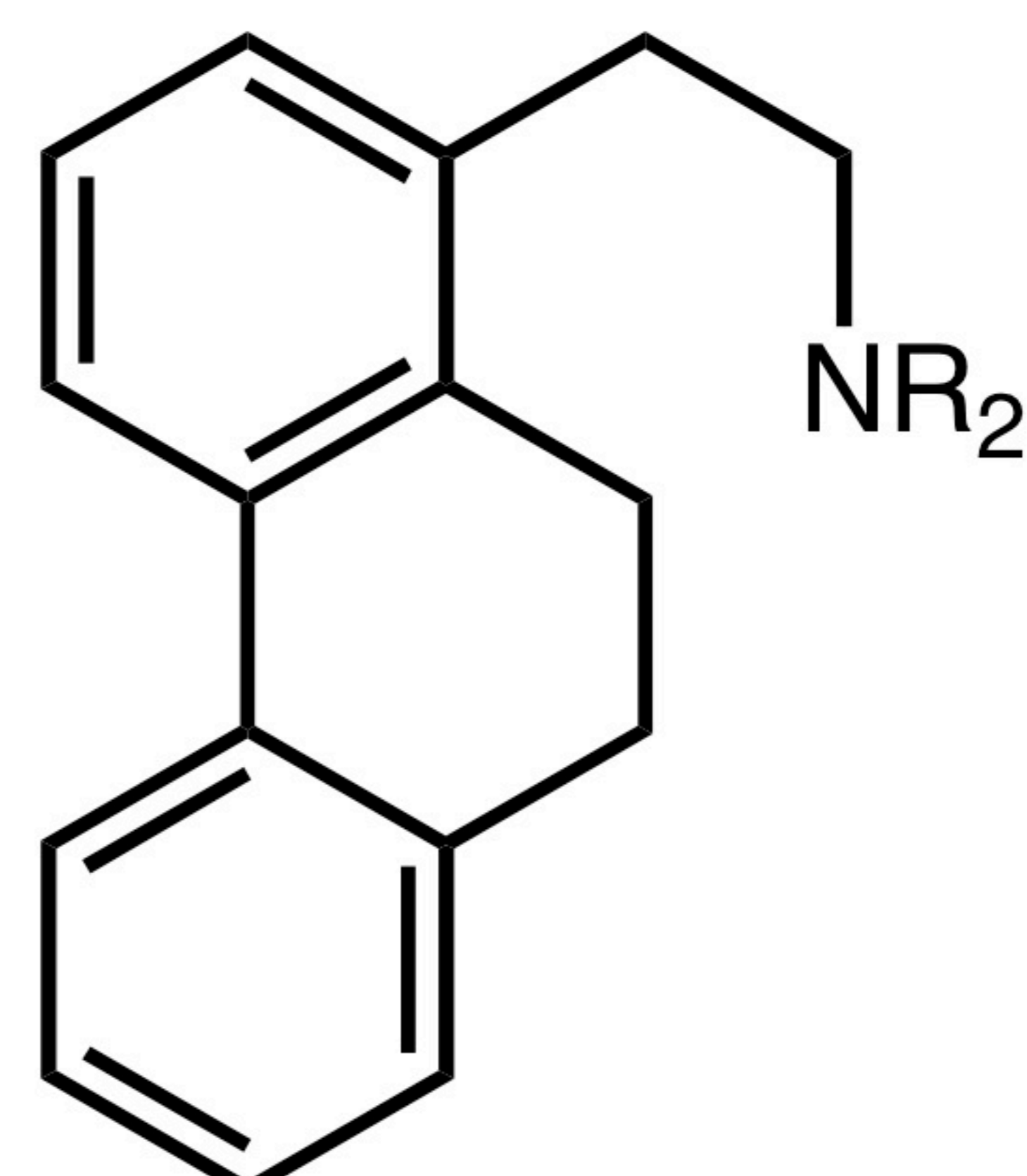
Secoisoquinoline
