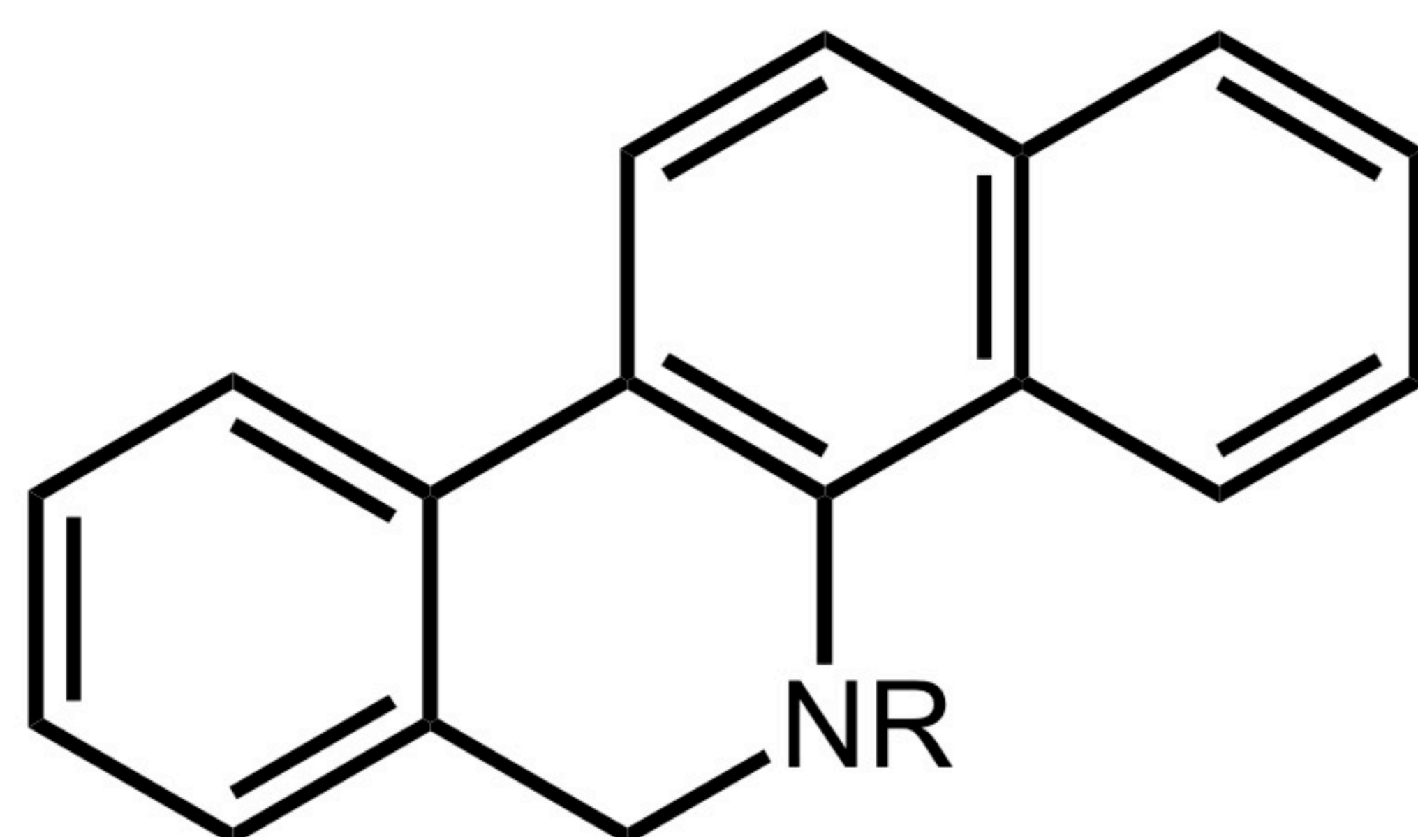
Benzo[c]phenanthridine
