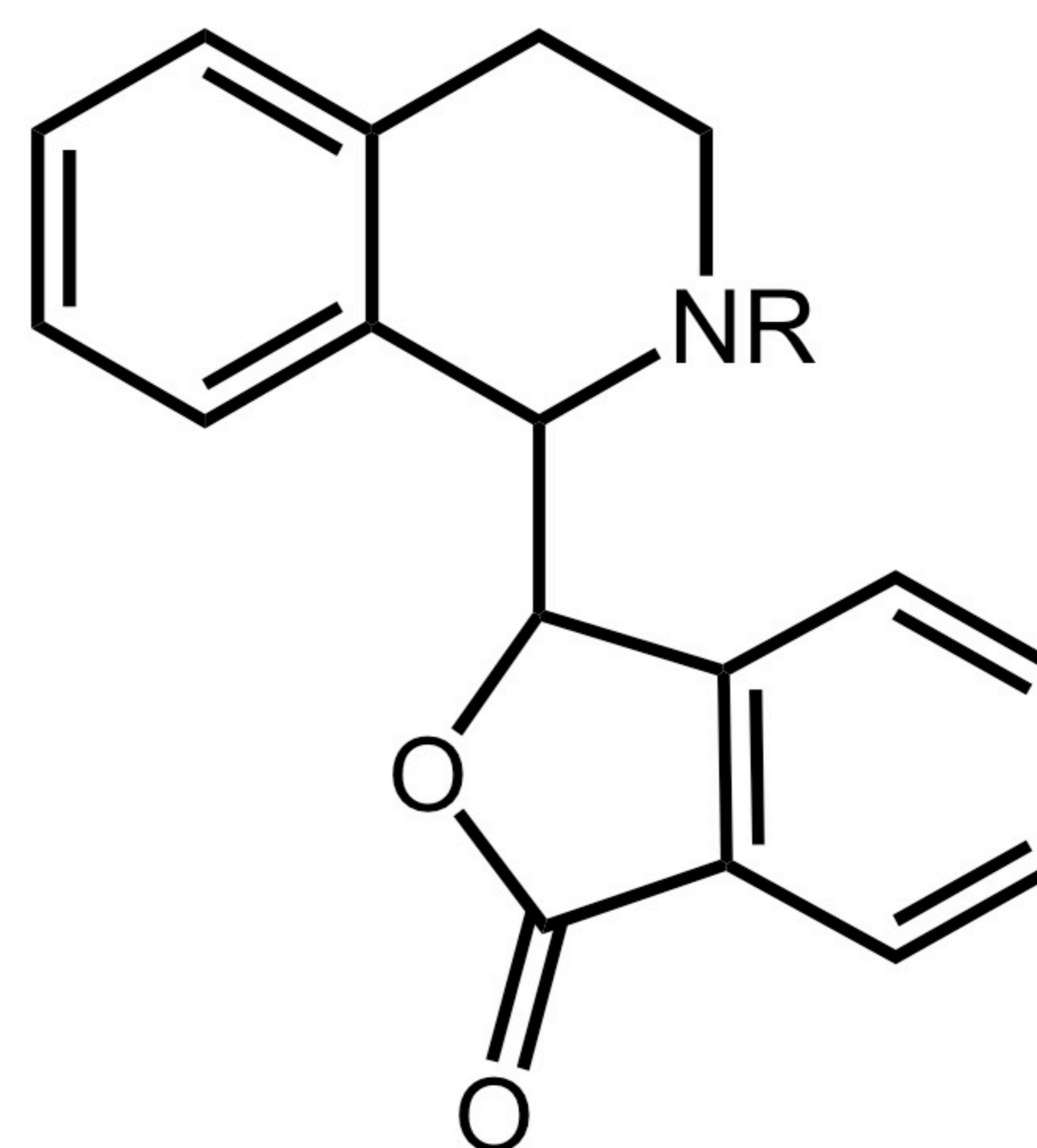
Phthalideisoquinoline
