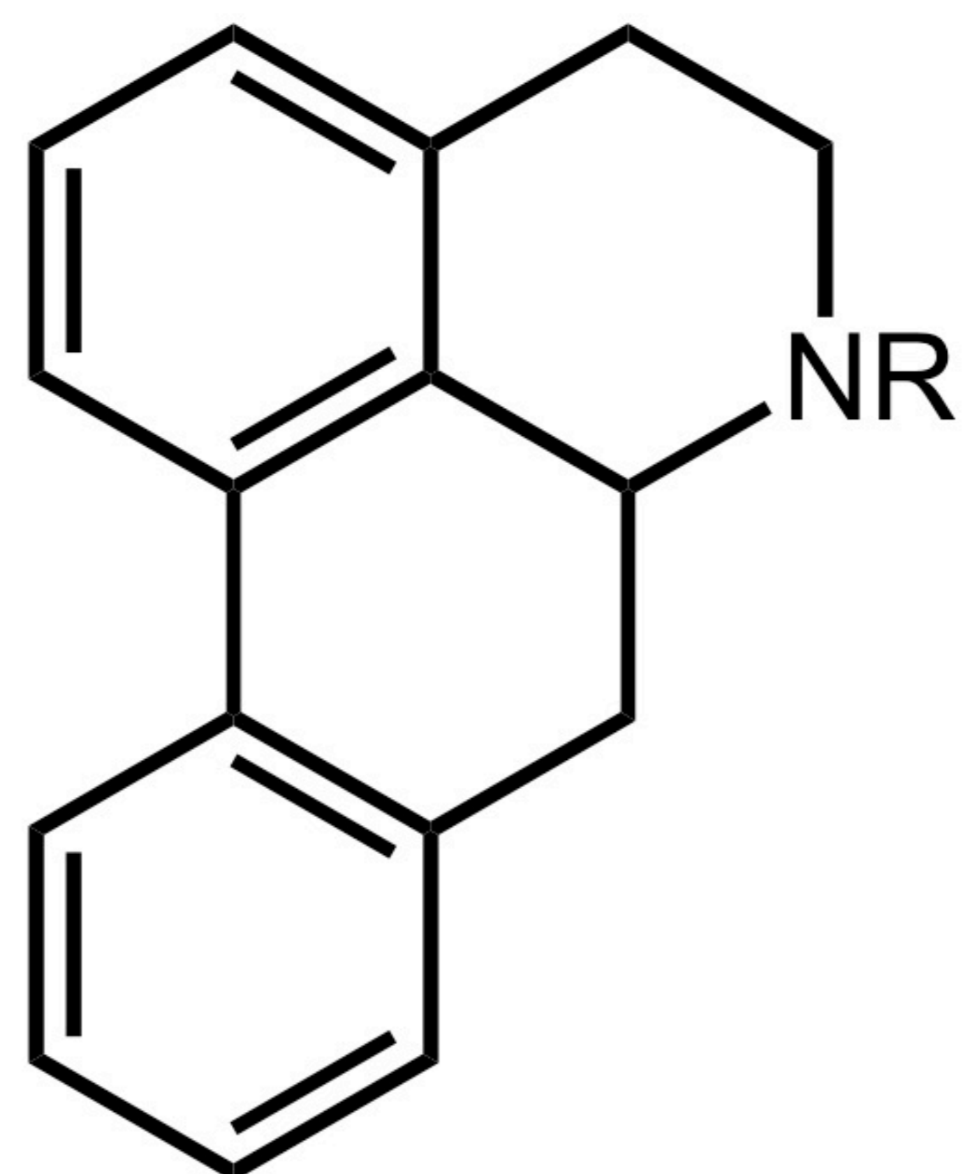
Aporphine
