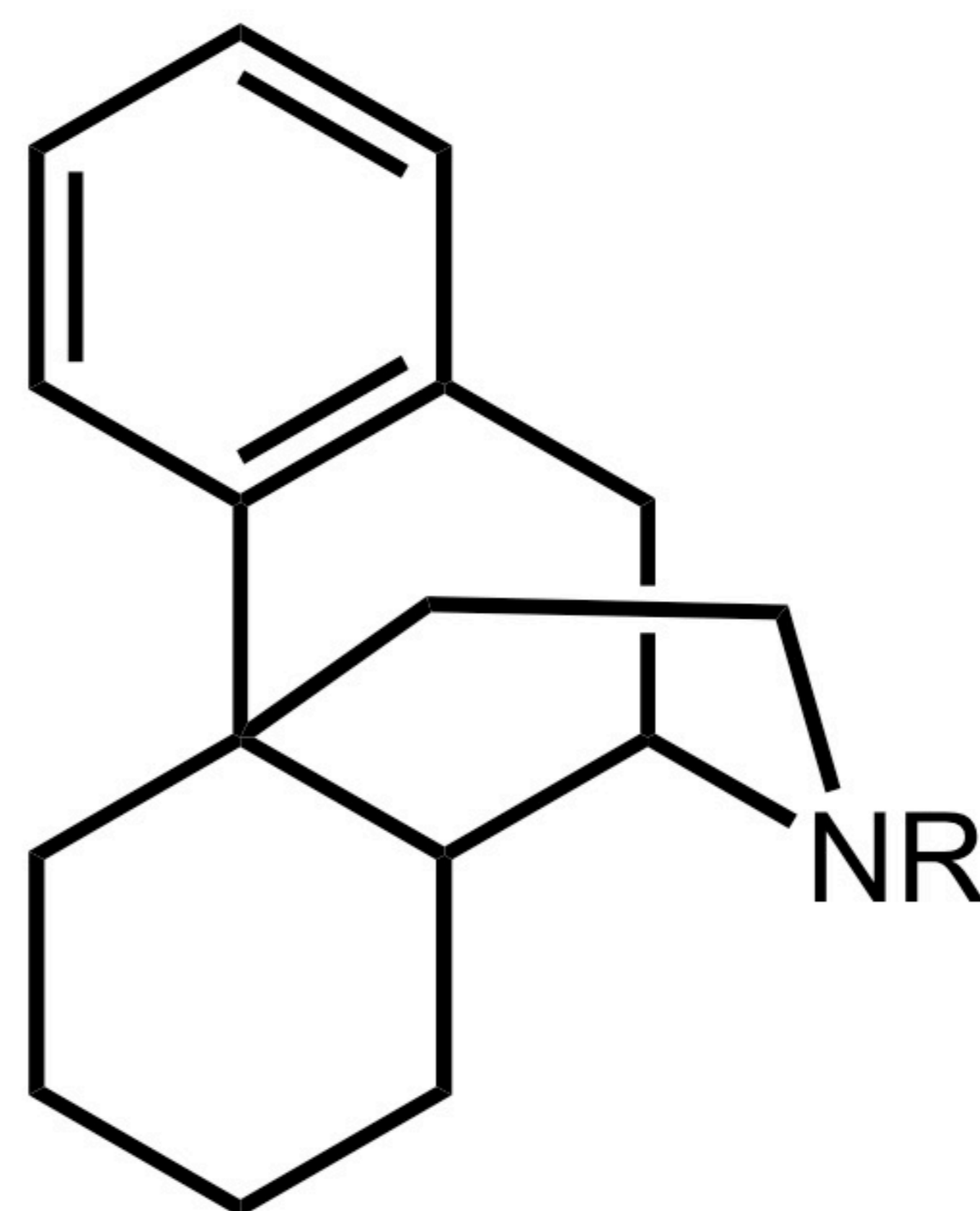
Promorphinan
