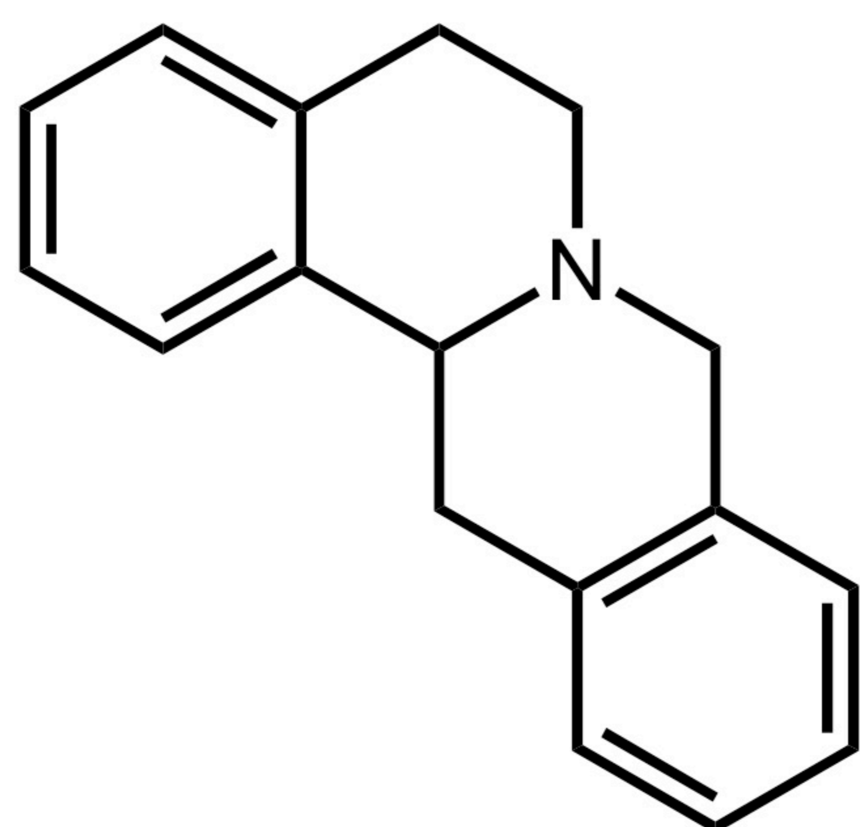
Protoberberine
