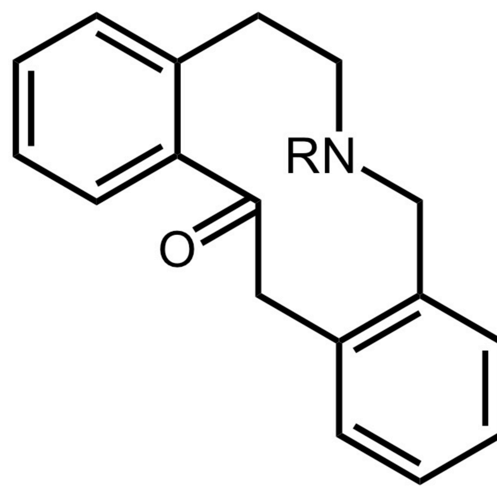
Protopine
