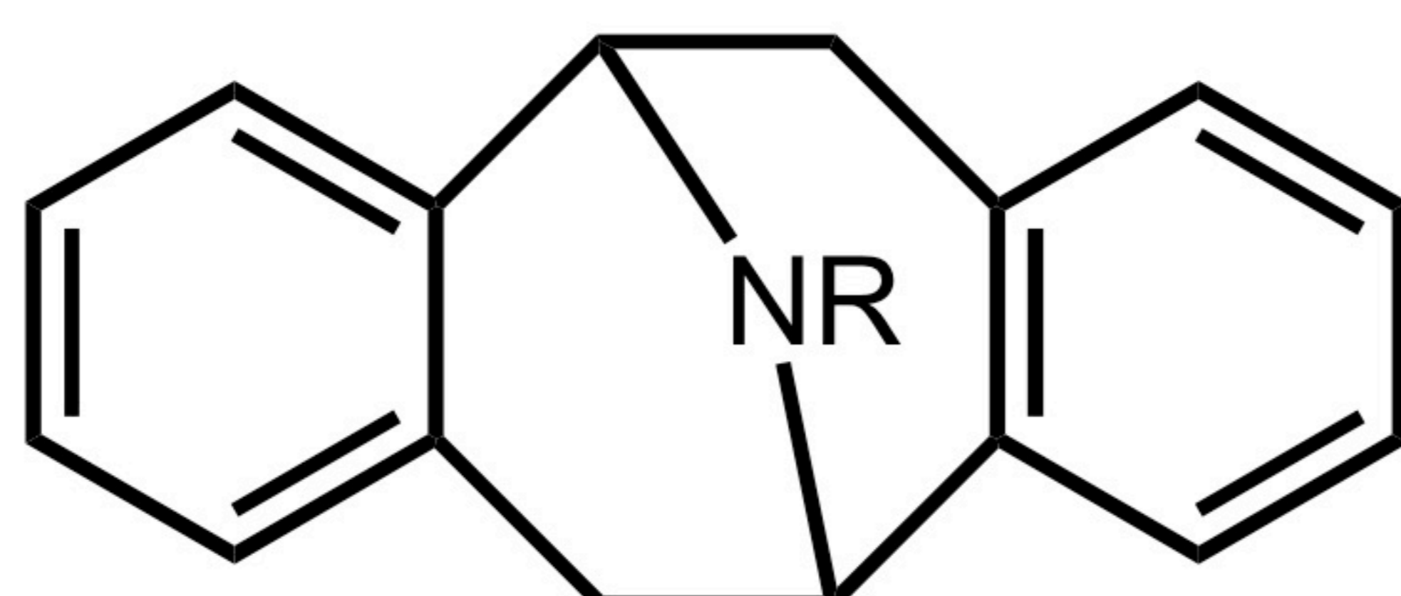
Pavine
