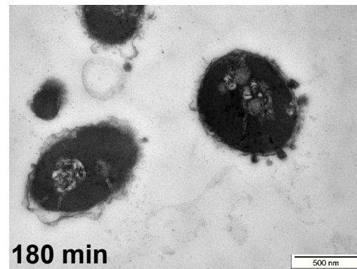
S2 Fig.: Effect of FLG2-4 on P. aeruginosa . Electron microscopy images of P. aeruginosa treated with FLG2-4 for the indicated time periods (right panel). Left panel: untreated controls.
