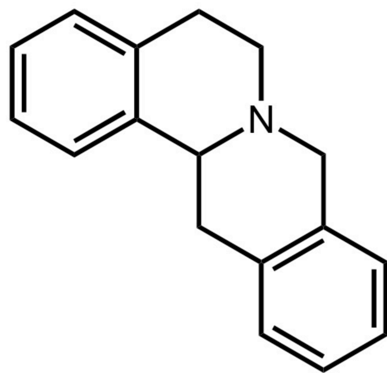
Protoberberine
