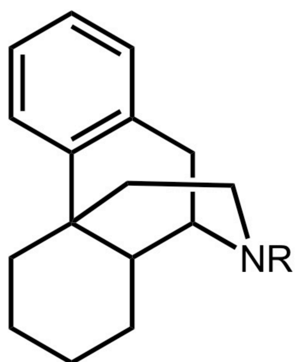
Promorphinan
