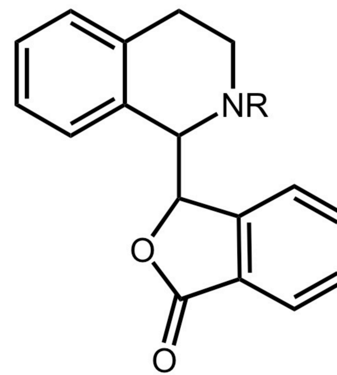
Phthalideisoquinoline
