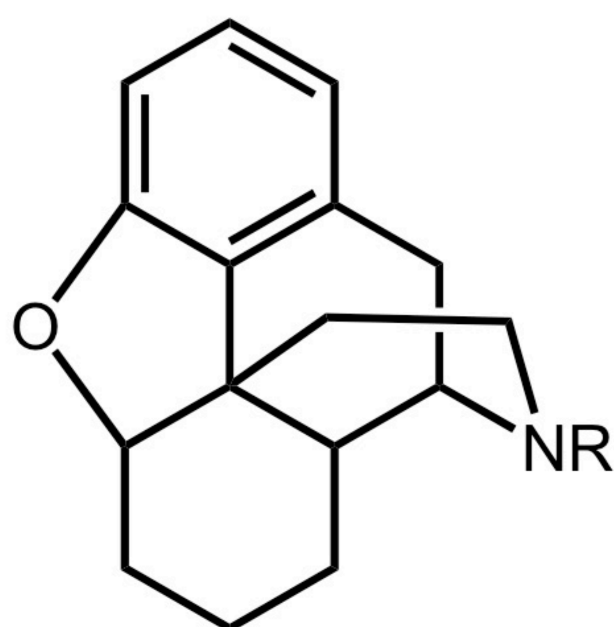
Morphinan
