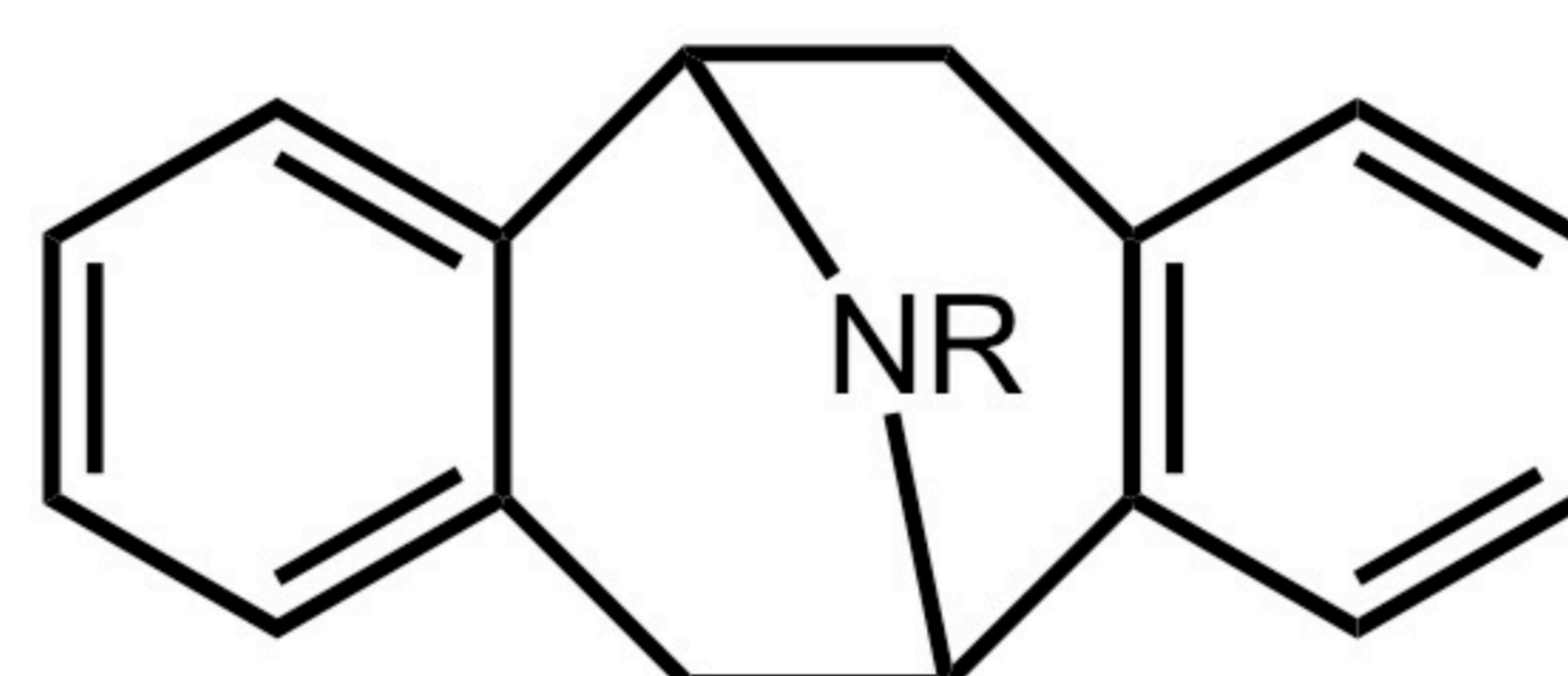
Pavine
