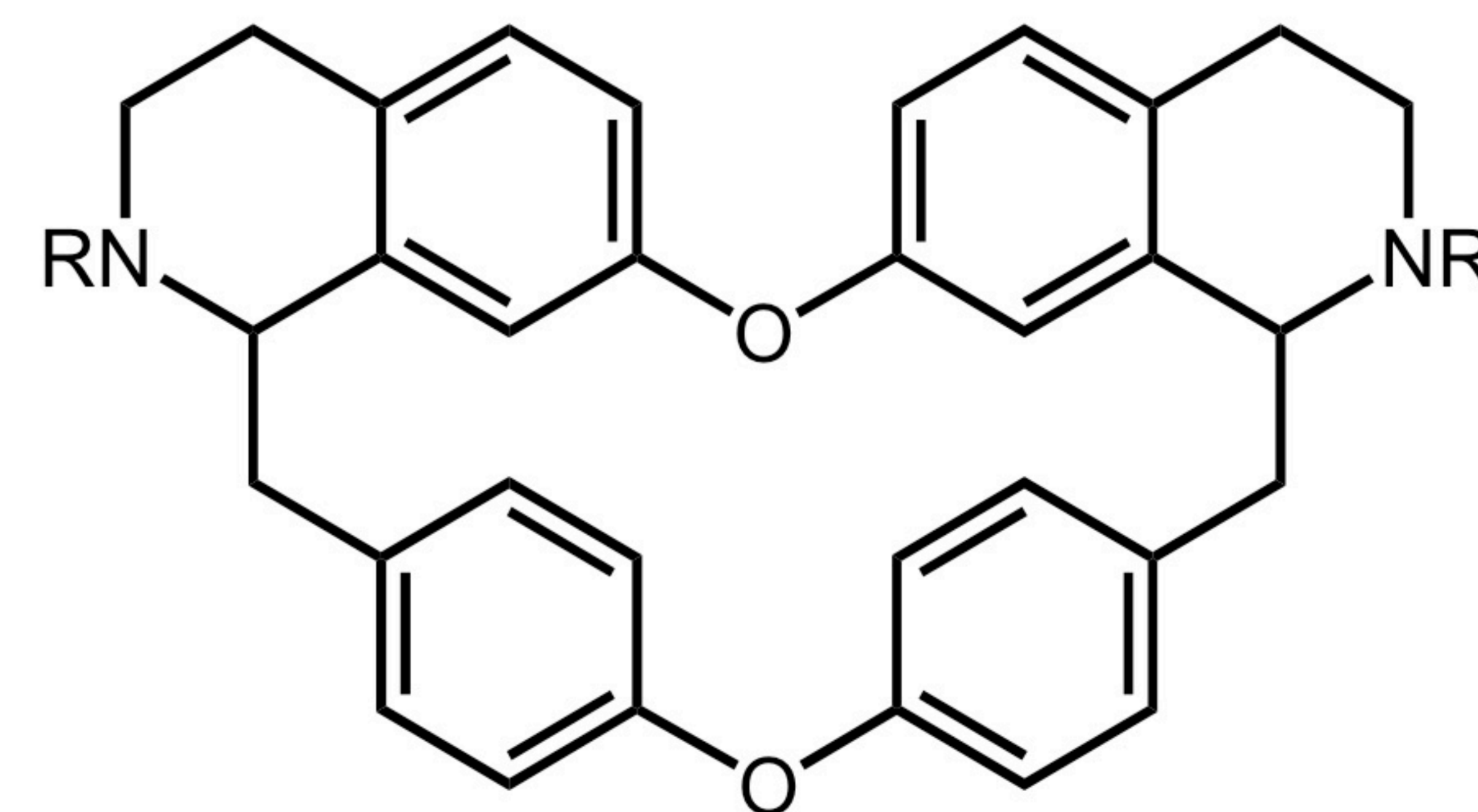
Bisbenzylisoquinoline
