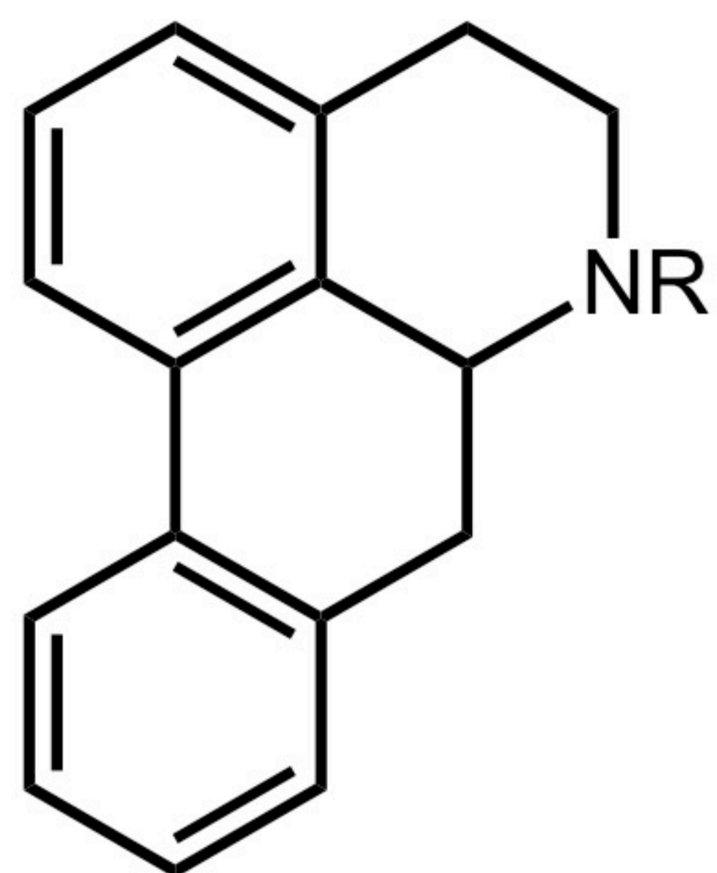
Aporphine
