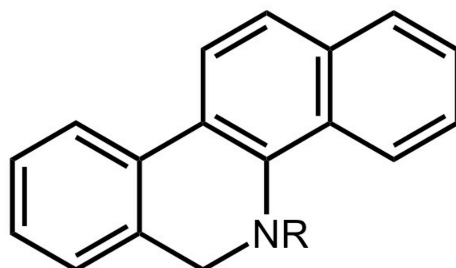
Benzo[c]phenanthridine
