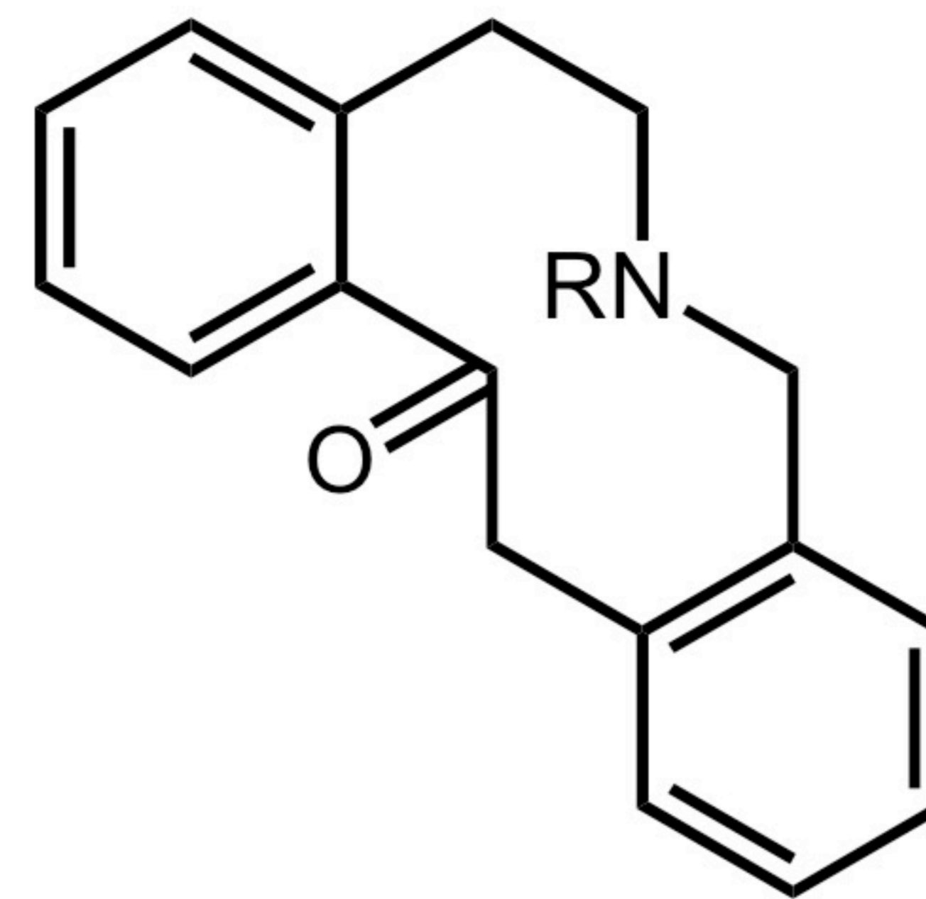
Protopine
