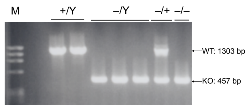
Genomic PCR
