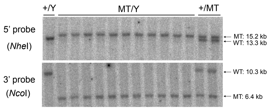
Southern blot
