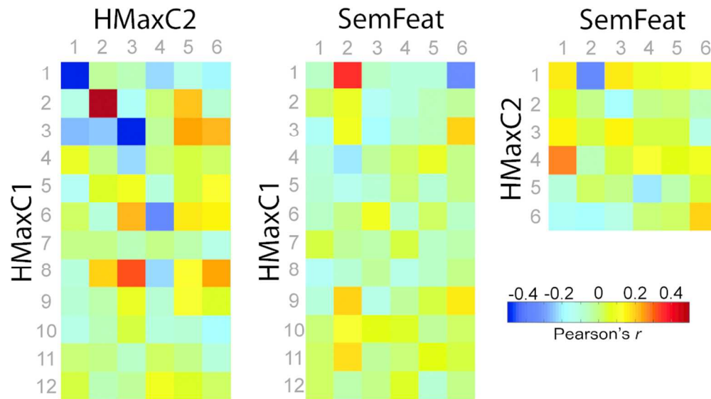
Figure S1. Correlations between model predictors. 101x56mm (300 x 300 DPI)
