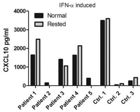
SUPPLEMENTARY FIG. S3. Variations in CXCL10 production in cells stimulated with IFN- \alpha (patients, n=5 and controls, n=3 ) directly after recovery from cryopreservation (as shown in Fig. 2) or after a resting period of 24 h.
