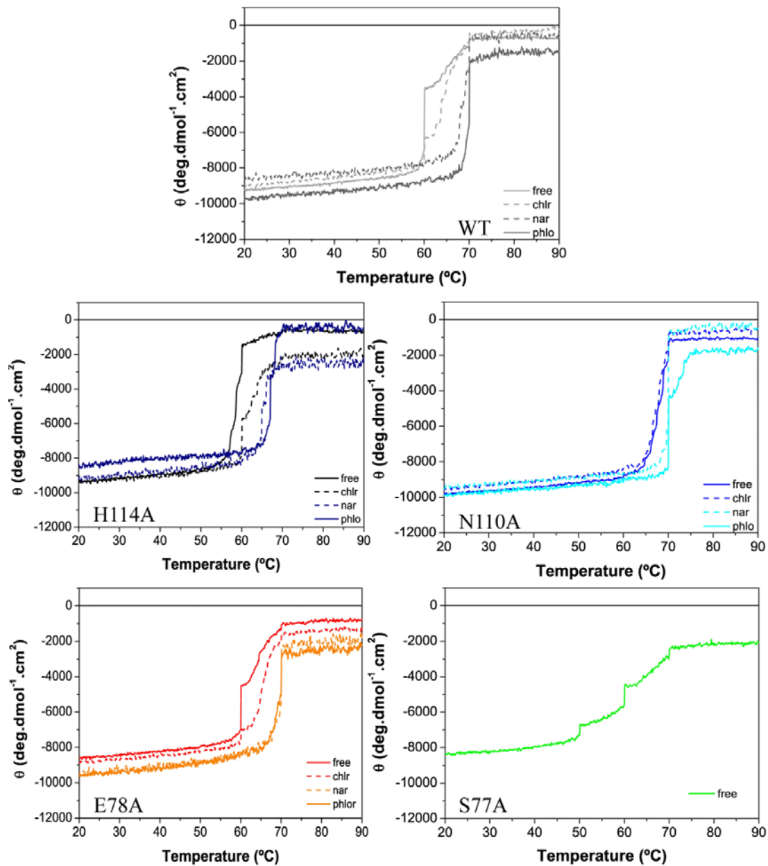
SI_Figure: Protein unfolding of TtgR WT and mutants in the presence of ligands monitored by CD ellipticity at 222 nm
