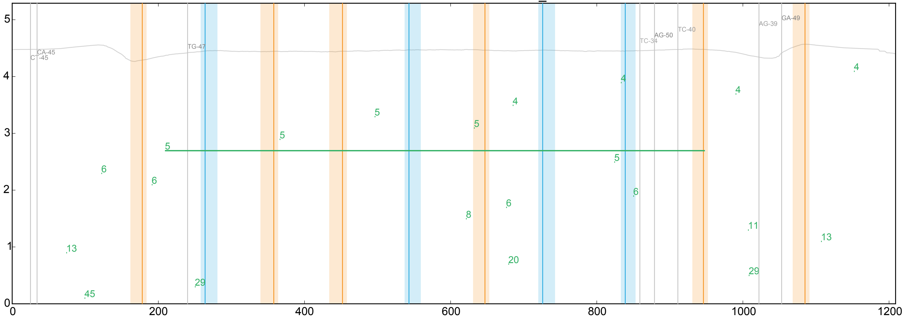
WT ENSDARG00000079738_5
