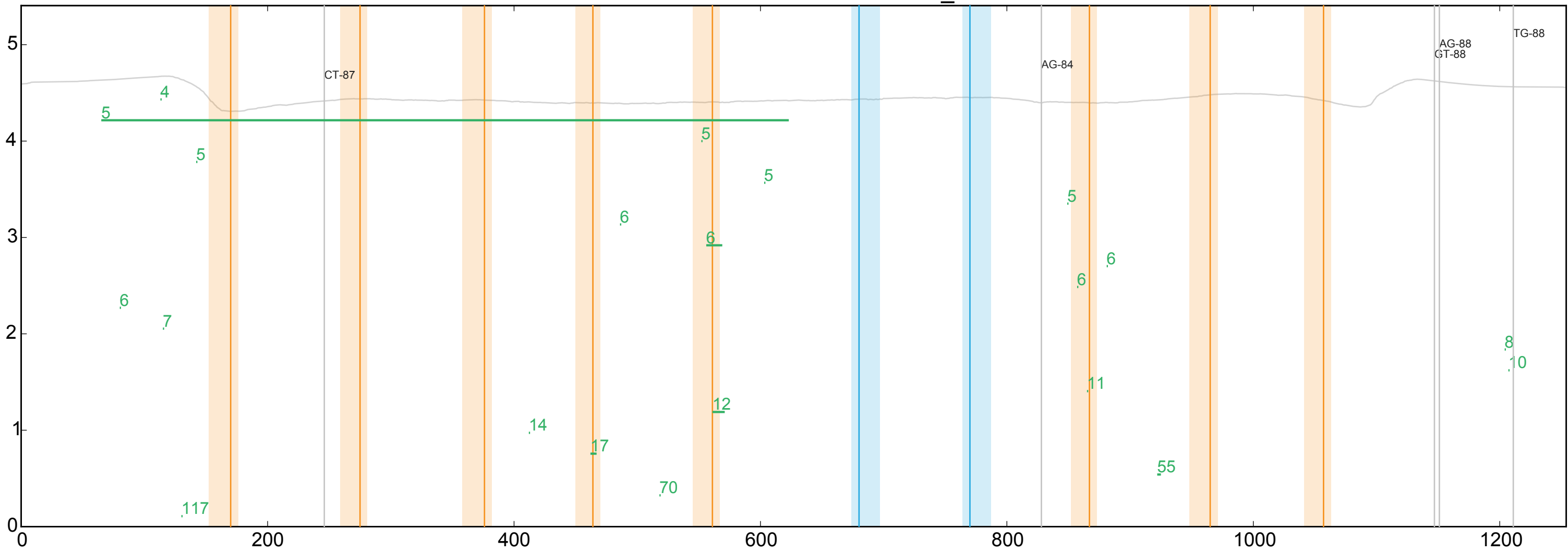
WT ENSDARG00000003469_0
