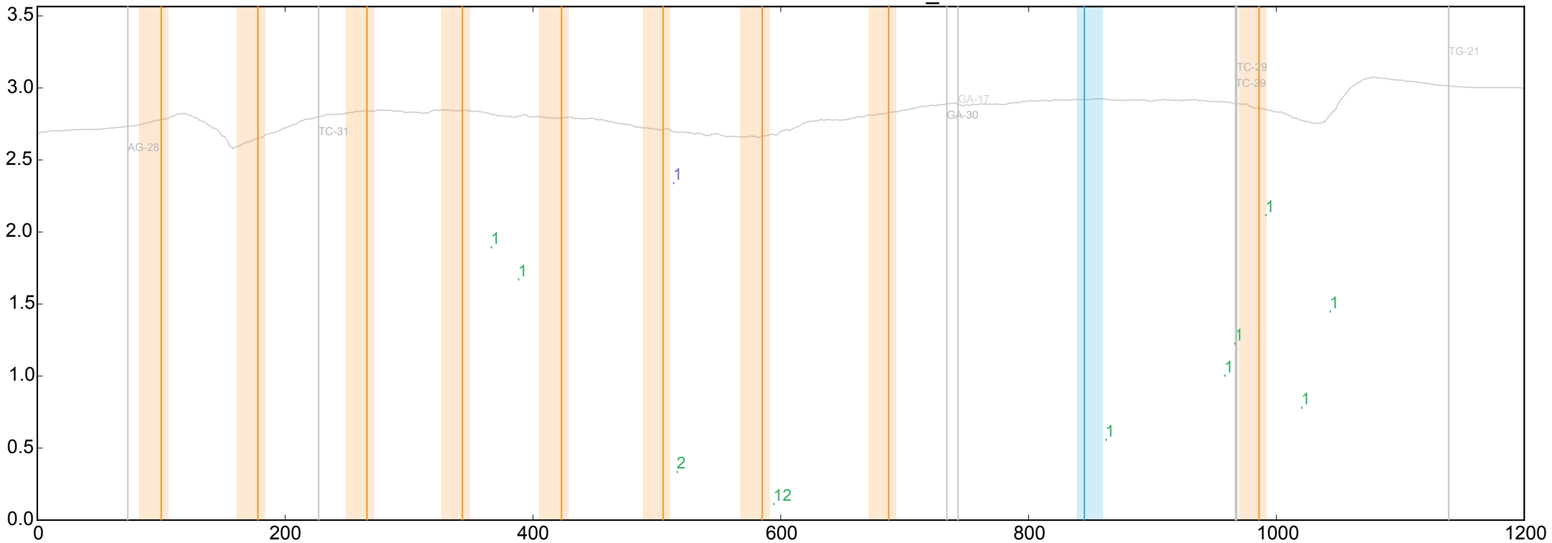
WT ENSDARG00000036245_3
