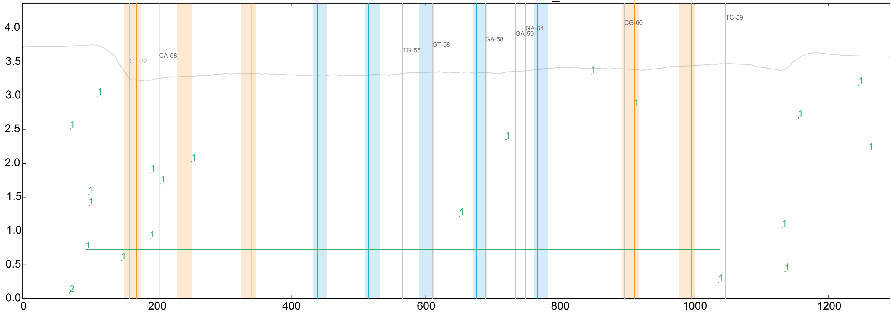
WT ENSDARG00000044671_0
