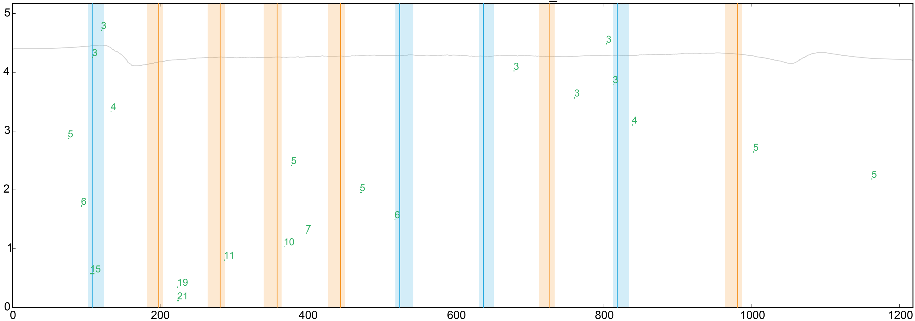
WT ENSDARG00000077489_1
