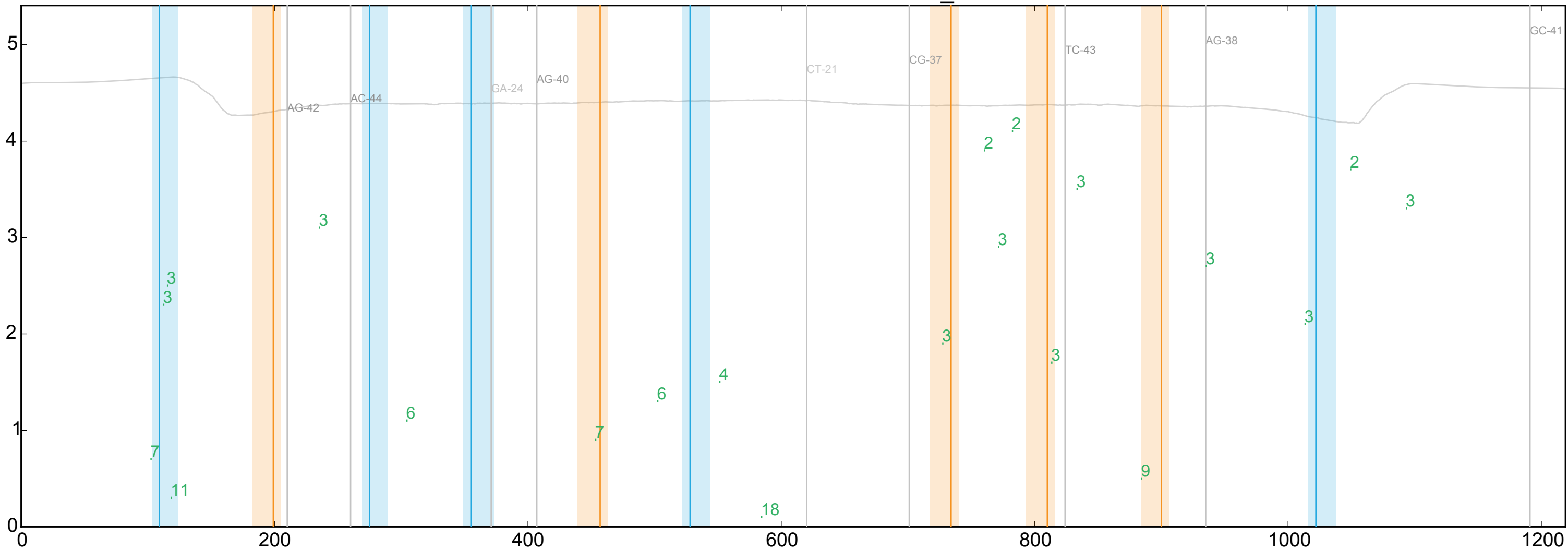
WT ENSDARG00000077293_7
