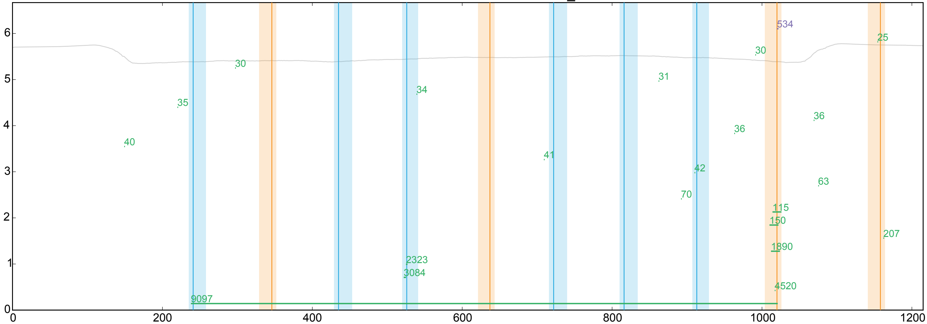
WT ENSDARG00000078251_0
