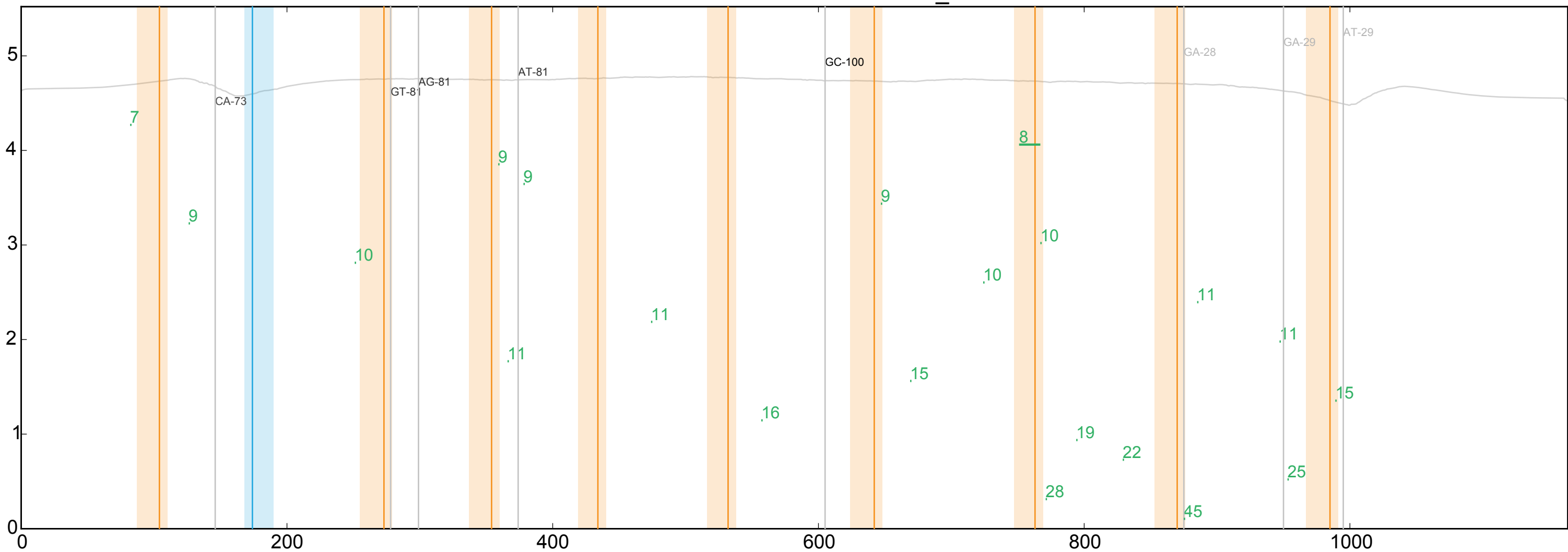
WT ENSDARG00000071150_18
