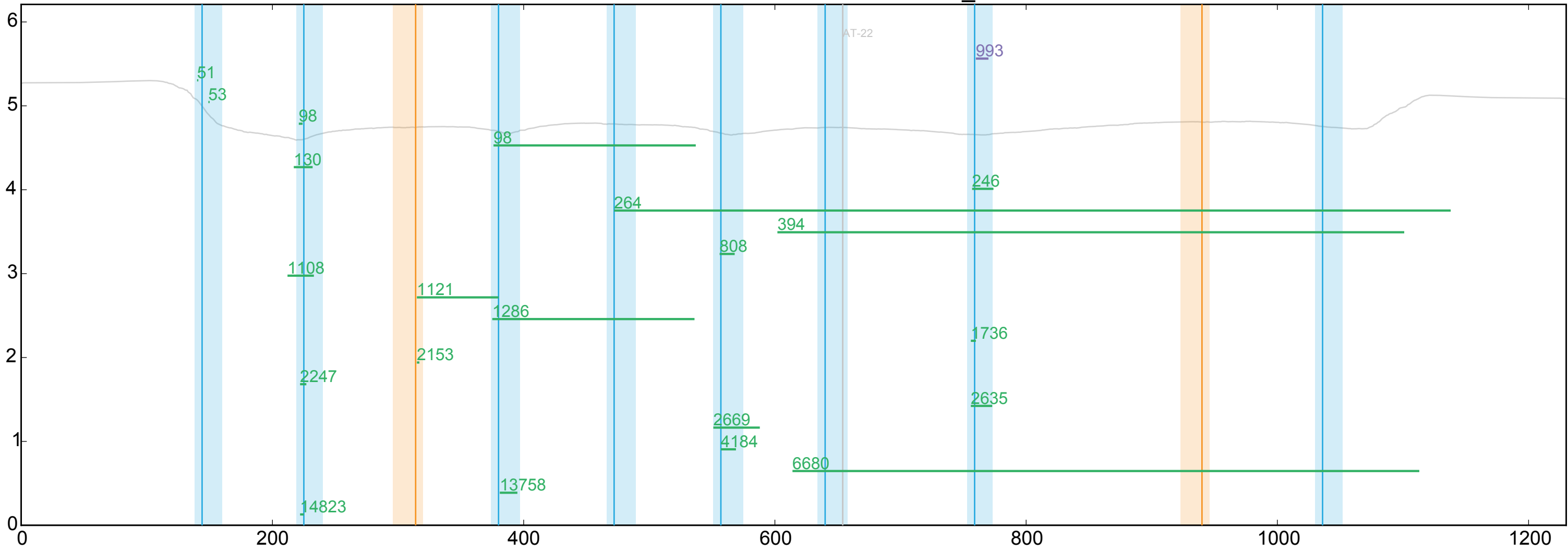
WT ENSDARG00000029045_5
