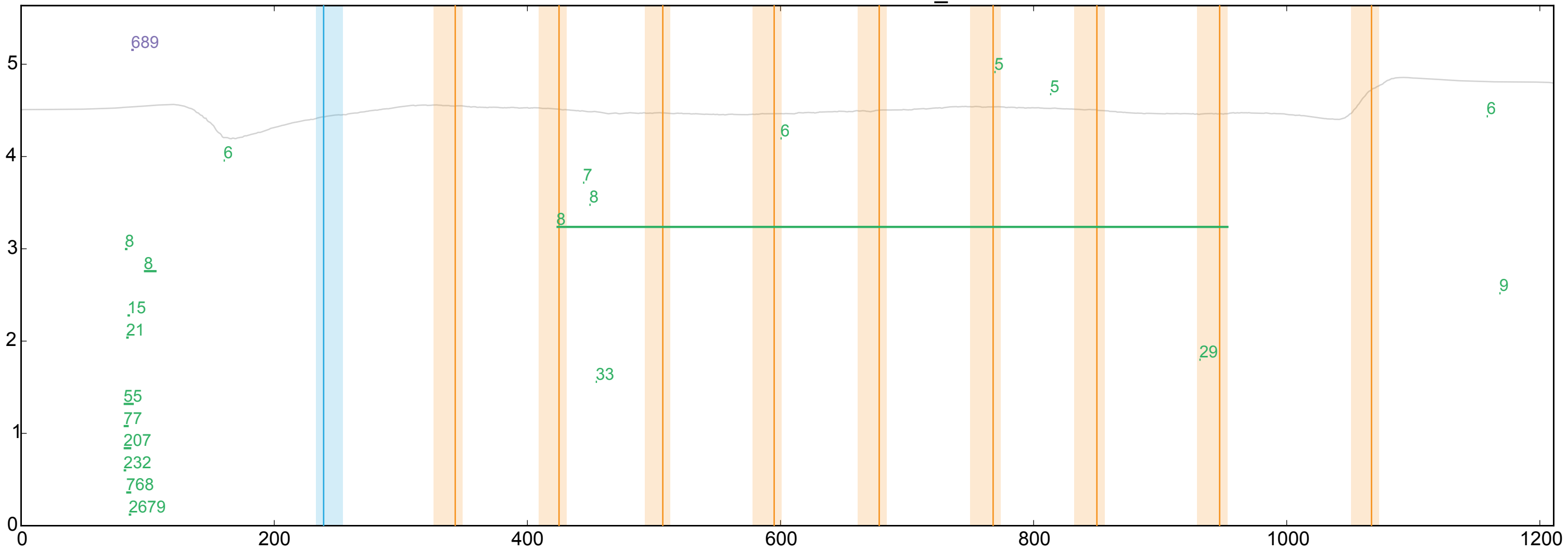
WT ENSDARG00000028415_0
