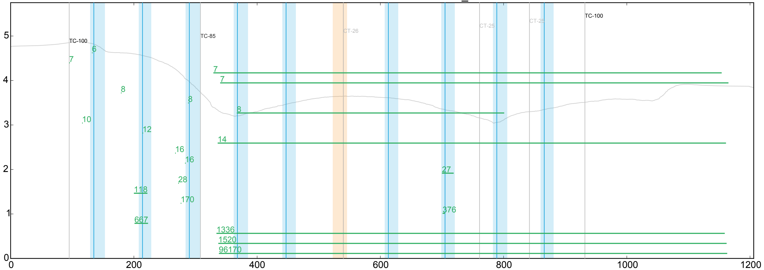
WT ENSDARG00000077353_15
