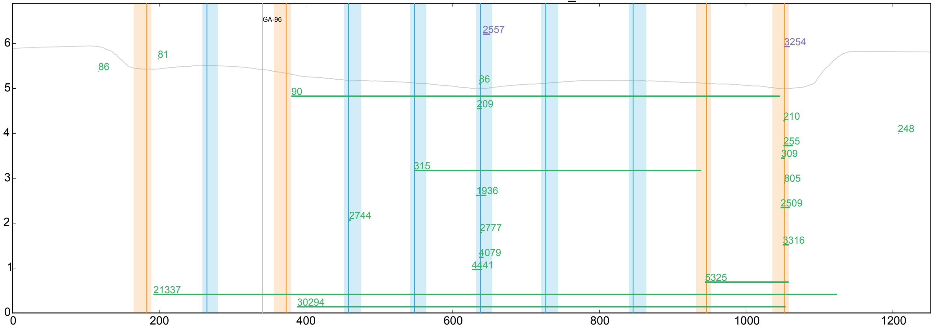
WT ENSDARG00000079097_24
