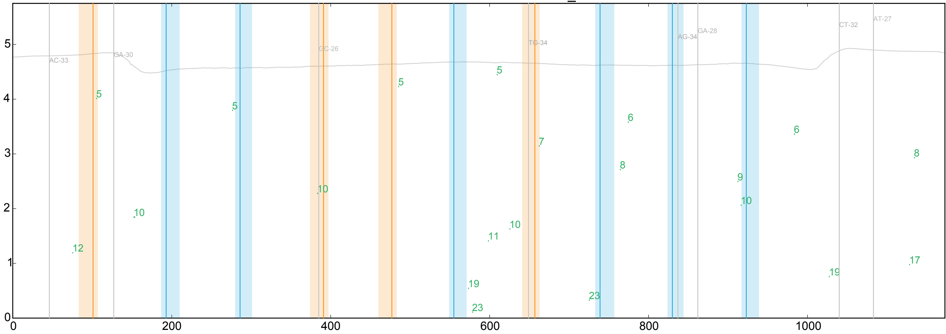
WT ENSDARG00000044098_0
