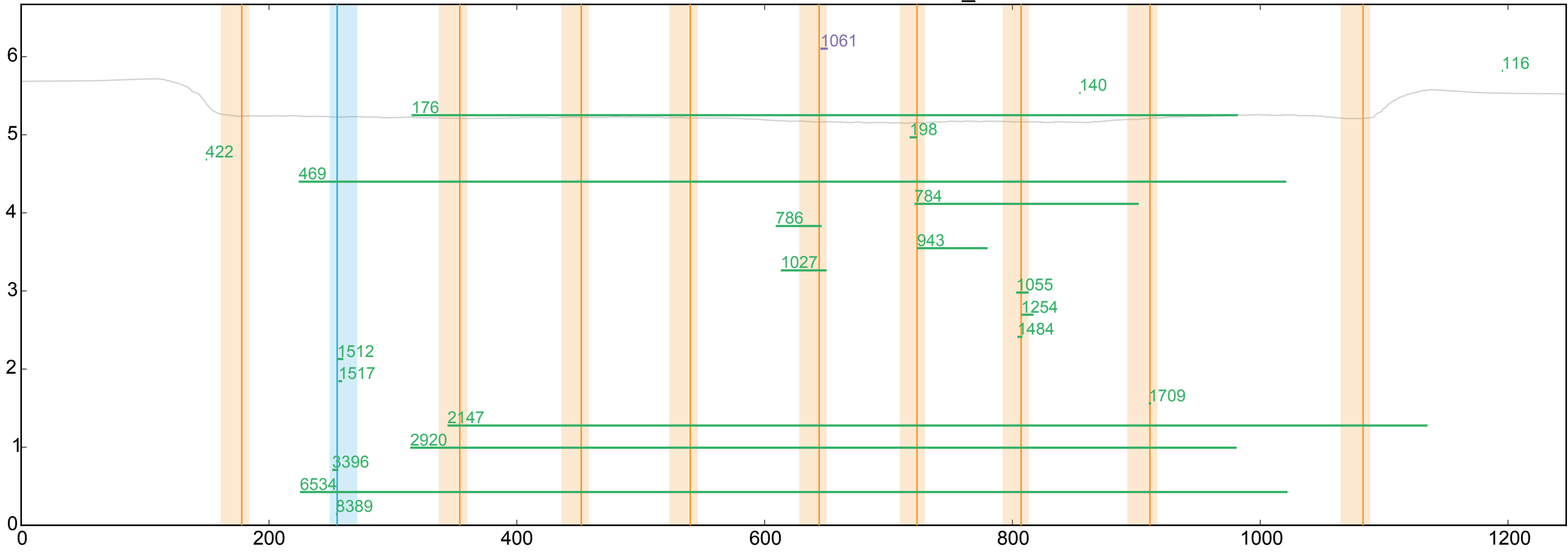
WT ENSDARG00000060697_9
