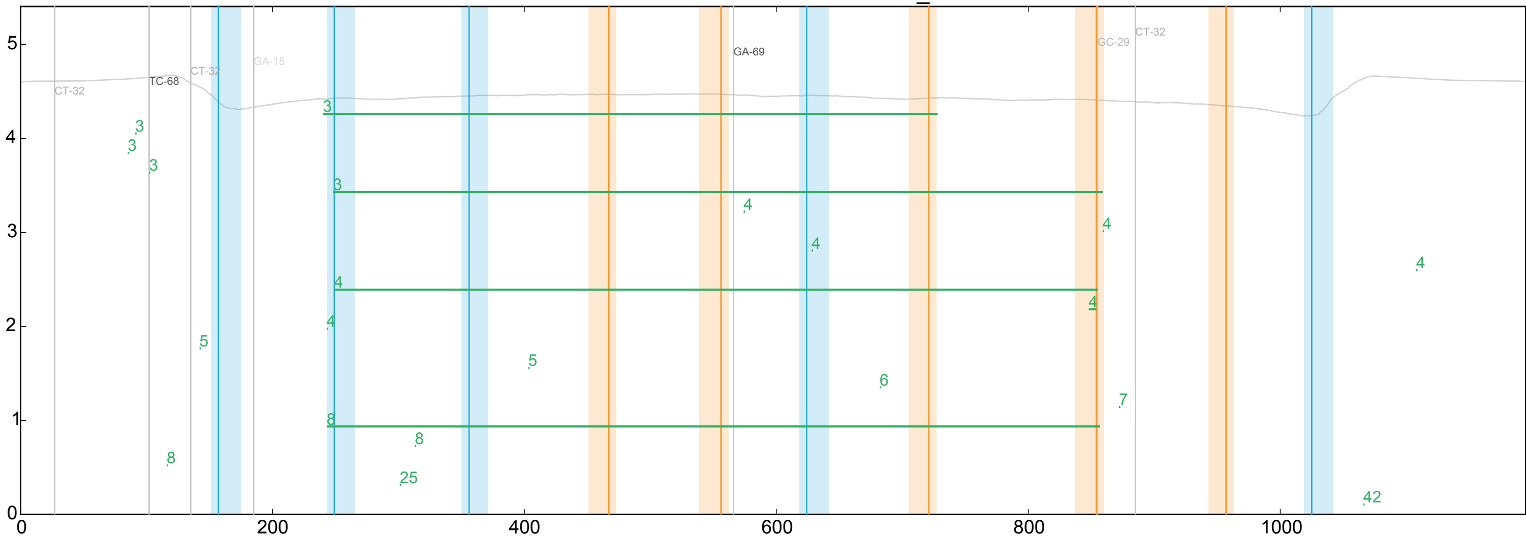
WT ENSDARG00000073817_2
