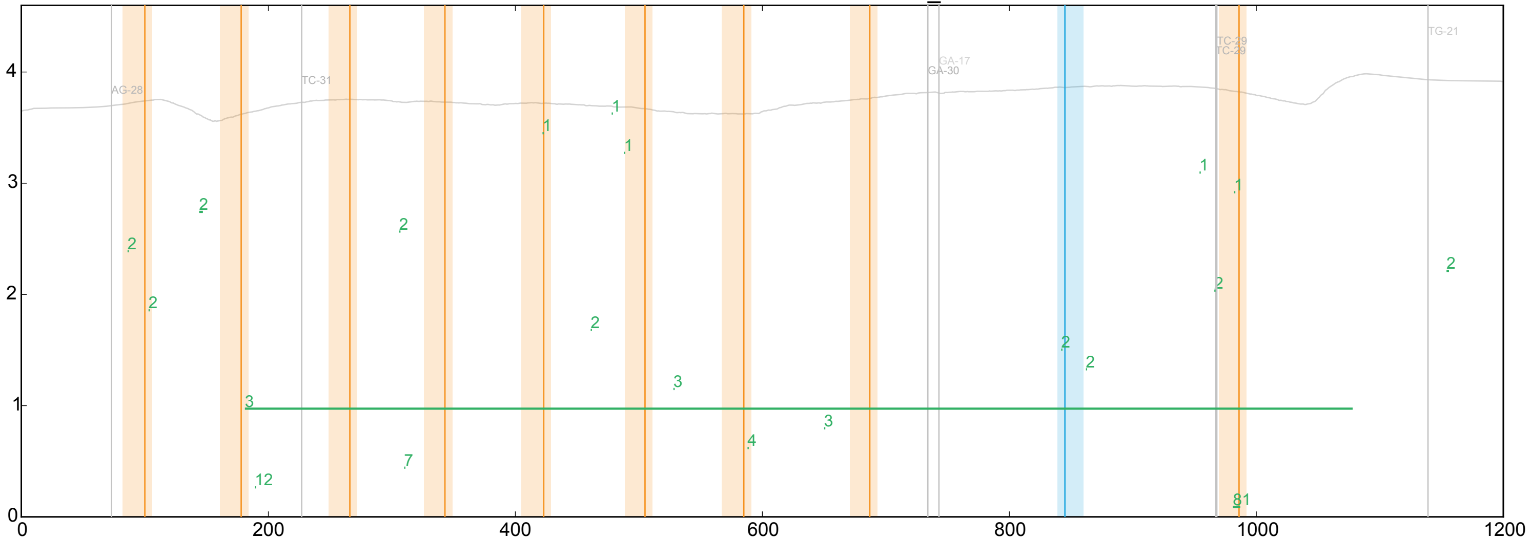
WT ENSDARG00000036245_3
