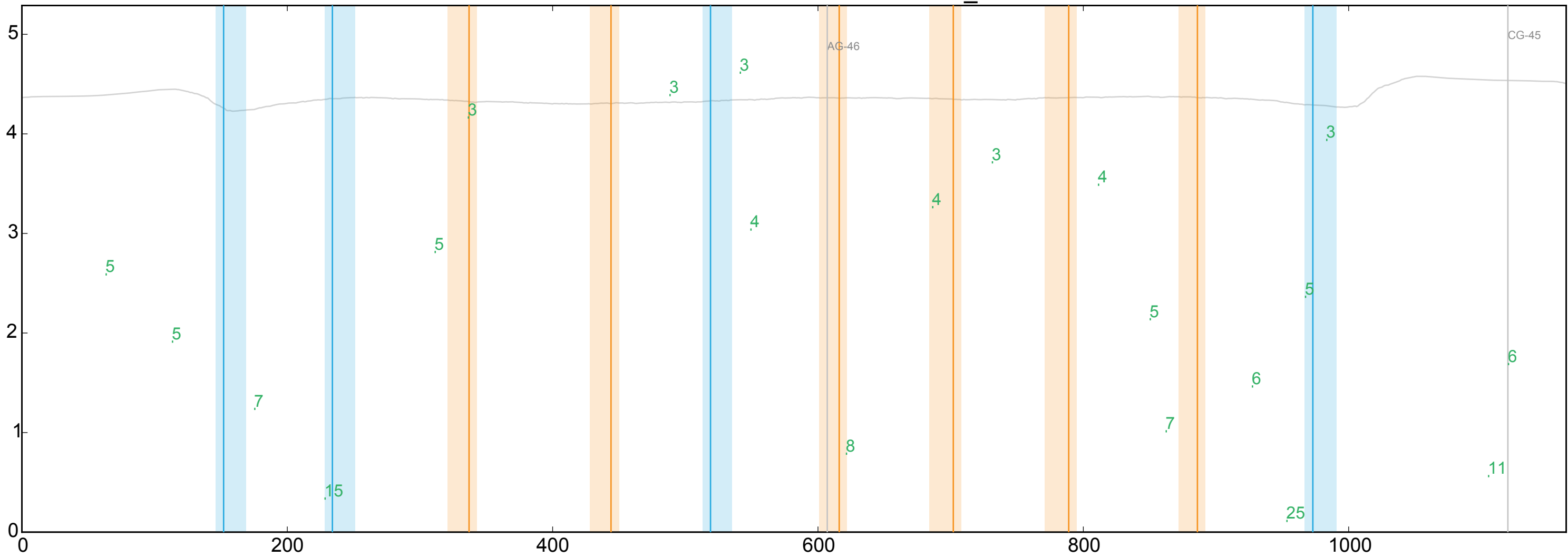
WT ENSDARG0000055054_0
