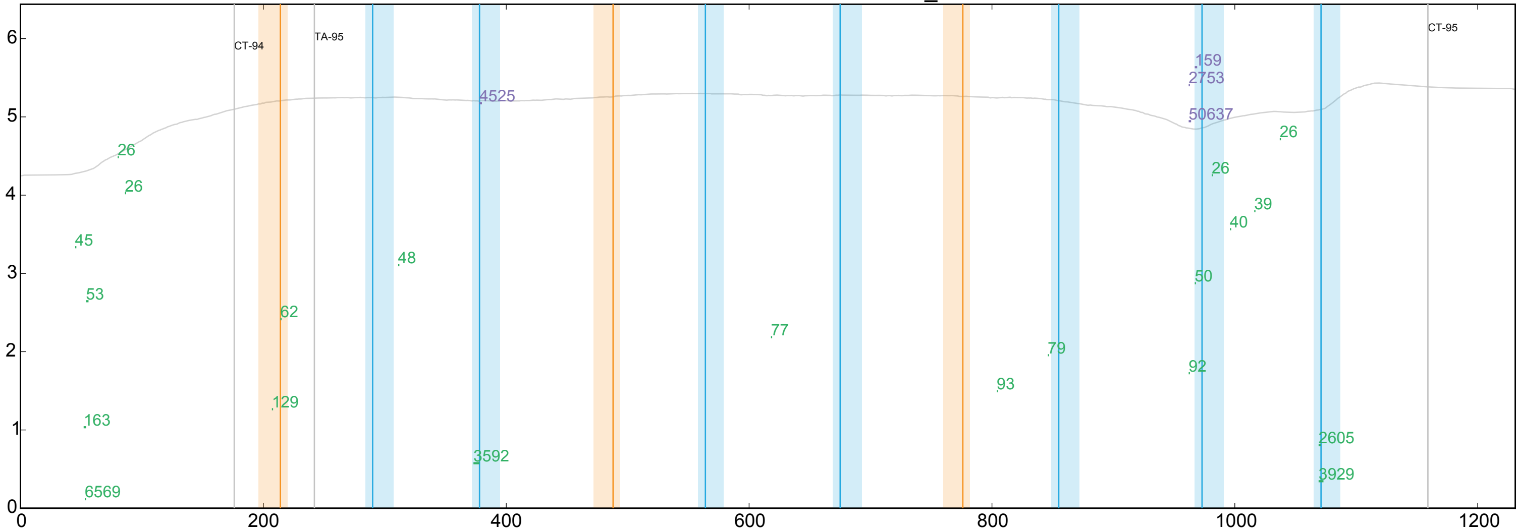
WT ENSDARG00000060073_17
