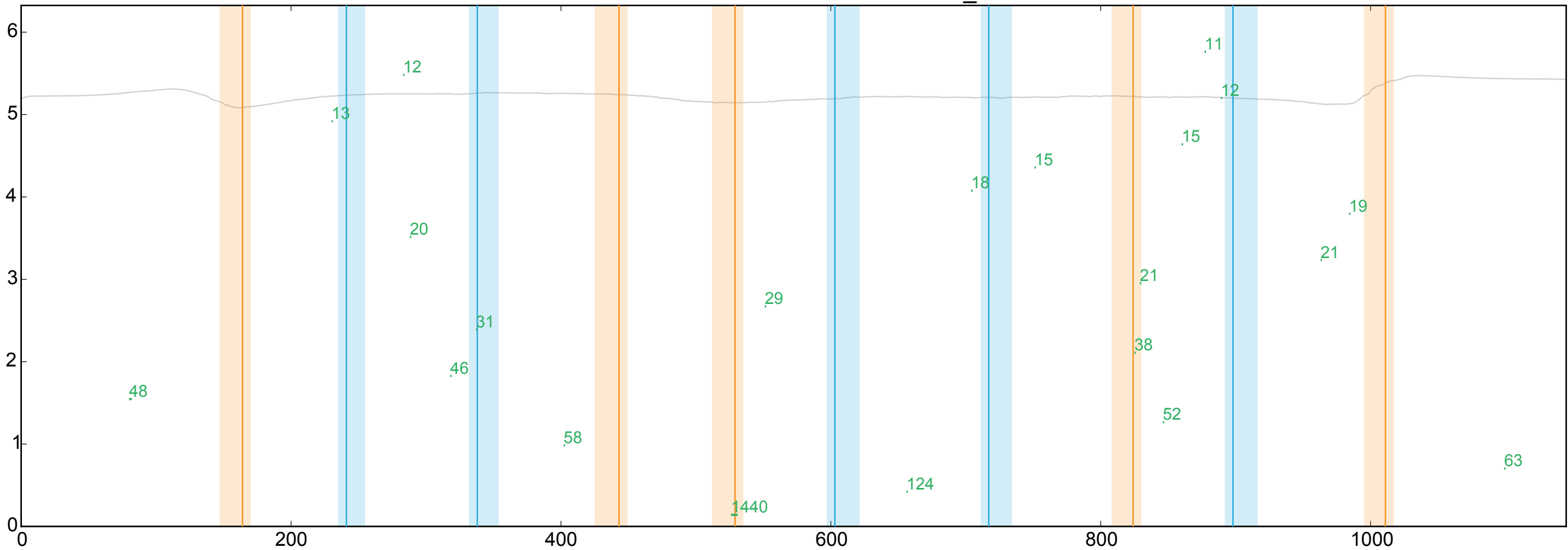
WT ENSDARG00000010770_1
