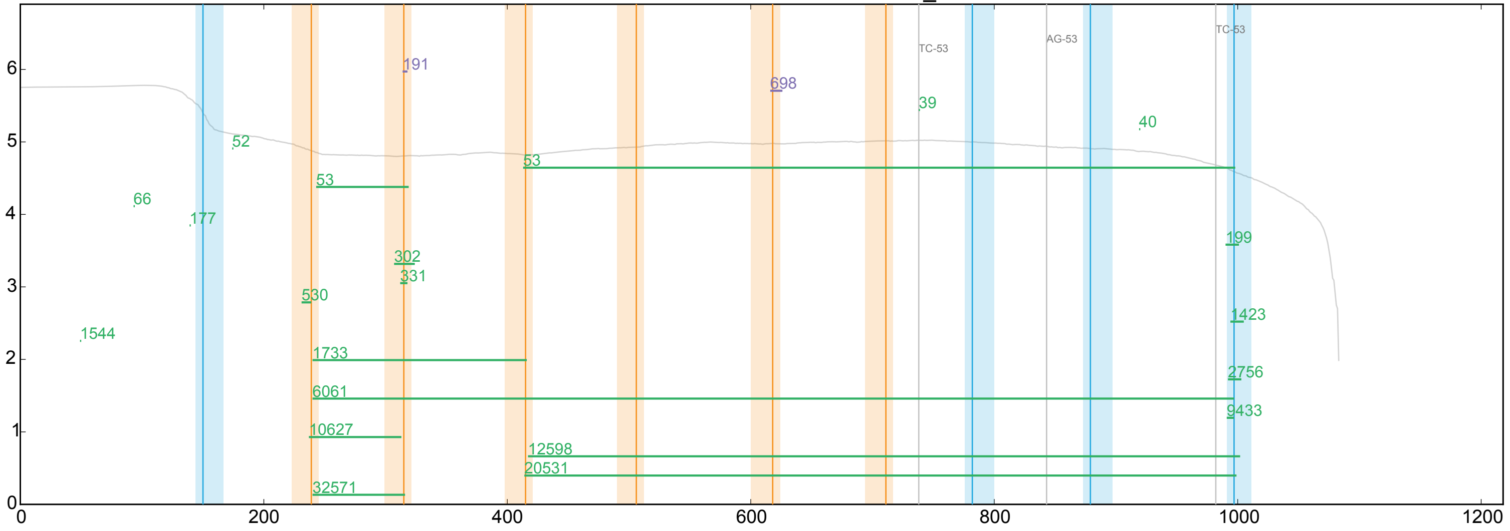
WT ENSDARG00000079348_0
