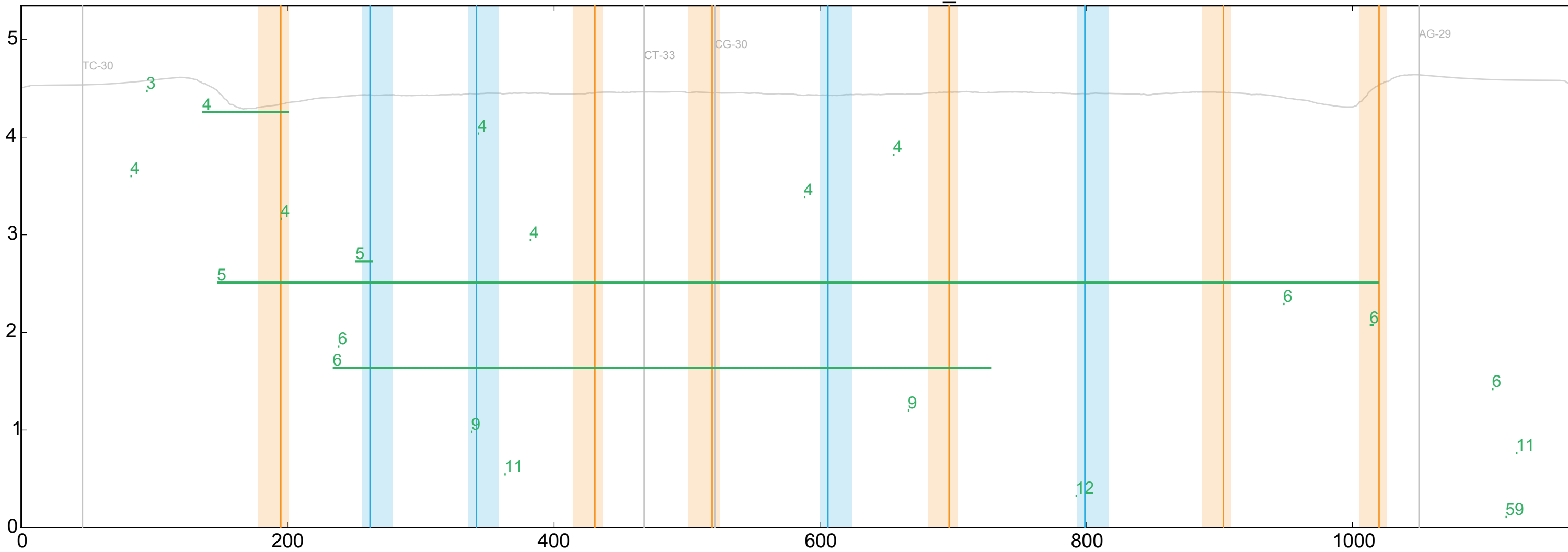
WT ENSDARG00000077842_7
