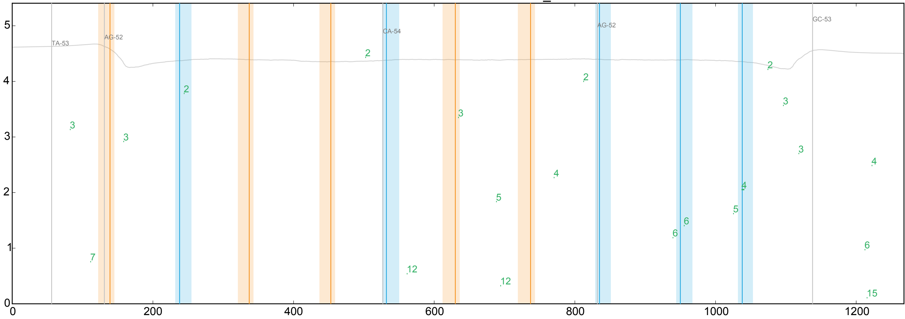
WT ENSDARG00000074184_0
