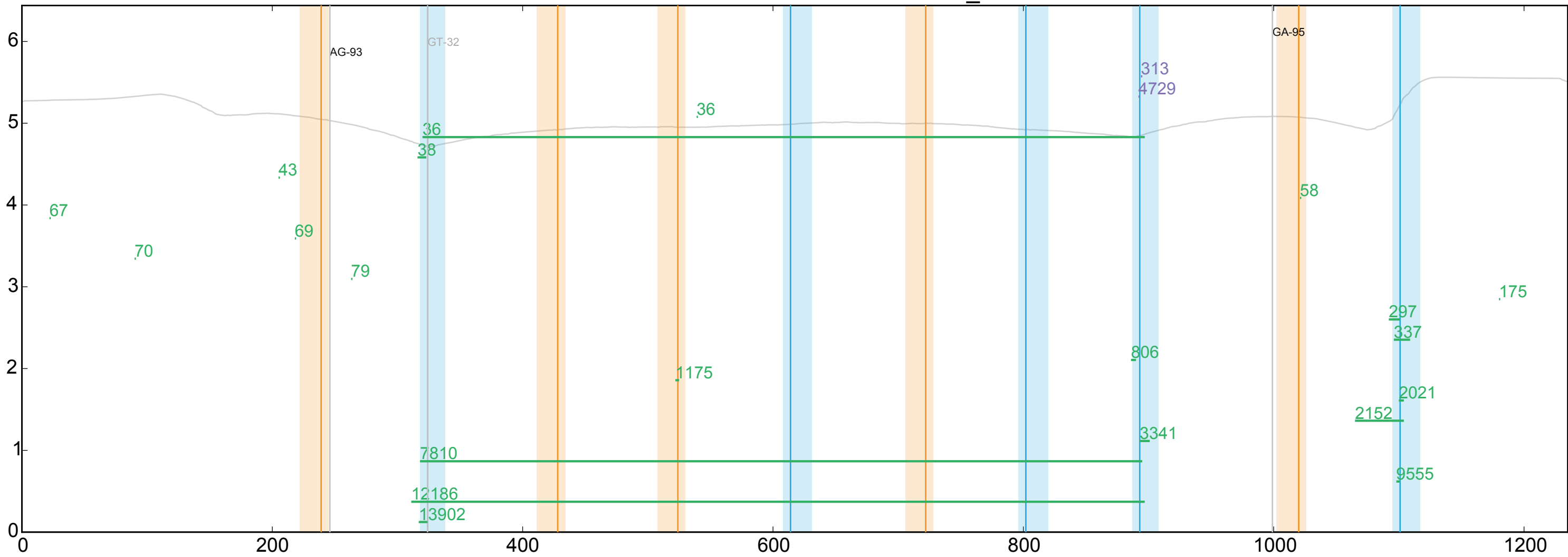
WT ENSDARG0000091127_1
