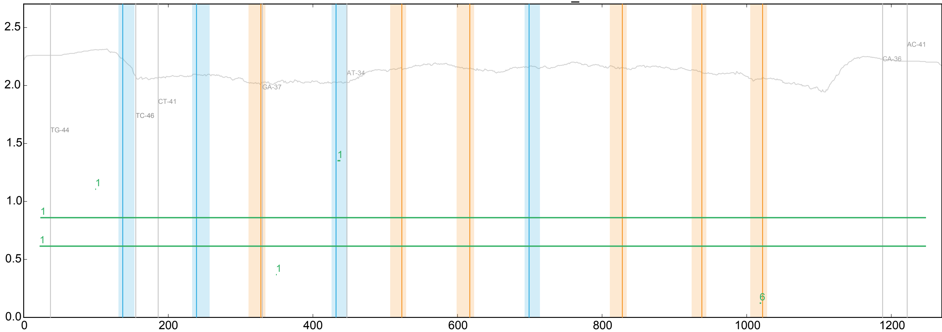
WT ENSDARG00000057582_0
