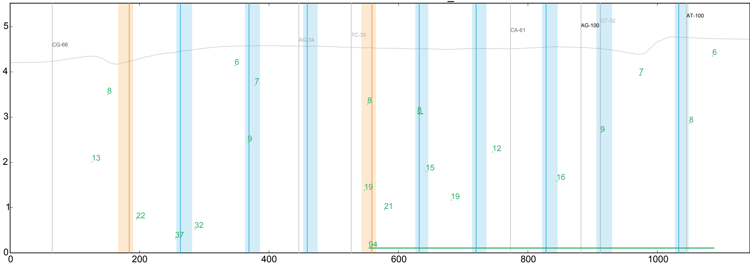
WT ENSDARG0000001244_13
