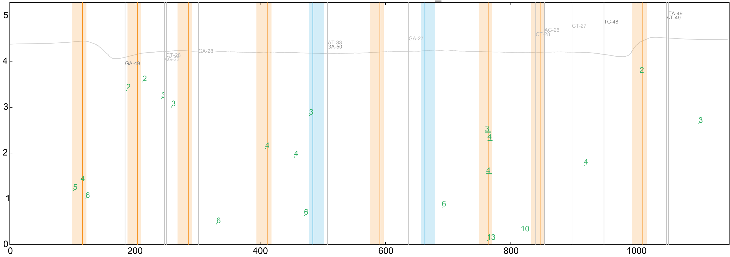
WT ENSDARG00000076485_12
