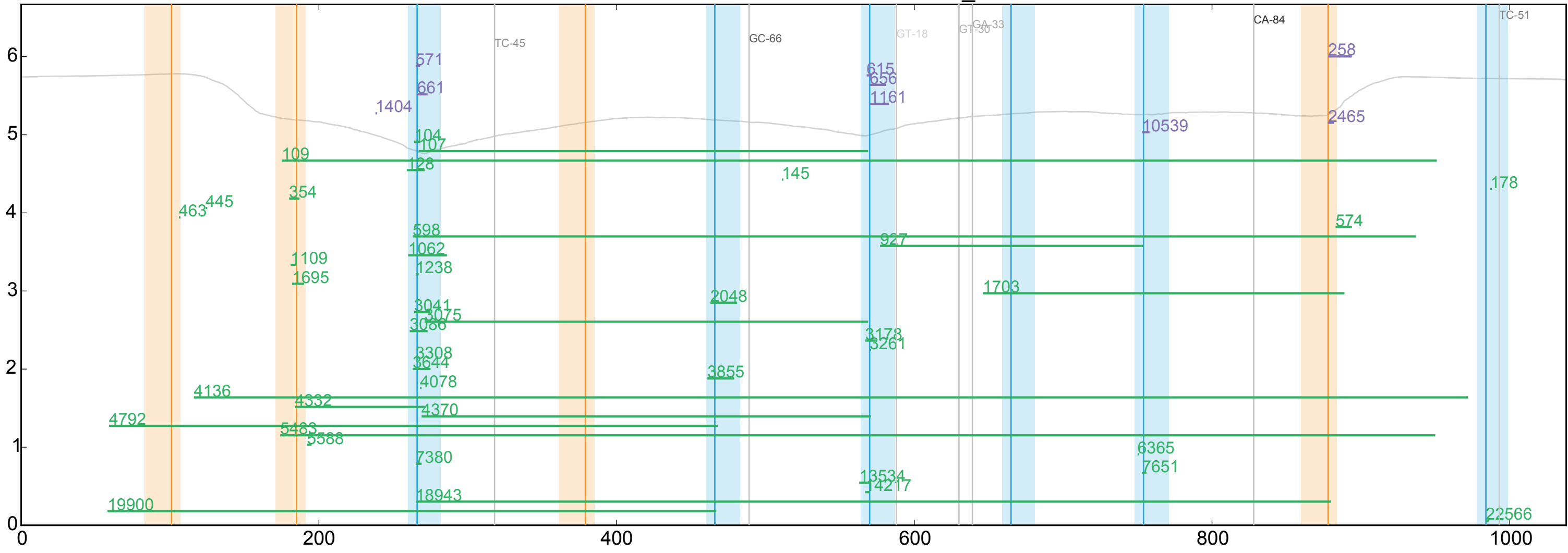
WT ENSDARG00000079850_0
