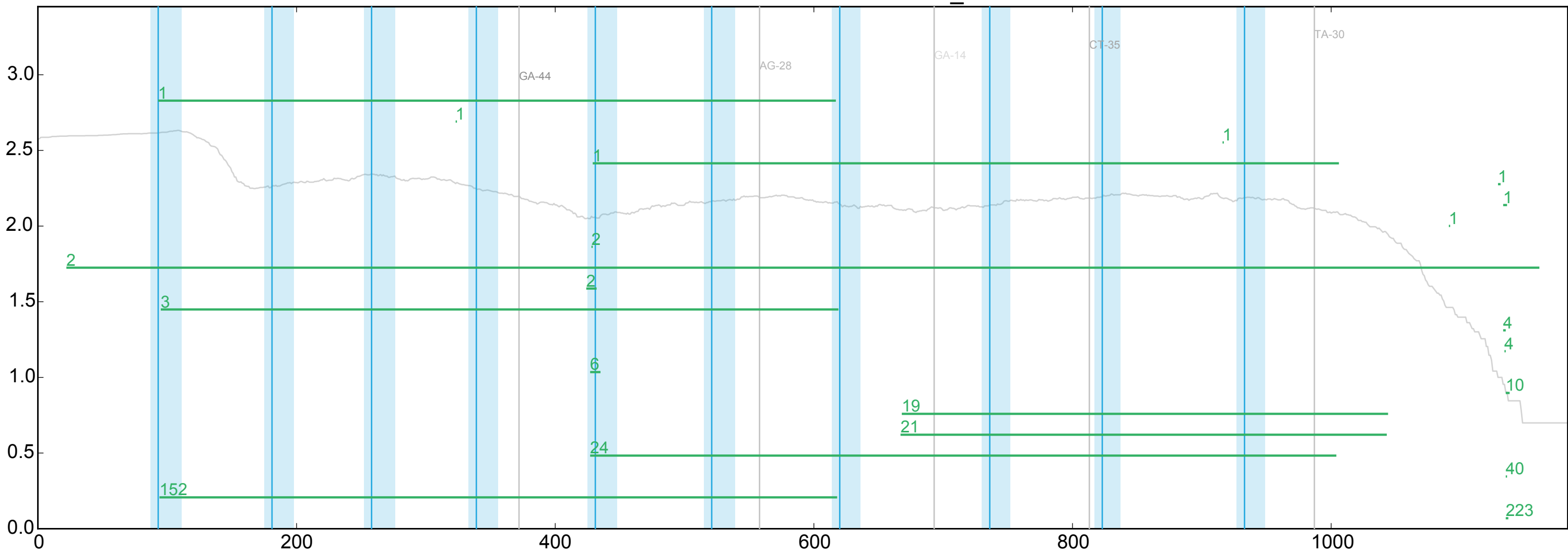
WT ENSDARG00000004473_5
