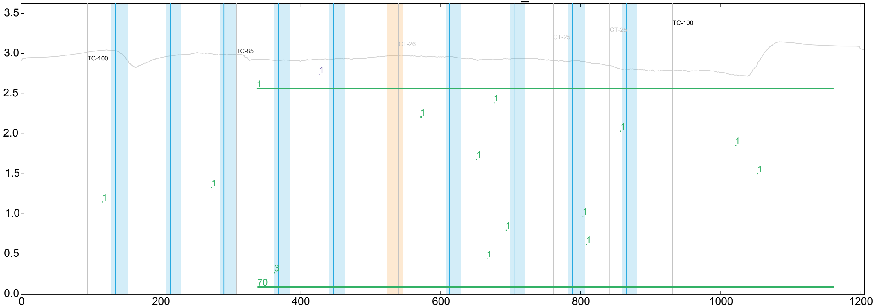
WT ENSDARG00000077353_15
