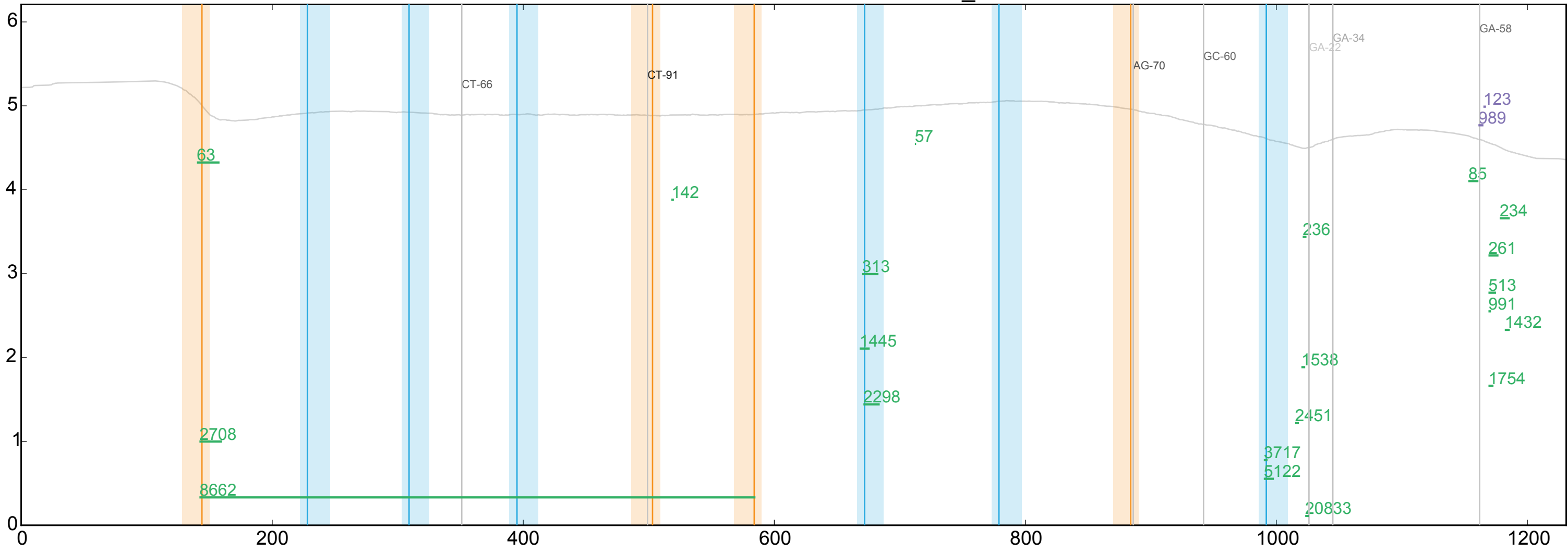
WT ENSDARG00000088347_3
