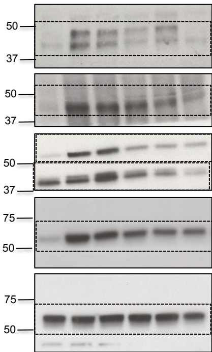
Fig. S4c (HFFF2)
