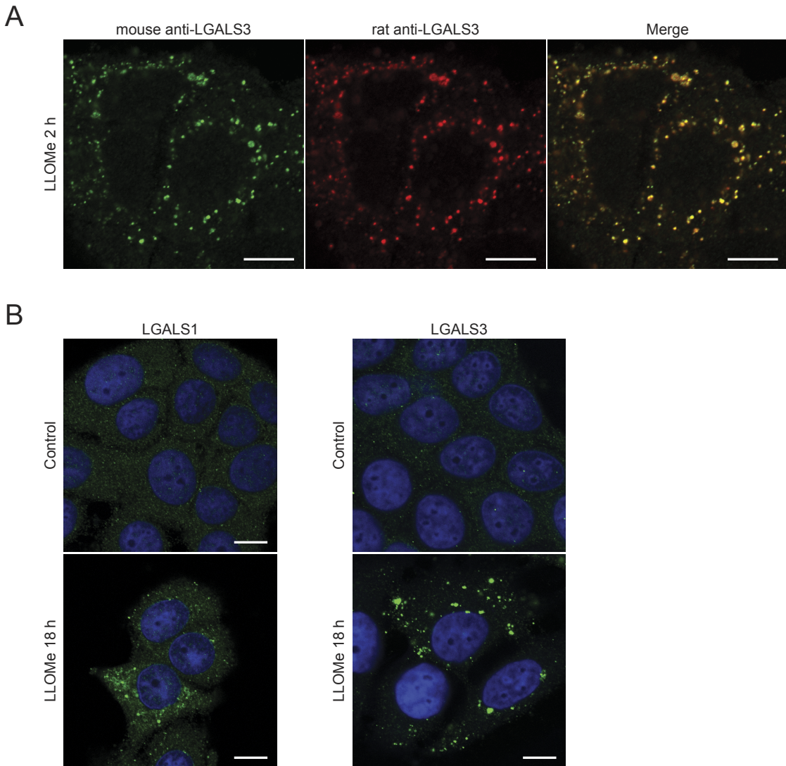
Figure S1. Comparison of LGALS3 antibodies and staining after methanol fixation. (A) MCF7 cells were treated with 2 mM LLOMe for 2 h and costained with mouse (green) and rat anti-LGALS3 (red) antibodies. Representative confocal microscopy images are shown. (B) MCF7 cells were treated with 2.5 mM LLOMe for 18 h, fixed in ice-cold methanol and stained with rabbit anti-LGALS1 or mouse anti-LGALS3 antibodies (green). Nuclei were labelled with Hoechst 33342 (blue). Representative confocal microscopy images are shown. Scale bars: 10 \mu m.
