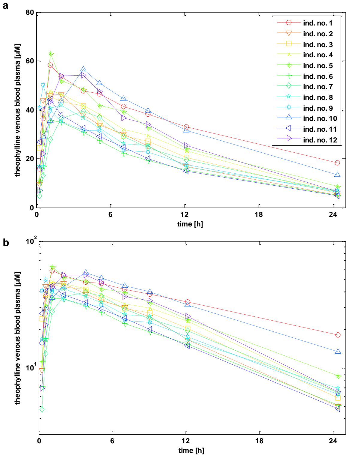
Figure S1: Experimental data of theophylline pharmacokinetics. The individual data is also provided in S2 Table. (a) Experimental data on linear scale. (b) Experimental data on semi-log scale.
