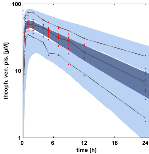
Figure S3: Visual predictive check (VPC) of the pharmacokinetic behavior using the posterior distributions of the positive control run based on the presented Bayesian population PBPK approach. The maximum posterior estimates of the population parameters have been used to estimate the posterior population distributions. The VPCs were performed as described in the text. In each VPC, the 5 % and 95 % percentiles (black dotted lines) and the median (black line) of the experimental data (red dots) are compared against the 95 % confidence intervals of the 5 % and 95 % percentile of the simulation (light blue area) and the median (blue area).
