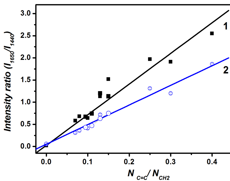
Additional file 4: illustration of intermixed standard fatty acids (oleic and palmitoleic acid) in the calibration curve with excitation of (1) 532 nm and (2) 785 nm.
