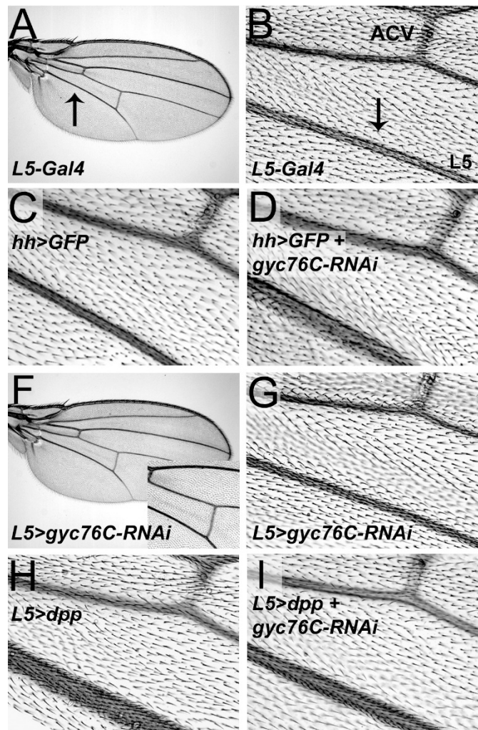
S7 Fig. Effects of Gyc76C on adult vein width.
