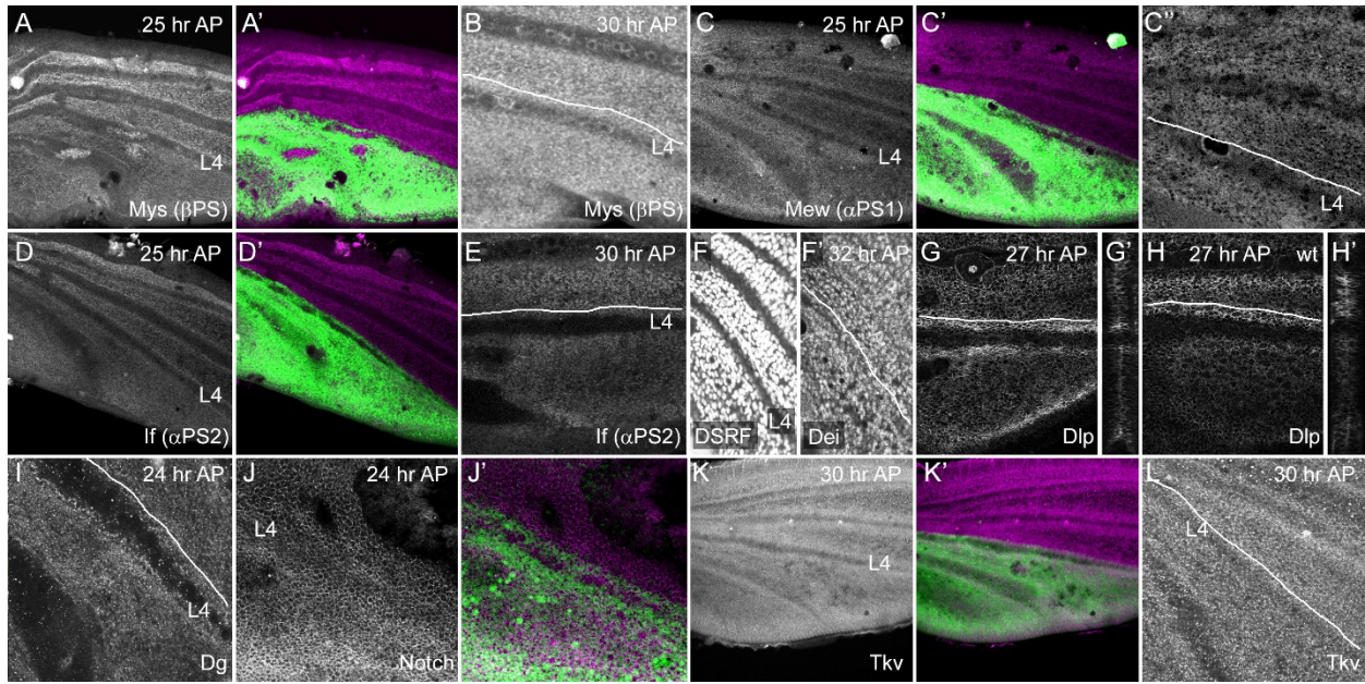
S10 Fig. Candidate proteins unaffected by posterior knockdown of gyc76C .
