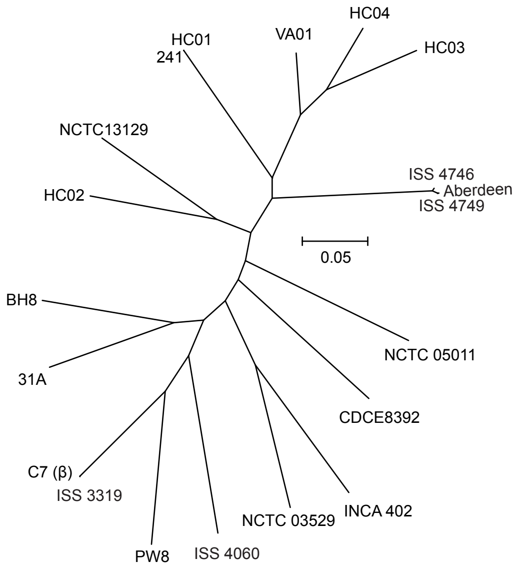
Supplementary Fig. 1. A phylogenetic tree from 400 conserved protein sequences using PhyloPhlAn.
