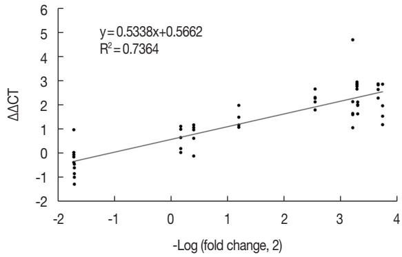
Supplementary Figure 1. Correlation of relative expression value quantified by qPCR with that analyzed by RNA sequencing. Y-axis, representing the circRNA abundance differentiation between rat mammary glands at day 1 and day 7 as measured by qPCR; X-axis, representing the circRNA abundance differentiation between rat mammary glands at day 1 and day 7 as measured by RNA-sequencing.
