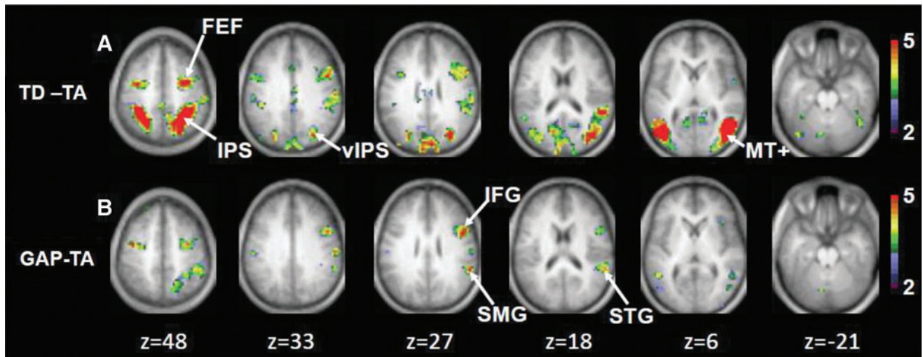
SUPPLEMENTARY FIG. 1. Voxelwise statistical maps showing that significant differences between tasks were observed in regions involved in attention and eye movements. Selected brain slices representing z values from voxelwise analyses of variance for the main effect of Task that compared (A) Tracking with Distracters vs. Tracking Alone and (B) Tracking with Gaps vs. Tracking Alone. Color scale represents z -statistic.
