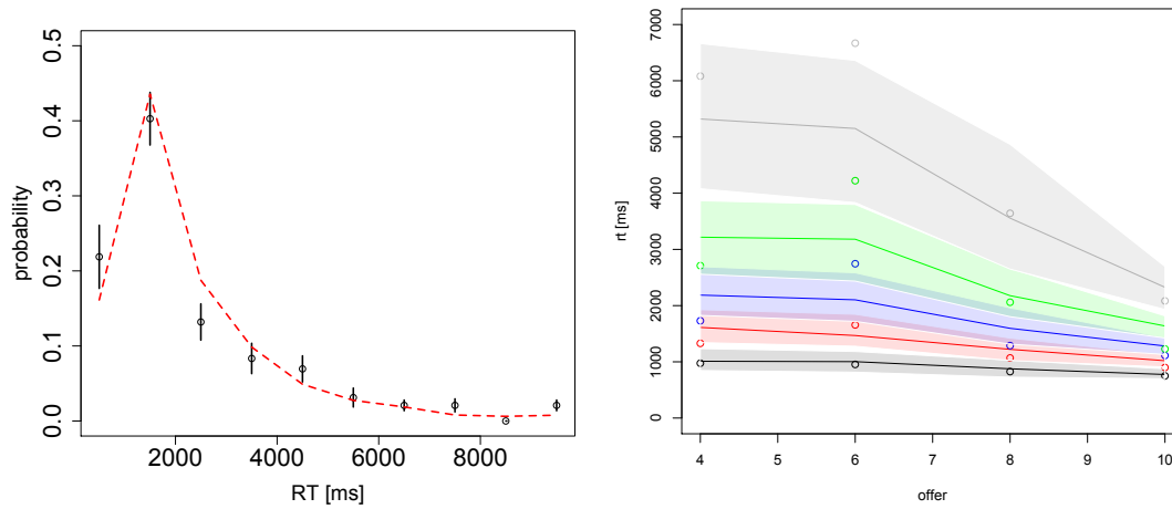
Figure S1: Reaction-time histograms and quantile-utility plots for Tasks 1-4 respectively, pooling all of the data from each task. In the histograms, black circles indicate the subject means with standard error bars clustered by subject. Red dashed lines indicate the aDDM predictions. In the quantile-utility plots, circles indicate the aggregate subject data and lines indicate the DDM predictions ( \theta = 0.3 ) with lighter shading showing 95% confidence intervals from the simulations. Black, red, blue, green and gray colors indicate the 10%, 30%, 50%, 70% and 90% quantiles for reaction times.
