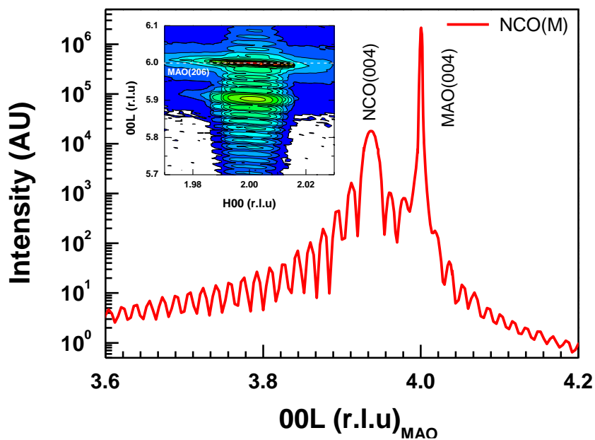
Figure S1. Room temperature x-ray diffractogram of metallic \text{NiCo}_2\text{O}_4 film grown on \text{MgAl}_2\text{O}_4(100) substrate. Corresponding Reciprocal Space Map around the (206) reflection is shown in the inset.
