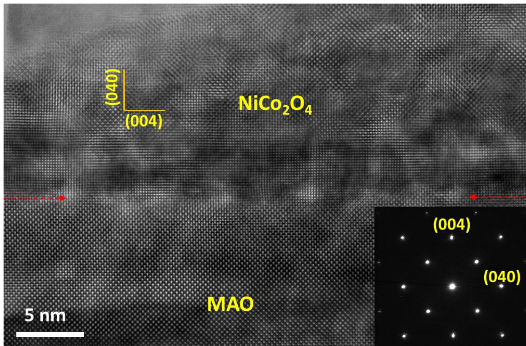
Figure S2. Cross-sectional HRTEM image for the NiCo 2 O 4 (NCO(M)) films grown on MgAl 2 O 4 substrate. The corresponding selected area diffraction patterns of the NCO films and MAO substrate along the [100] zone axis.
