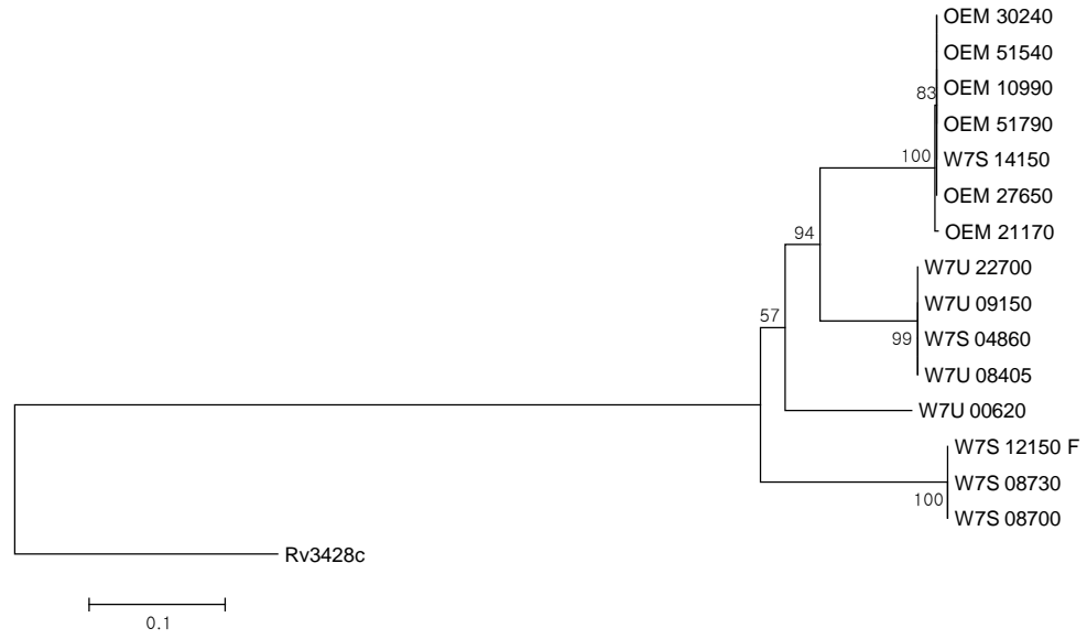
(A) istA -like sequence
