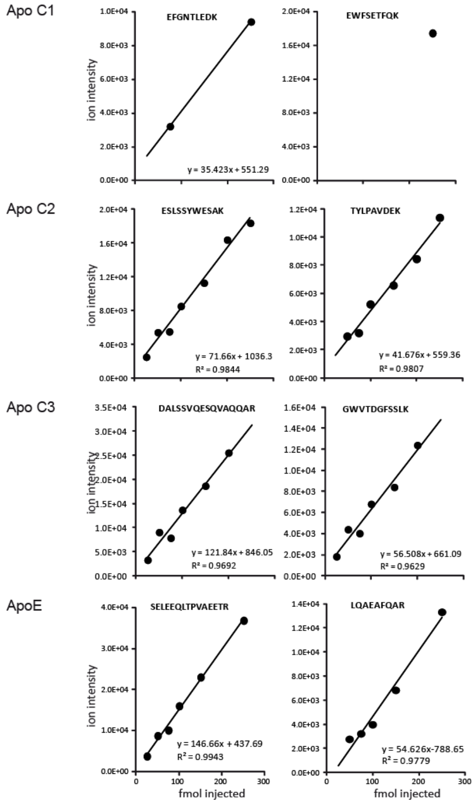
S3 Fig b. Linearity of detection of individual peptides derived from QconCAT in a plasma background. Increasing amounts of QconCAT added to a pooled plasma sample prior to digestion. Ion intensities of identified peptides are plotted against the amount (fmols) added. Formula and r^2 obtained are depicted
