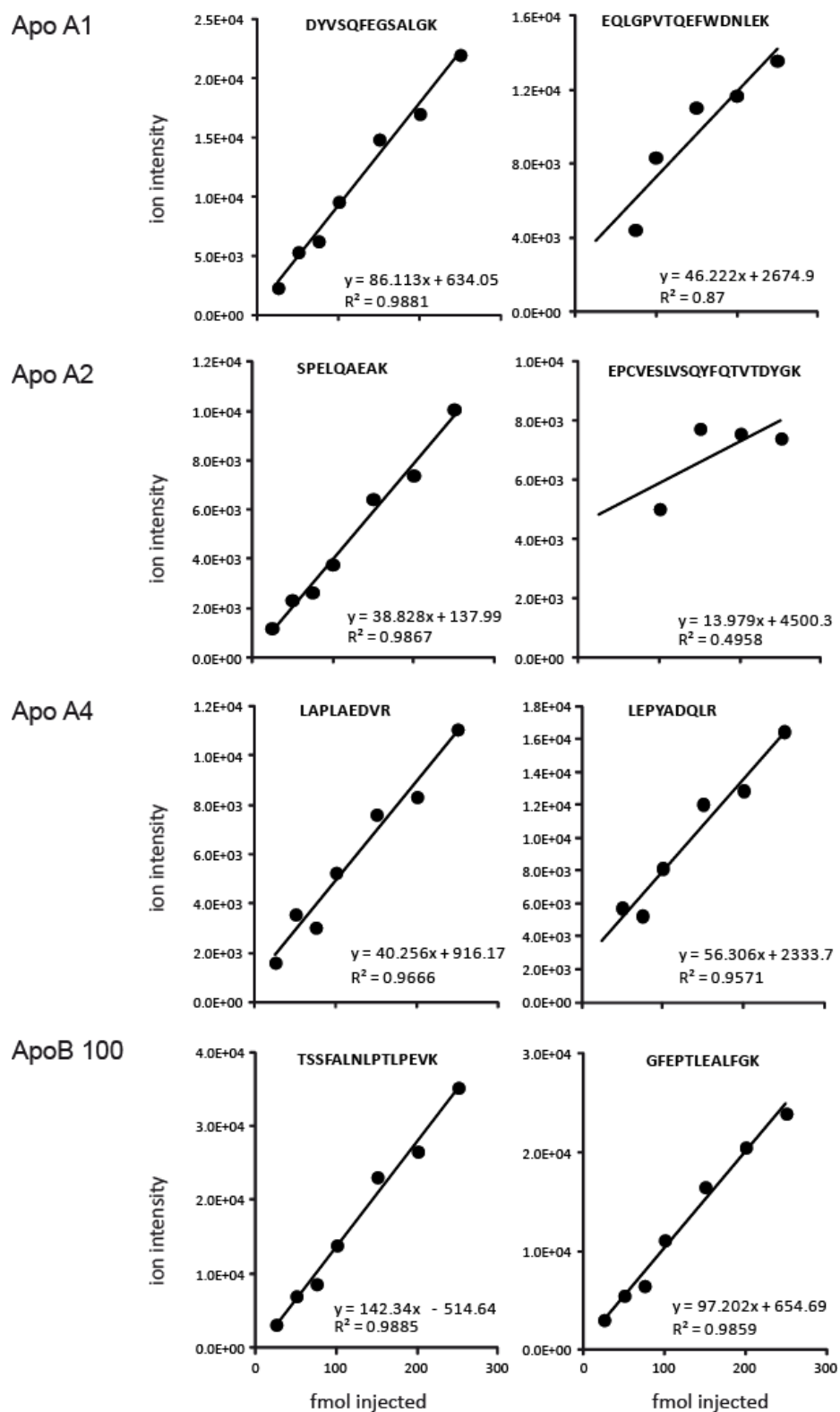
S3 Fig a. Linearity of detection of individual peptides derived from QconCAT in a plasma background. Increasing amounts of QconCAT added to a pooled plasma sample prior to digestion. Ion intensities of identified peptides are plotted against the amount (fmols) added. Formula and r 2 obtained are depicted
