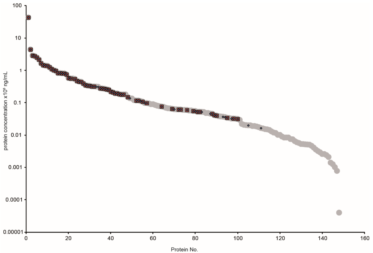
S4 Fig. Reference concentrations of proteins identified by LCMS E . Average concentration from Hortin et al. is shown (grey dots), proteins identified by LCMS analysis are shown by blue diamonds, proteins for which a quantitative value was also determined by HI3 peptide quantitation are indicated by red squares.
