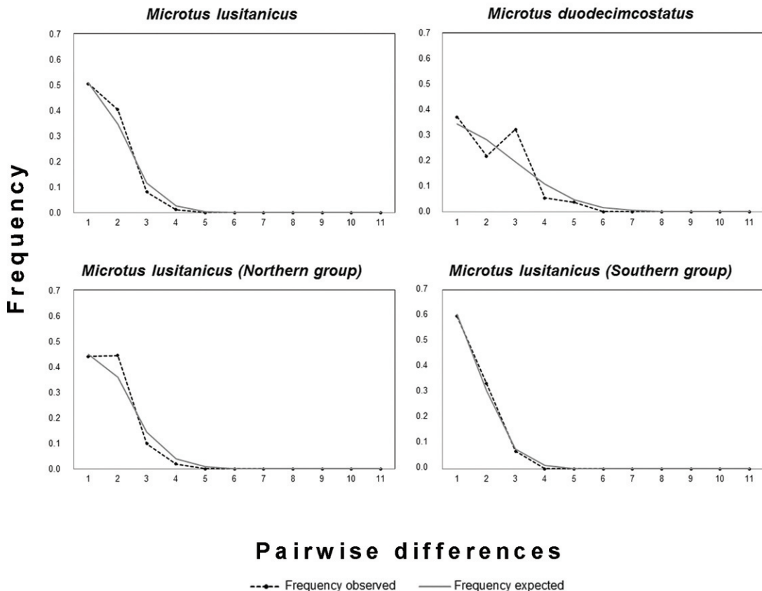
Supplementary Figure S1 Frequency distributions of the number of pairwise nucleotide differences (mismatch distributions) between p53 haplotypes of M. lusitanicus , M. duodecimcostatus and regional groups of M. lusitanicus , according to the sudden-expansion model.
