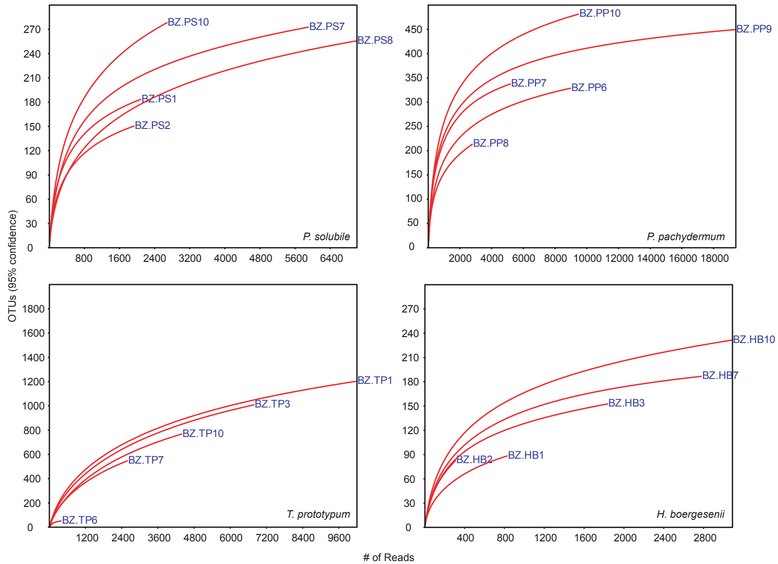
SI Figure 1. Rarefaction curves of CCA biofilm samples showing each of the five samples per CCA species.
