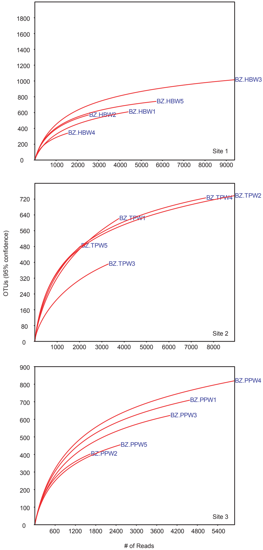
SI Figure 2. Rarefaction curves of seawater samples showing each of the five samples per site.
