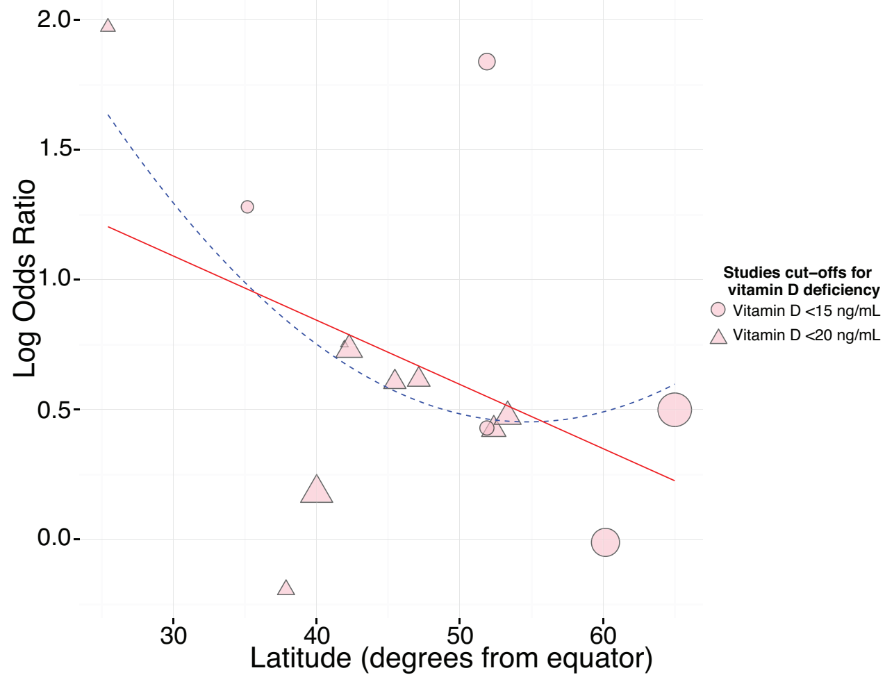
Supplementary Figure 1: Meta-regression analysis on the association between IBD and serum vitamin D levels using latitude as a moderator. Red solid line represents the linear model, whereas blue dashed line represents the polynomial fractional best fitting model. No interaction was found between serum vitamin D levels and latitude.
