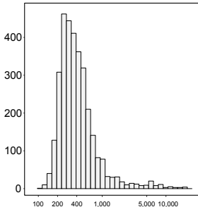
cerebellum circRNA
