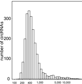
blood circRNA
