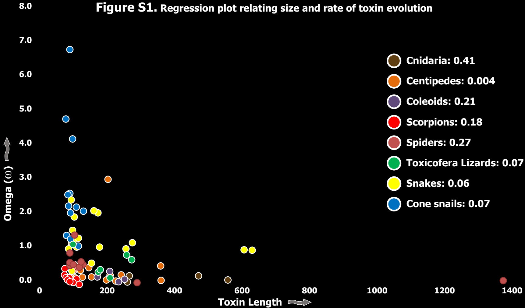
Figure S1: Regression analyses of various toxin types in each of the examined venomous lineage is presented here. Omega values are plotted against the size/length of the respective toxin type. The coefficient of determination ( r^2 ) for each clade has also presented. r^2 values closer to 0 suggest an absence of correlation between the size of the toxin and its omega (rate of evolution) value.
