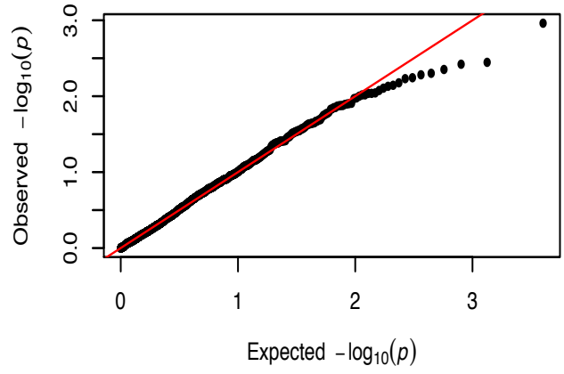
most correlated
