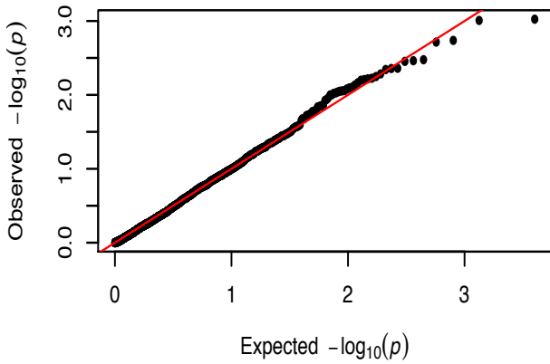
RF
