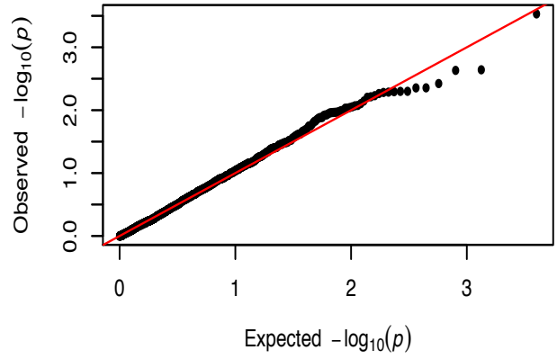
most correlated
