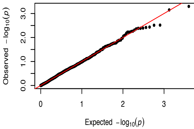
RF
