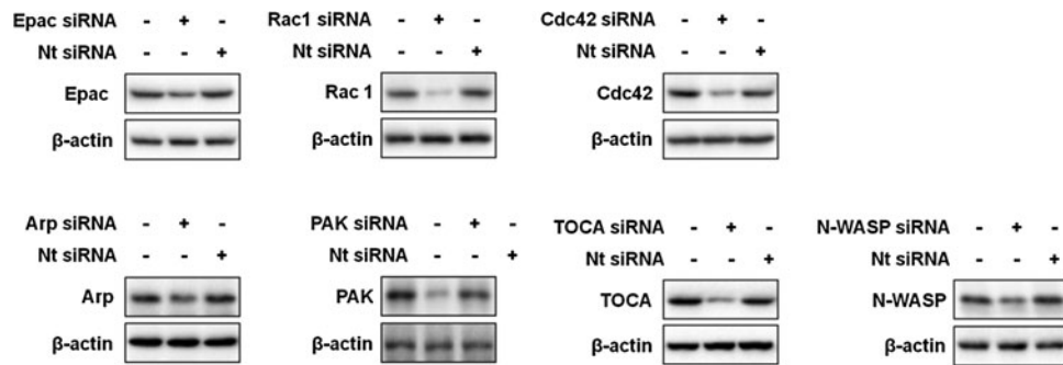
SUPPLEMENTARY FIG. S1. Small interfering RNA (siRNA) efficacy used in the present study. Mouse embryonic stem cells were transfected with Epac, Rac1, CDC42, Arp, PAK, TOCA, and N-WASP siRNA for 6 h and then the culture media were replaced with transfection mixture-free and serum-free media. The cells were harvested at 24 h from initial transfection time. Each target protein of siRNA was detected with western blot analysis, respectively.
