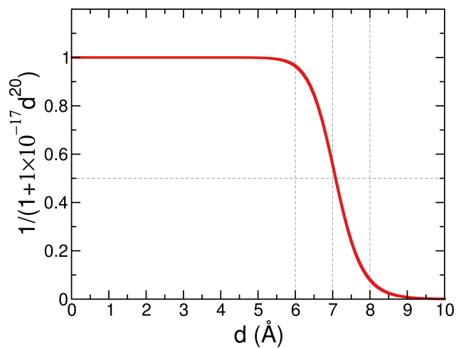
Figure S2: Switching function between 6 Å and 8 Å used for the probe occupancy calculation based on equation 1 in the main text.
