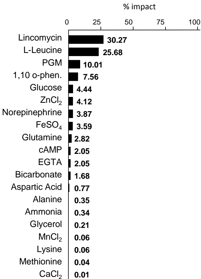
Figure S1. Component effect on the variability of the CFA/I response. Pareto distribution diagram showing the percent impact of each component on CFA/I surface expression.
