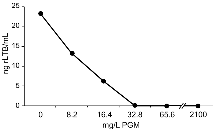
Figure S2. Concentration dependent LTB epitope masking by PGM. 20 ng/mL recombinant LTB (rLTB) was incubated in SP1 culture media containing 0 to 2100 mg/L PGM for 1 hour before LTB quantification by GM1 ELISA.
