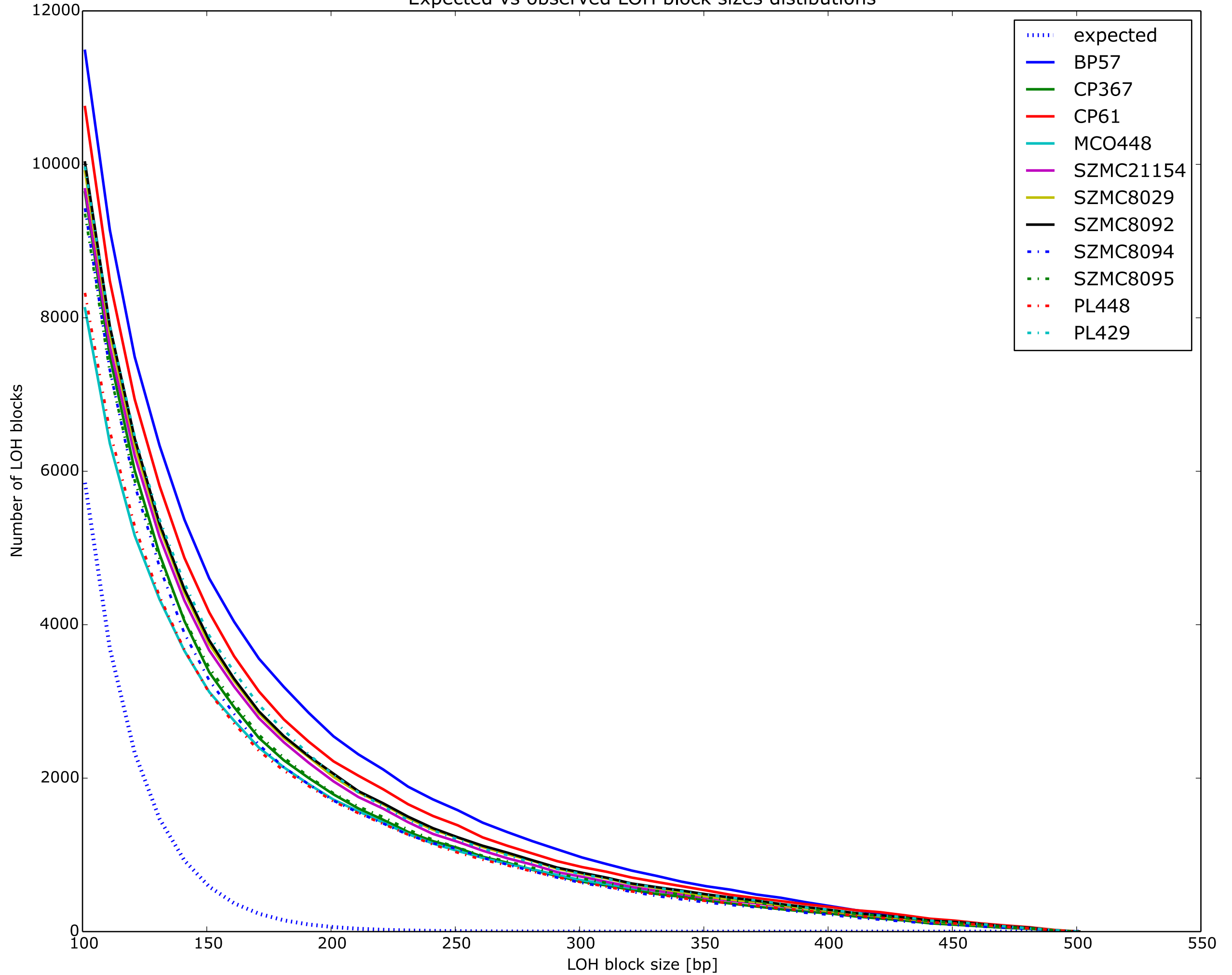
Expected vs observed LOH block sizes distributions
