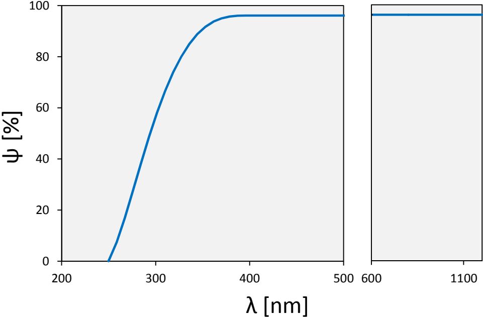
Suppl. 1 Spectral transmittance ( \Psi ) of Plexiglas® XT Clear 29070 (thickness: 3 mm) in the ultraviolet and visible range (after data from Röhm, Darmstadt, Germany)
